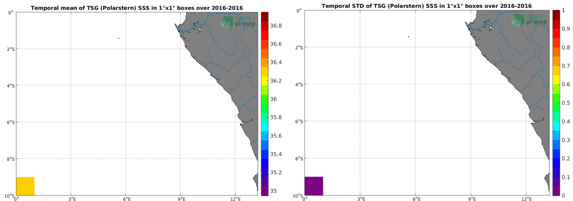
(c) MEAN(TSG (Polarstern) SSS)
