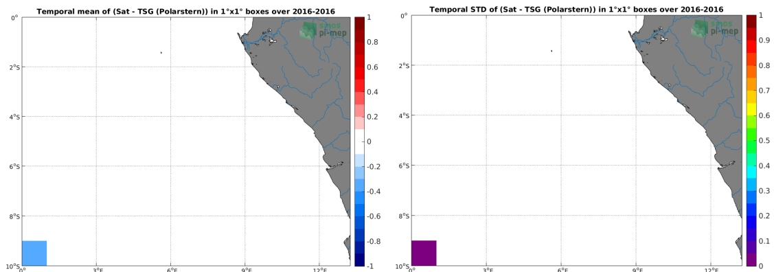
(e) MEAN( \Delta SSS) (Satellite - TSG (Polarstern))
