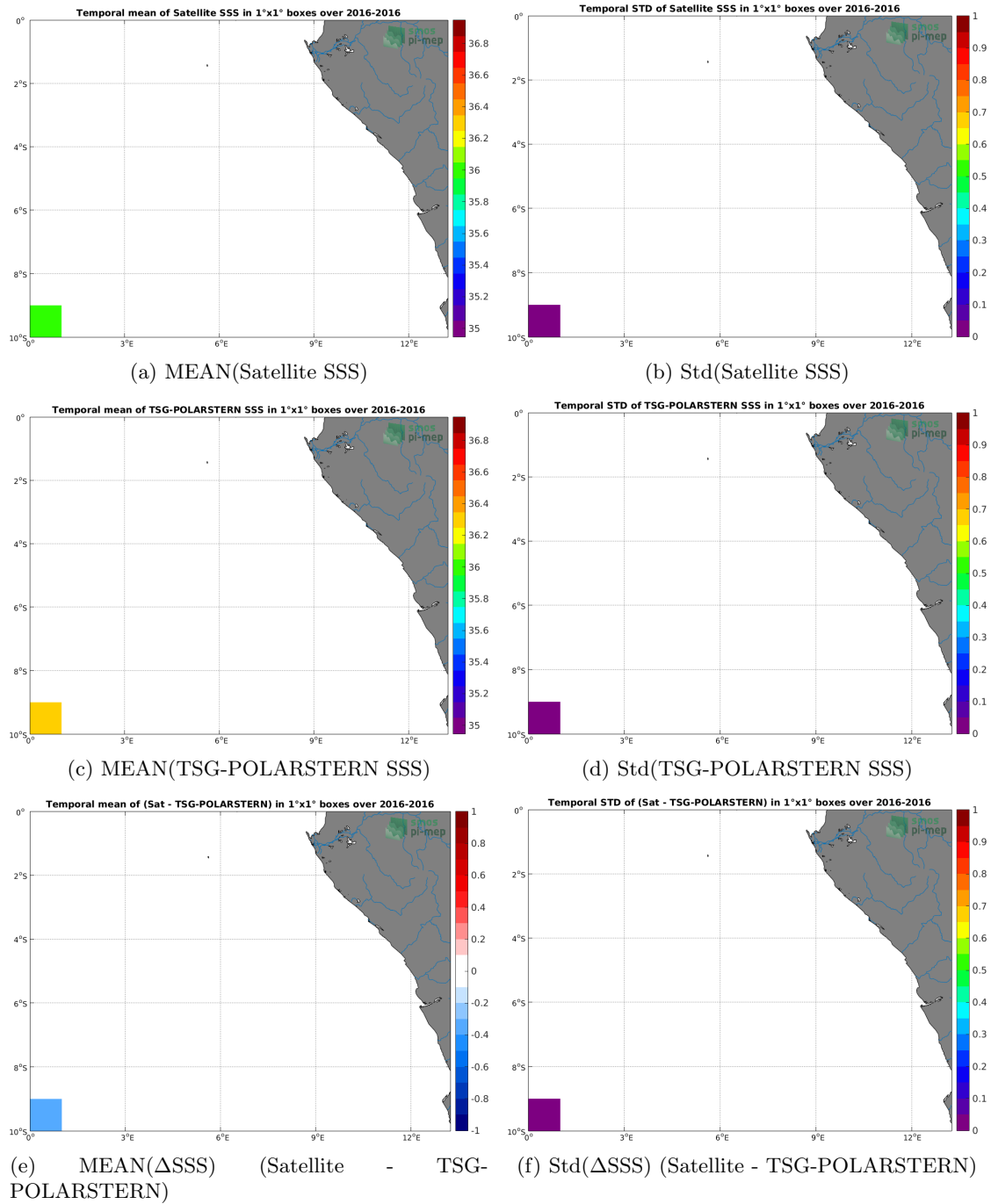
Figure 6: Temporal mean (left) and Std (right) of SSS from SMOS L3 v2 - Monthly - 0.25 Deg (CATDS-CECOS-IFREMER) (top), TSG-POLARSTERN (middle), and of \Delta SSS (Satellite - TSG-POLARSTERN). Only match-up pairs are used to generate these maps.
