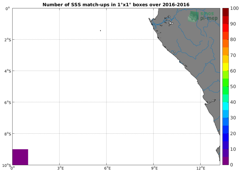
Figure 4: Number of SSS match-ups between TSG-POLARSTERN SSS and the SMOS L3 v2 - Monthly - 0.25 Deg (CATDS-CECOS-IFREMER) SSS product for the Congo river plume Pi-MEP region over 1^\circ \times 1^\circ boxes and for the full satellite product period.
