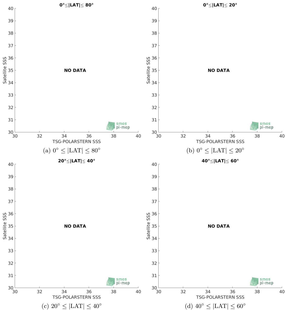
Figure 9: Contour maps of the concentration of SMOS L3 v2 - Monthly - 0.25 Deg (CATDS-CECOS-IFREMER) SSS (y-axis) versus TSG-POLARSTERN SSS (x-axis) at match-up pairs for different latitude bands. For each plot, the red line shows x=y . The black thin and dashed lines indicate a linear fit through the data cloud and the \pm 95\% confidence levels, respectively. The number match-up pairs n , the slope and R^2 coefficient of the linear fit, the root mean square (RMS) and the mean bias between satellite and in situ data are indicated for each latitude band in each plots.
