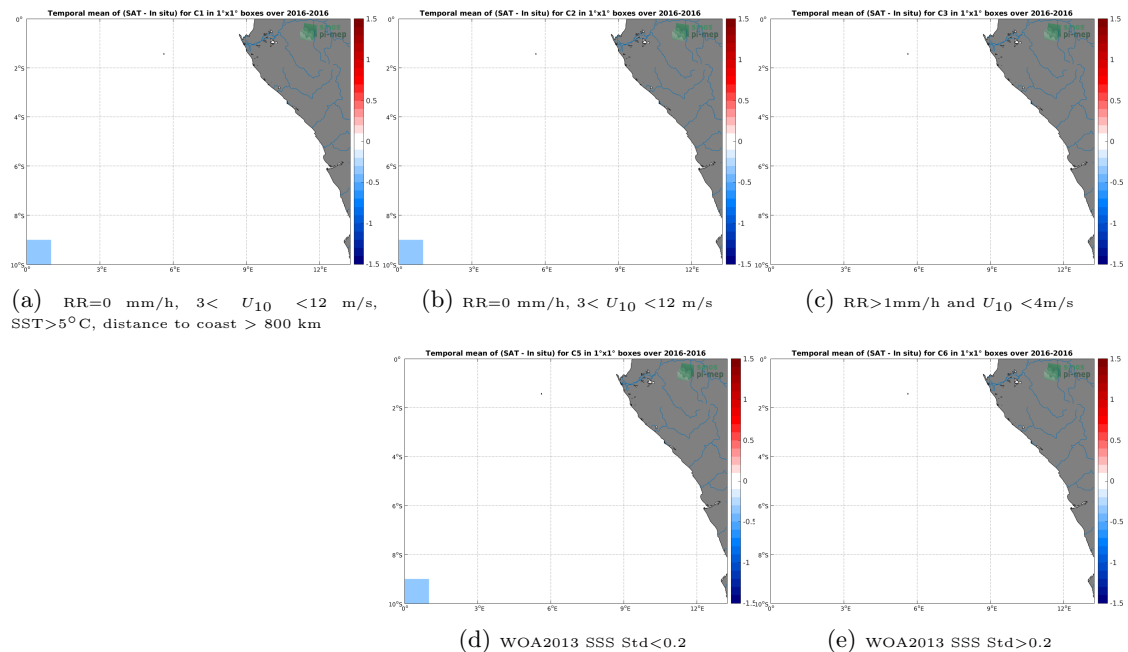
Figure 12: Temporal mean gridded over spatial boxes of size 1^{\circ}\times 1^{\circ} of \Delta\text{SSS} (SMOS L3 v2 - Monthly - 0.25 Deg (CATDS-CECOS-IFREMER) - TSG-POLARSTERN) for 5 different sub-datasets corresponding to:RR=0 mm/h, 3 < U_{10} < 12 m/s, SST >5^{\circ}\text{C} , distance to coast > 800 km (a), RR=0 mm/h, 3 < U_{10} < 12 m/s (b), RR >1 mm/h and U_{10} < 4 m/s (c), WOA2013 SSS Std <0.2 (d), WOA2013 SSS Std >0.2 (e).
