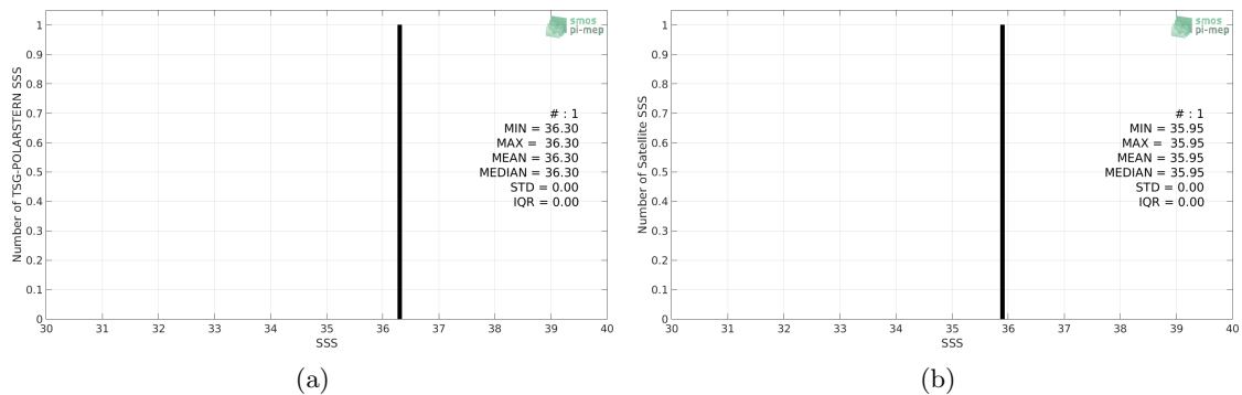
Figure 2: Histograms of SSS from TSG-POLARSTERN (a) and SMOS L3 v2 - Monthly - 0.25 Deg (CATDS-CECOS-IFREMER) (b) considering all match-up pairs per bins of 0.1 over the Congo river plume Pi-MEP region and for the full satellite product period.
