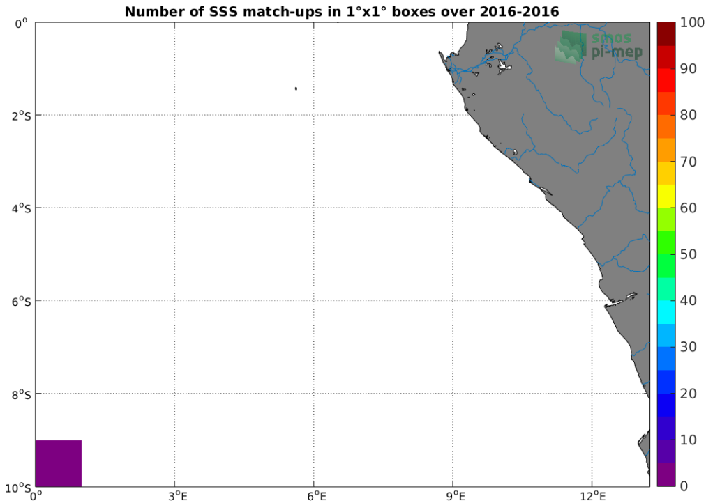
Figure 4: Number of SSS match-ups between TSG-POLARSTERN SSS and the SMOS-L3-CATDS-IFREMER-CECOS-V2-MONTHLY-0.25DEG SSS product for the Congo river plume Pi-MEP region over 1^\circ \times 1^\circ boxes and for the full satellite product period.
