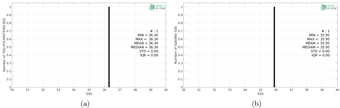
Figure 2: Histograms of SSS from TSG-POLARSTERN (a) and SMOS-L3-CATDS-IFREMER-CECOS-V2-MONTHLY-0.25DEG (b) considering all match-up pairs per bins of 0.1 over the Congo river plume Pi-MEP region and for the full satellite product period.
