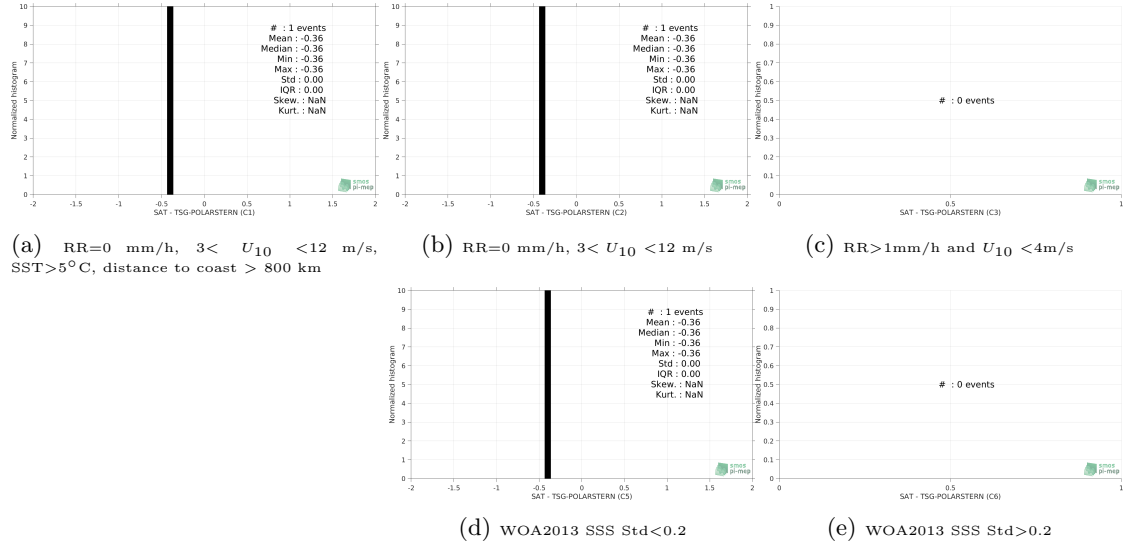
Figure 13: Normalized histogram of \Delta SSS (SMOS-L3-CATDS-IFREMER-CECOS-V2-MONTHLY-0.25DEG - TSG-POLARSTERN) for 5 different subdatasets corresponding to: RR=0 mm/h, 3 < U_{10} < 12 m/s, SST>5°C, distance to coast > 800 km (a), RR=0 mm/h, 3 < U_{10} < 12 m/s (b), RR>1mm/h and U_{10} < 4 m/s (c), WOA2013 SSS Std<0.2 (d), WOA2013 SSS Std>0.2 (e).
