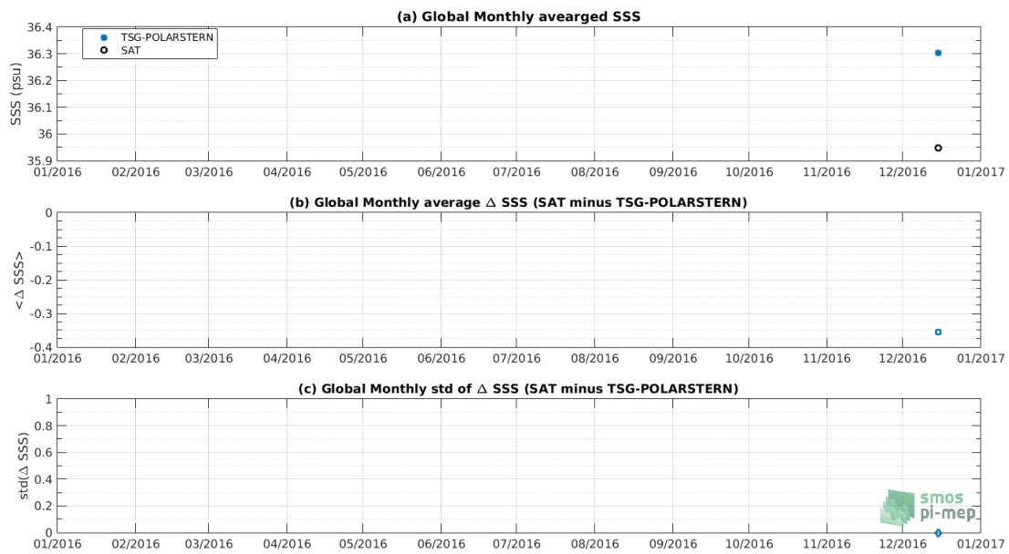
Figure 7: Time series of the monthly averaged mean SSS (top), mean \Delta SSS (Satellite - TSG-POLARSTERN) and Std of \Delta SSS (Satellite - TSG-POLARSTERN) over the Congo river plume Pi-MEP region considering all match-ups collected by the Pi-MEP platform.
