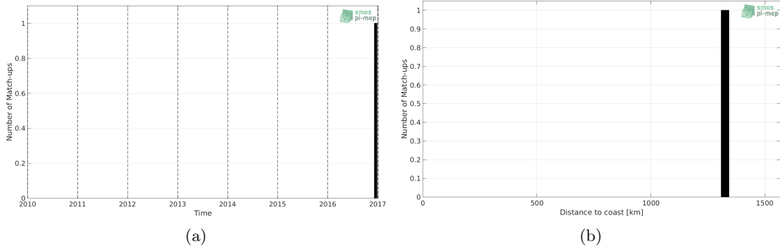
Figure 1: Number of match-ups between TSG-POLARSTERN and SMOS-L3-CATDS-IFREMER-CECOS-V2-MONTHLY-0.25DEG SSS as a function of time (a) and as function of the distance to coast (b) over the Congo river plume Pi-MEP region and for the full satellite product period.
