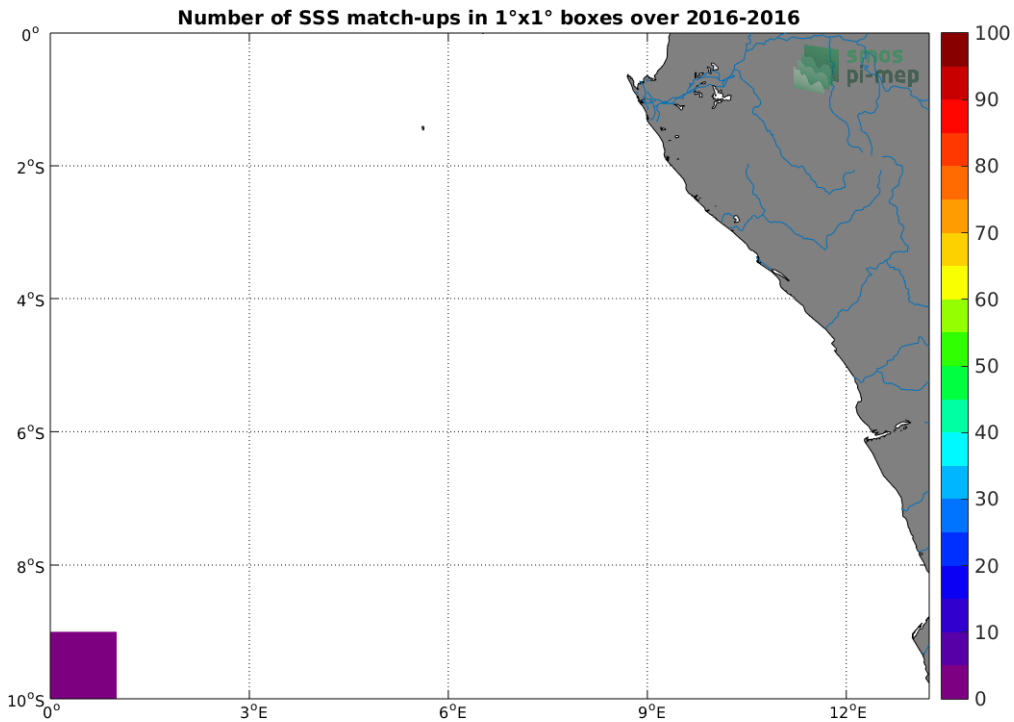
Figure 4: Number of SSS match-ups between TSG-POLARSTERN SSS and the SMOS-L3-CATDS-IFREMER-CECOS-V2-MONTHLY-0.25DEG SSS product for the Congo river plume Pi-MEP region over 1^{\circ} \times 1^{\circ} boxes and for the full satellite product period.
