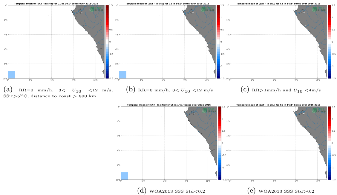
Figure 12: Temporal mean gridded over spatial boxes of size 1^\circ \times 1^\circ of \Delta SSS (SMOS-L3-CATDS-IFREMER-CECOS-V2-MONTHLY-0.25DEG - TSG-POLARSTERN) for 5 different subdatasets corresponding to: RR=0 mm/h, 3 < U_{10} < 12 m/s, SST > 5^\circ C , distance to coast > 800 km (a), RR=0 mm/h, 3 < U_{10} < 12 m/s (b), RR > 1 mm/h and U_{10} < 4 m/s (c), WOA2013 SSS Std < 0.2 (d), WOA2013 SSS Std > 0.2 (e).
