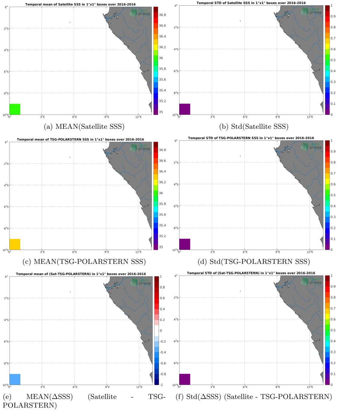
Figure 6: Temporal mean (left) and Std (right) of SSS from SMOS-L3-CATDS-IFREMER-CECOS-V2-MONTHLY-0.25DEG (top), TSG-POLARSTERN (middle), and of \Delta SSS (Satellite - TSG-POLARSTERN). Only match-up pairs are used to generate these maps.
