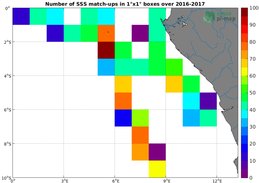
Figure 4: Number of SSS match-ups between TSG (LEGOS-DM) SSS and the SMOS SSS L3 v2 - Monthly - 0.25 Deg (CATDS-CECOS-IFREMER) SSS product for the Congo river plume Pi-MEP region over 1°x1° boxes and for the full satellite product period.
