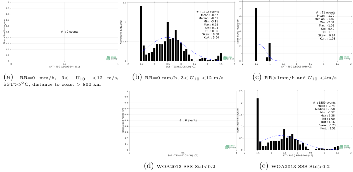
Figure 13: Normalized histogram of \Delta\text{SSS} (SMOS SSS L3 v2 - Monthly - 0.25 Deg (CATDS-CECOS-IFREMER) - TSG (LEGOS-DM)) for 5 different subdatasets corresponding to: RR=0 mm/h, 3 < U_{10} < 12 m/s, SST > 5^\circ\text{C} , distance to coast > 800 km (a), RR=0 mm/h, 3 < U_{10} < 12 m/s (b), RR > 1\text{mm/h} and U_{10} < 4\text{m/s} (c), WOA2013 SSS Std < 0.2 (d), WOA2013 SSS Std > 0.2 (e).
