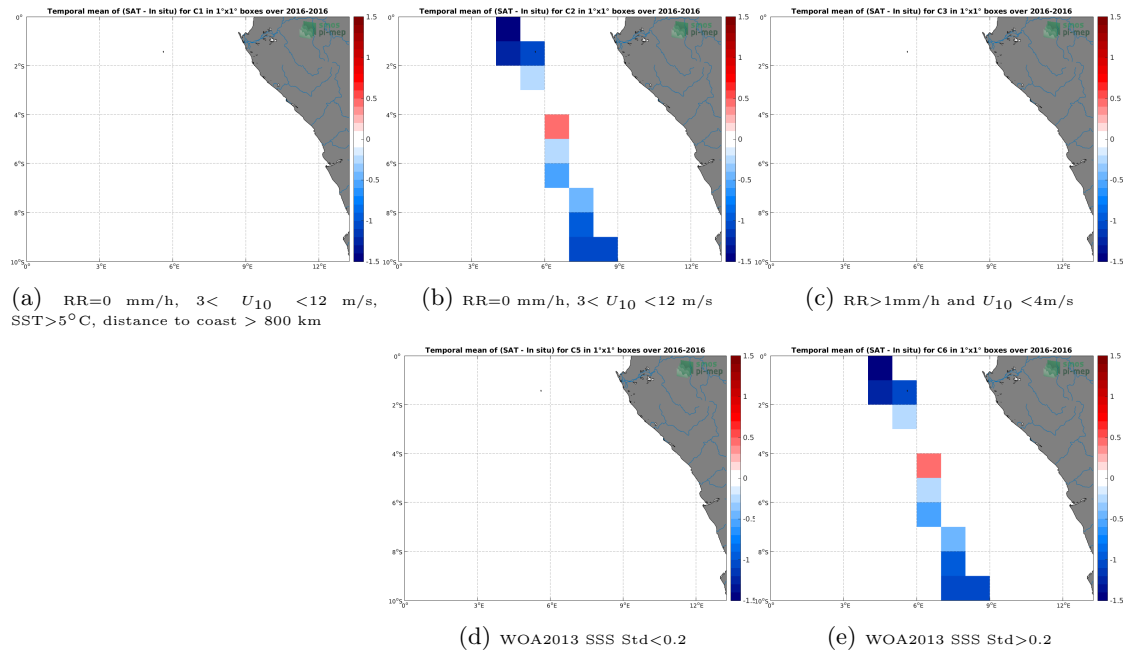
Figure 12: Temporal mean gridded over spatial boxes of size 1^{\circ}\times 1^{\circ} of \Delta\text{SSS} (SMOS L3 v2 - Monthly - 0.25 Deg (CATDS-CECOS-IFREMER) - TSG-LEGOS-DM) for 5 different subdatasets corresponding to:RR=0 mm/h, 3 < U_{10} < 12 m/s, SST >5^{\circ}\text{C} , distance to coast > 800 km (a), RR=0 mm/h, 3 < U_{10} < 12 m/s (b), RR >1 mm/h and U_{10} < 4 m/s (c), WOA2013 SSS Std <0.2 (d), WOA2013 SSS Std >0.2 (e).
