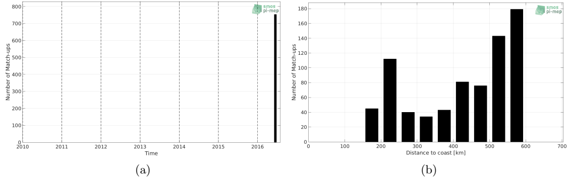
Figure 1: Number of match-ups between TSG-LEGOS-DM and SMOS L3 v2 - Monthly - 0.25 Deg (CATDS-CECOS-IFREMER) SSS as a function of time (a) and as function of the distance to coast (b) over the Congo river plume Pi-MEP region and for the full satellite product period.
