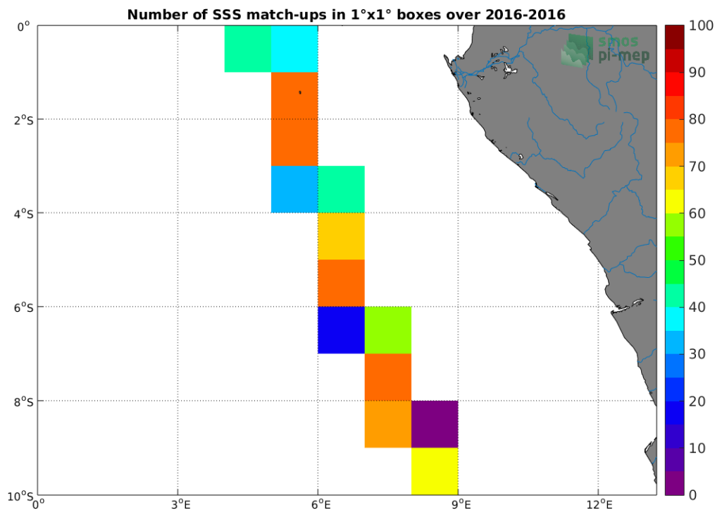
Figure 4: Number of SSS match-ups between TSG-LEGOS-DM SSS and the SMOS L3 v2 - Monthly - 0.25 Deg (CATDS-CECOS-IFREMER) SSS product for the Congo river plume Pi-MEP region over 1^\circ \times 1^\circ boxes and for the full satellite product period.
