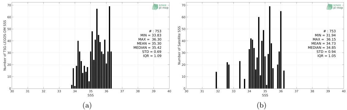
Figure 2: Histograms of SSS from TSG-LEGOS-DM (a) and SMOS L3 v2 - Monthly - 0.25 Deg (CATDS-CECOS-IFREMER) (b) considering all match-up pairs per bins of 0.1 over the Congo river plume Pi-MEP region and for the full satellite product period.
