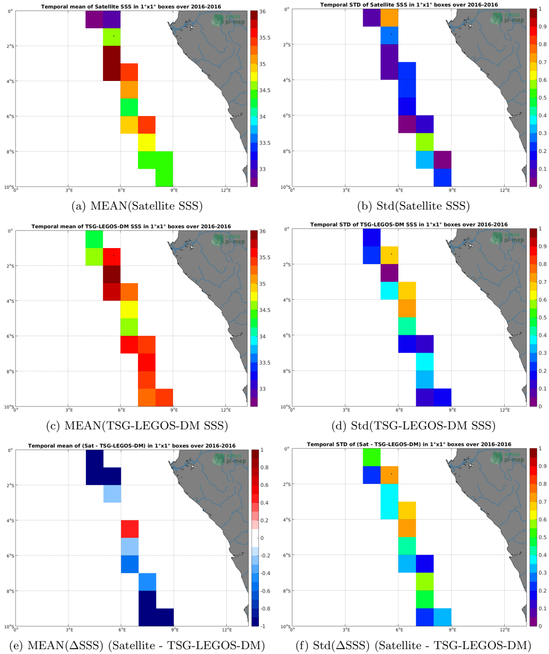
Figure 6: Temporal mean (left) and Std (right) of SSS from SMOS L3 v2 - Monthly - 0.25 Deg (CATDS-CECOS-IFREMER) (top), TSG-LEGOS-DM (middle), and of \Delta SSS (Satellite - TSG-LEGOS-DM). Only match-up pairs are used to generate these maps.
