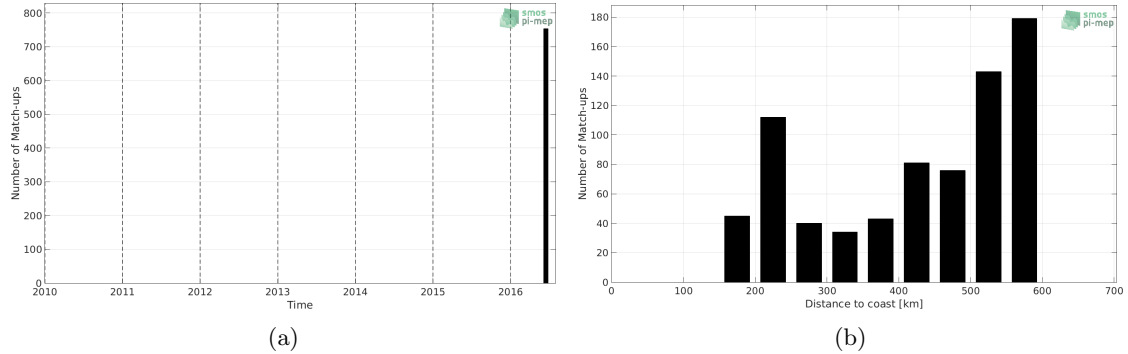
Figure 1: Number of match-ups between TSG-LEGOS-DM and SMOS-L3-CATDS-IFREMER-CECOS-V2-MONTHLY-0.25DEG SSS as a function of time (a) and as function of the distance to coast (b) over the Congo river plume Pi-MEP region and for the full satellite product period.
