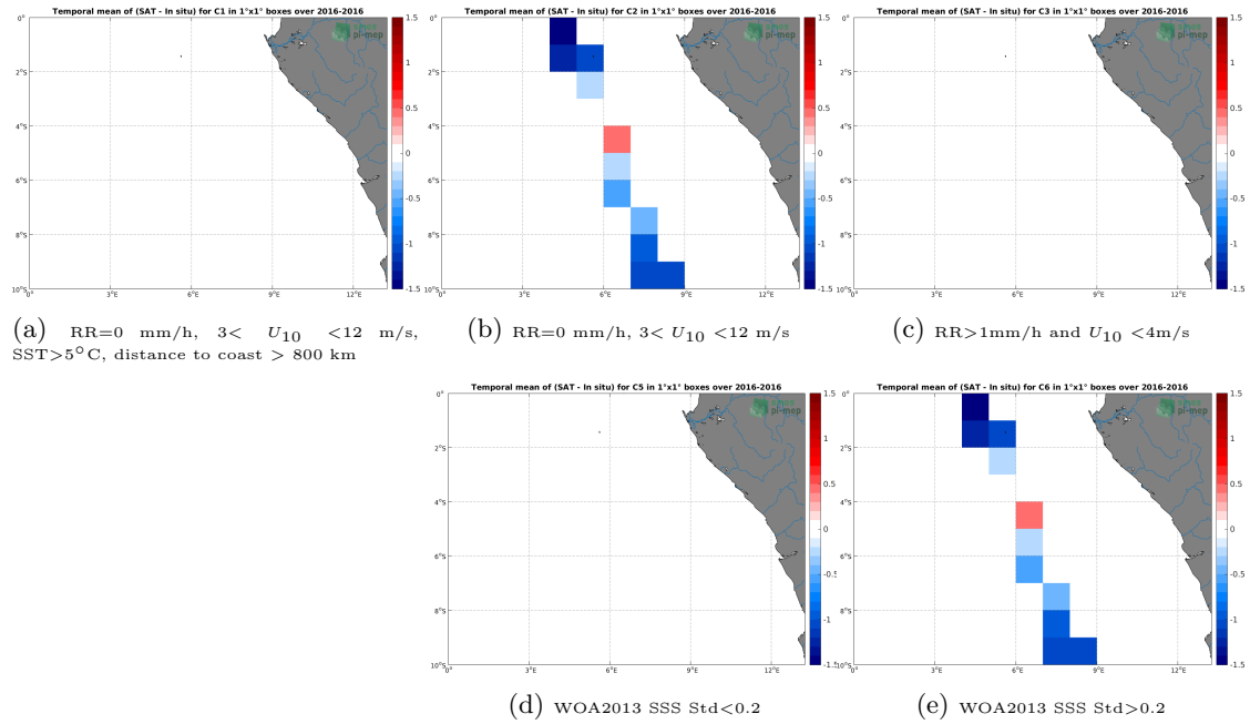
Figure 12: Temporal mean gridded over spatial boxes of size 1^\circ \times 1^\circ of \Delta SSS (SMOS-L3-CATDS-IFREMER-CECOS-V2-MONTHLY-0.25DEG - TSG-LEGOS-DM) for 5 different subdatasets corresponding to:RR=0 mm/h, 3 < U_{10} < 12 m/s, SST > 5^\circ\text{C} , distance to coast > 800 km (a), RR=0 mm/h, 3 < U_{10} < 12 m/s (b), RR > 1 mm/h and U_{10} < 4 m/s (c), WOA2013 SSS Std < 0.2 (d), WOA2013 SSS Std > 0.2 (e).
