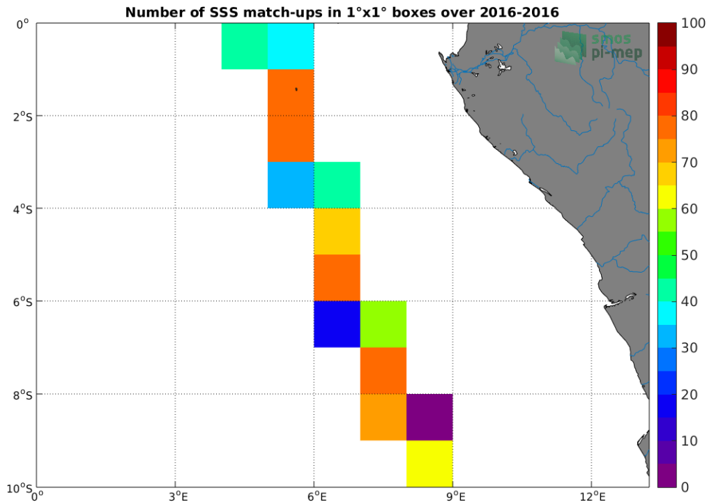
Figure 4: Number of SSS match-ups between TSG-LEGOS-DM SSS and the SMOS-L3-CATDS-IFREMER-CECOS-V2-MONTHLY-0.25DEG SSS product for the Congo river plume Pi-MEP region over 1°x1° boxes and for the full satellite product period.
