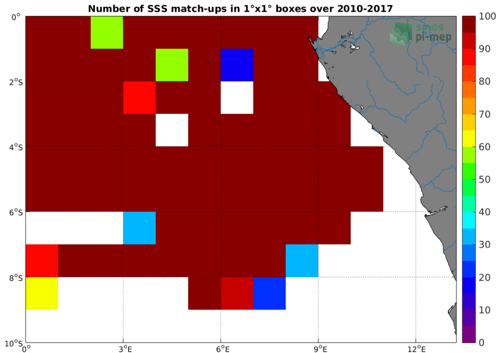
Figure 4: Number of SSS match-ups between TSG-GOSUD-Research-vessel SSS and the SMOS L3 v2 - Monthly - 0.25 Deg (CATDS-CECOS-IFREMER) SSS product for the Congo river plume Pi-MEP region over 1^\circ \times 1^\circ boxes and for the full satellite product period.
