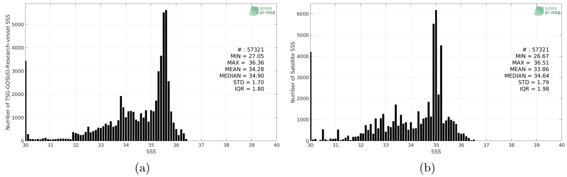
Figure 2: Histograms of SSS from TSG-GOSUD-Research-vessel (a) and SMOS-L3-CATDS-IFREMER-CECOS-V2-MONTHLY-0.25DEG (b) considering all match-up pairs per bins of 0.1 over the Congo river plume Pi-MEP region and for the full satellite product period.
