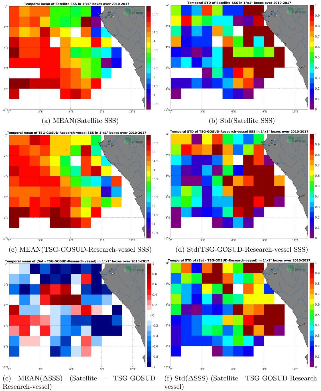
Figure 6: Temporal mean (left) and Std (right) of SSS from SMOS-L3-CATDS-IFREMER-CECOS-V2-MONTHLY-0.25DEG (top), TSG-GOSUD-Research-vessel (middle), and of \Delta SSS (Satellite - TSG-GOSUD-Research-vessel). Only match-up pairs are used to generate these maps.
