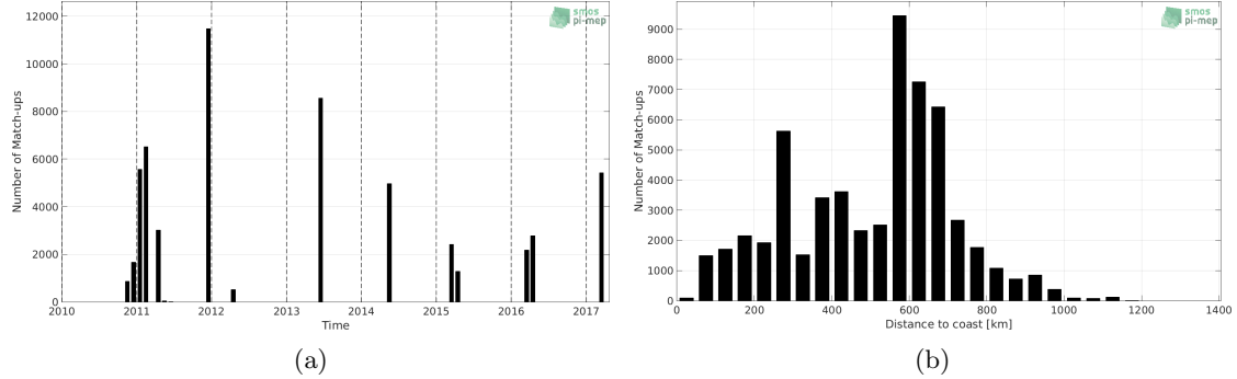
Figure 1: Number of match-ups between TSG-GOSUD-Research-vessel and SMOS-L3-CATDS-IFREMER-CECOS-V2-MONTHLY-0.25DEG SSS as a function of time (a) and as function of the distance to coast (b) over the Congo river plume Pi-MEP region and for the full satellite product period.
