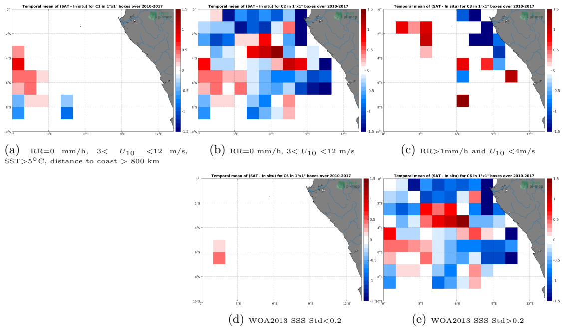
Figure 12: Temporal mean gridded over spatial boxes of size 1°x1° of \Delta SSS (SMOS-L3-CATDS-IFREMER-CECOS-V2-MONTHLY-0.25DEG - TSG-GOSUD-Research-vessel) for 5 different subdatasets corresponding to:RR=0 mm/h, 3 < U_{10} < 12 m/s, SST > 5°C, distance to coast > 800 km (a), RR=0 mm/h, 3 < U_{10} < 12 m/s (b), RR > 1mm/h and U_{10} < 4 m/s (c), WOA2013 SSS Std < 0.2 (d), WOA2013 SSS Std > 0.2 (e).
