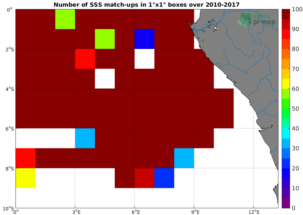
Figure 4: Number of SSS match-ups between TSG-GOSUD-Research-vessel SSS and the SMOS-L3-CATDS-IFREMER-CECOS-V2-MONTHLY-0.25DEG SSS product for the Congo river plume Pi-MEP region over 1^{\circ} \times 1^{\circ} boxes and for the full satellite product period.
