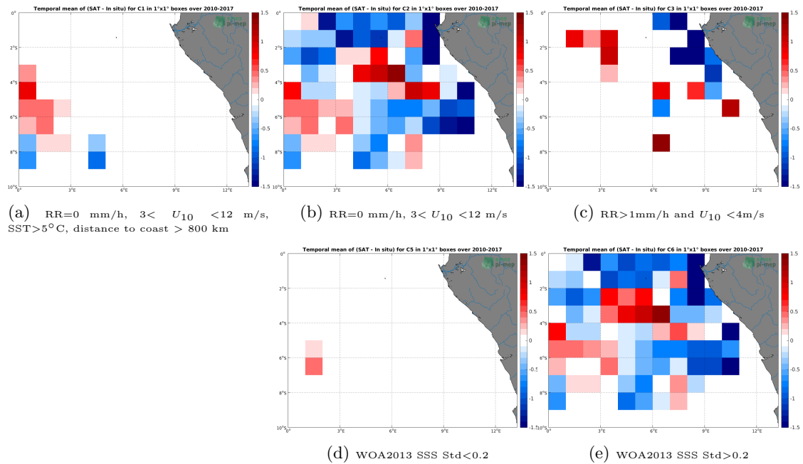
Figure 12: Temporal mean gridded over spatial boxes of size 1^\circ \times 1^\circ of \Delta SSS (SMOS-L3-CATDS-IFREMER-CECOS-V2-MONTHLY-0.25DEG - TSG-GOSUD-Research-vessel) for 5 different subdatasets corresponding to:RR=0 mm/h, 3 < U_{10} < 12 m/s, SST >5^\circ C, distance to coast > 800 km (a), RR=0 mm/h, 3 < U_{10} < 12 m/s (b), RR >1 mm/h and U_{10} < 4 m/s (c), WOA2013 SSS Std <0.2 (d), WOA2013 SSS Std >0.2 (e).
