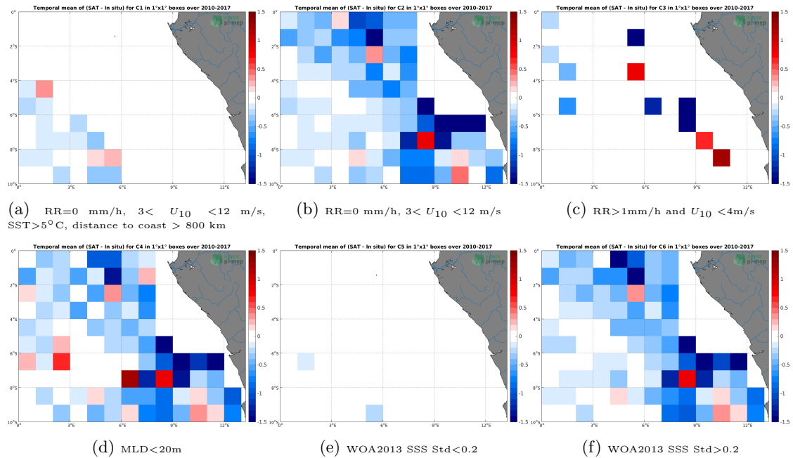
Figure 12: Temporal mean gridded over spatial boxes of size 1^\circ \times 1^\circ of \Delta SSS (SMOS L3 v2 - Monthly - 0.25 Deg (CATDS-CECOS-IFREMER) - Argo) for 6 different subdatasets corresponding to:RR=0 mm/h, 3 < U_{10} < 12 m/s, SST >5^\circ C, distance to coast > 800 km (a), RR=0 mm/h, 3 < U_{10} < 12 m/s (b), RR >1 mm/h and U_{10} < 4 m/s (c),MLD <20 m (d),WOA2013 SSS Std <0.2 (e),WOA2013 SSS Std >0.2 (f).
