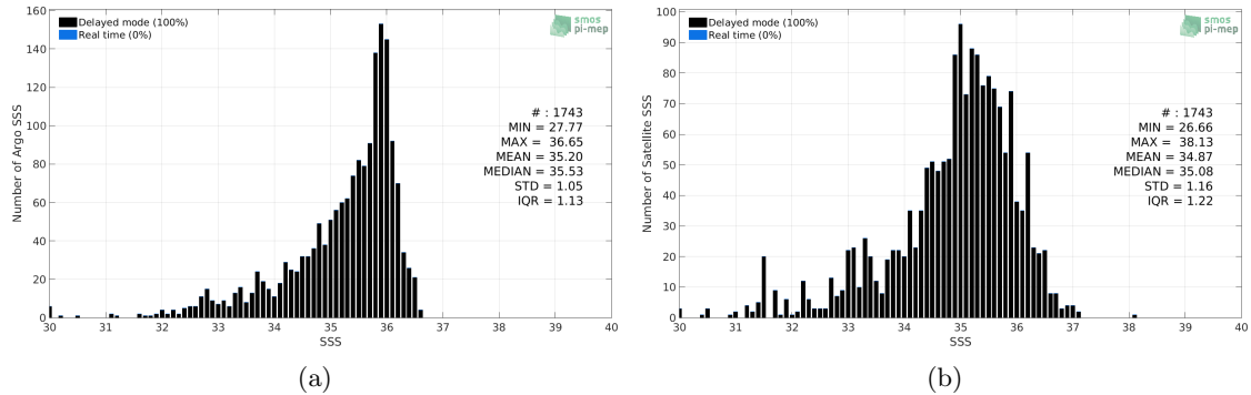
Figure 2: Histograms of SSS from Argo (a) and SMOS L3 v2 - Monthly - 0.25 Deg (CATDS-CECOS-IFREMER) (b) considering all match-up pairs per bins of 0.1 over the Congo river plume Pi-MEP region and for the full satellite product period.
