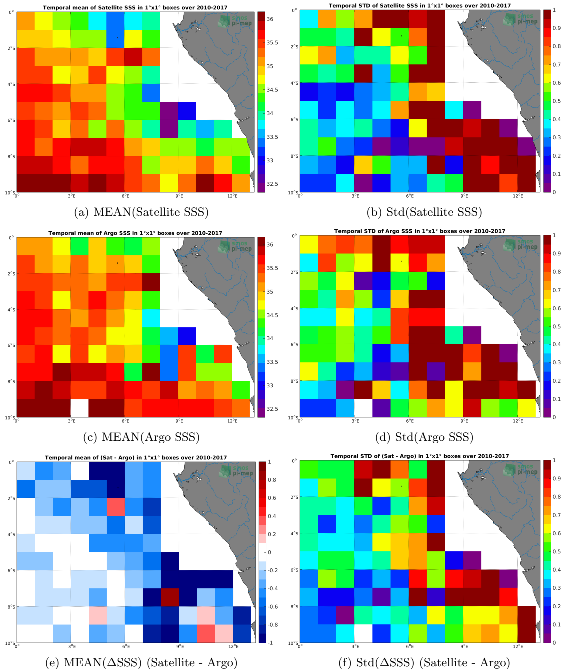
Figure 6: Temporal mean (left) and Std (right) of SSS from SMOS L3 v2 - Monthly - 0.25 Deg (CATDS-CECOS-IFREMER) (top), Argo (middle), and of \Delta SSS (Satellite - Argo). Only match-up pairs are used to generate these maps.
