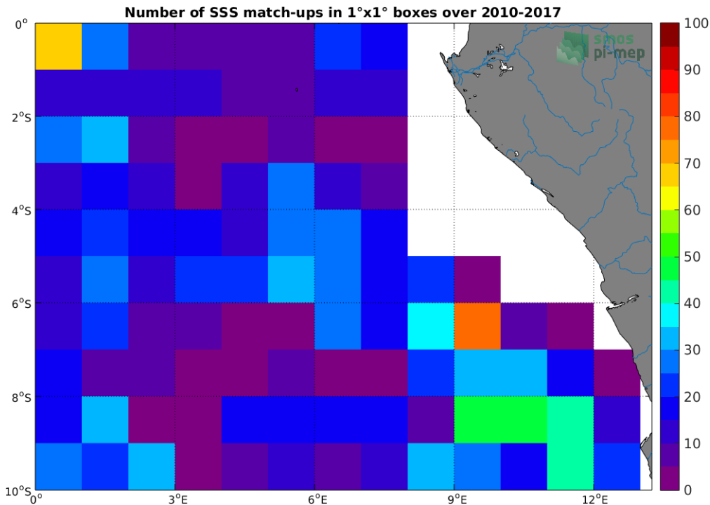
Figure 4: Number of SSS match-ups between Argo SSS and the SMOS L3 v2 - Monthly - 0.25 Deg (CATDS-CECOS-IFREMER) SSS product for the Congo river plume Pi-MEP region over 1°x1° boxes and for the full satellite product period.
