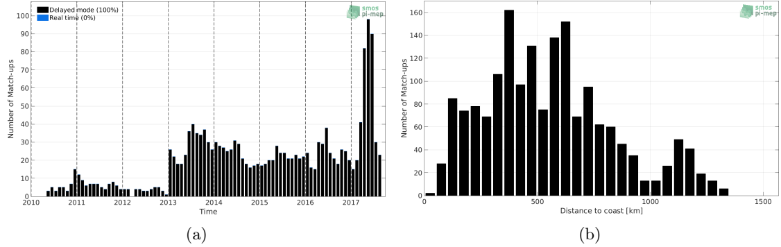
Figure 1: Number of match-ups between Argo and SMOS L3 v2 - Monthly - 0.25 Deg (CATDS-CECOS-IFREMER) SSS as a function of time (a) and as function of the distance to coast (b) over the Congo river plume Pi-MEP region and for the full satellite product period.
