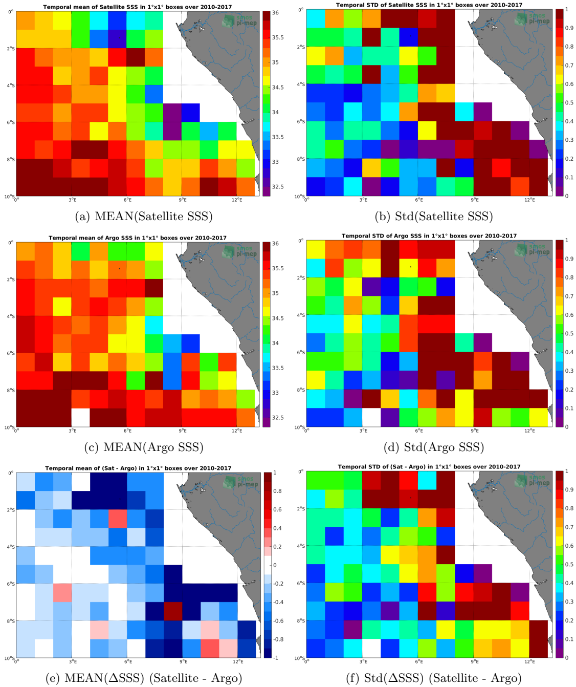
Figure 6: Temporal mean (left) and Std (right) of SSS from SMOS-L3-CATDS-IFREMER-CECOS-V2-MONTHLY-0.25DEG (top), Argo (middle), and of \Delta SSS (Satellite - Argo). Only match-up pairs are used to generate these maps.
