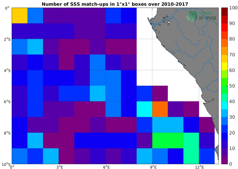
Figure 4: Number of SSS match-ups between Argo SSS and the SMOS-L3-CATDS-IFREMER-CECOS-V2-MONTHLY-0.25DEG SSS product for the Congo river plume Pi-MEP region over 1°x1° boxes and for the full satellite product period.
