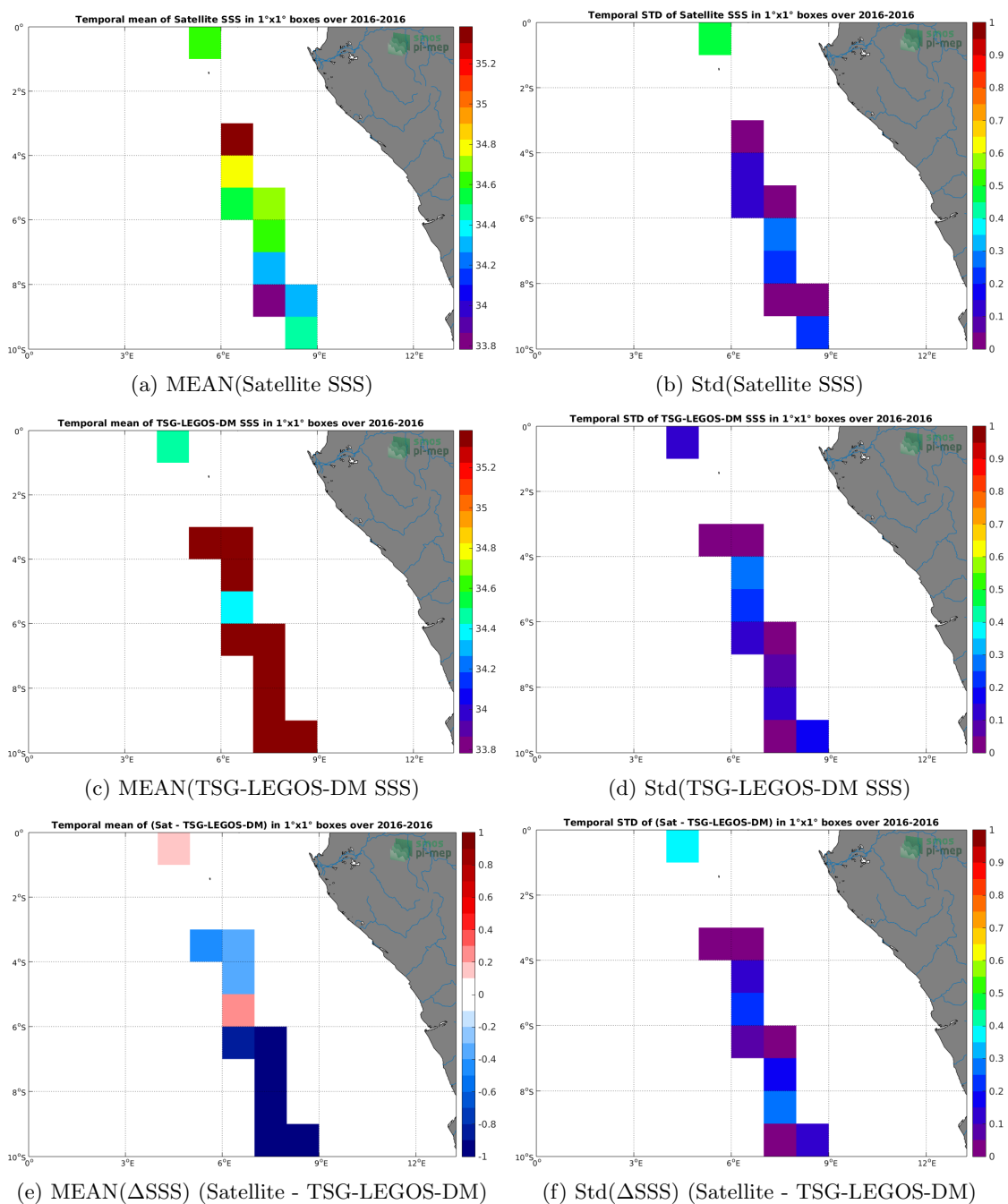
Figure 6: Temporal mean (left) and Std (right) of SSS from SMOS L3 v2 - Daily - 0.5 Deg (CATDS-CECOS-IFREMER) (top), TSG-LEGOS-DM (middle), and of \Delta SSS (Satellite - TSG-LEGOS-DM). Only match-up pairs are used to generate these maps.
