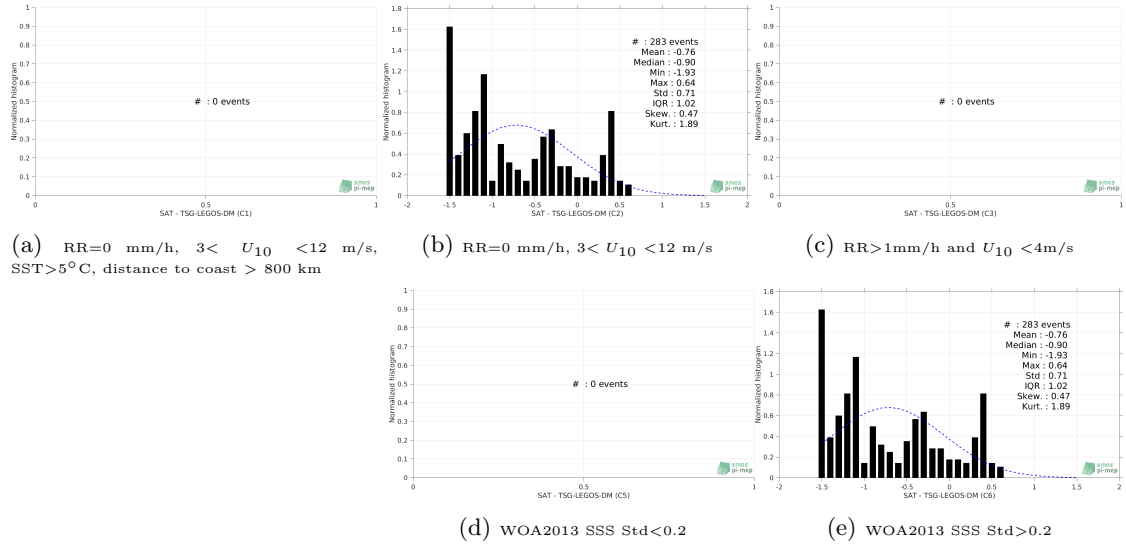
Figure 13: Normalized histogram of \Delta SSS (SMOS L3 v2 - Daily - 0.5 Deg (CATDS-CECOS-IFREMER) - TSG-LEGOS-DM) for 5 different subdatasets corresponding to: RR=0 mm/h, 3 < U_{10} < 12 m/s, SST > 5°C, distance to coast > 800 km (a), RR=0 mm/h, 3 < U_{10} < 12 m/s (b), RR > 1mm/h and U_{10} < 4 m/s (c), WOA2013 SSS Std < 0.2 (d), WOA2013 SSS Std > 0.2 (e).
