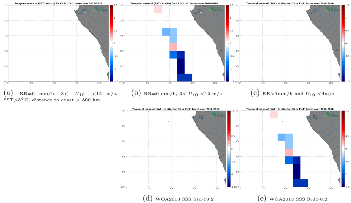
Figure 12: Temporal mean gridded over spatial boxes of size 1^{\circ}\times 1^{\circ} of \Delta\text{SSS} (SMOS L3 v2 - Daily - 0.5 Deg (CATDS-CECOS-IFREMER) - TSG-LEGOS-DM) for 5 different subdatasets corresponding to:RR=0 mm/h, 3 < U_{10} < 12 m/s, SST >5^{\circ}\text{C} , distance to coast > 800 km (a), RR=0 mm/h, 3 < U_{10} < 12 m/s (b), RR >1 mm/h and U_{10} < 4 m/s (c), WOA2013 SSS Std <0.2 (d), WOA2013 SSS Std >0.2 (e).
