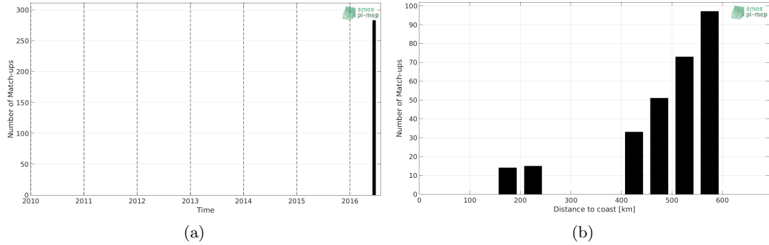
Figure 1: Number of match-ups between TSG-LEGOS-DM and SMOS L3 v2 - Daily - 0.5 Deg (CATDS-CECOS-IFREMER) SSS as a function of time (a) and as function of the distance to coast (b) over the Congo river plume Pi-MEP region and for the full satellite product period.
