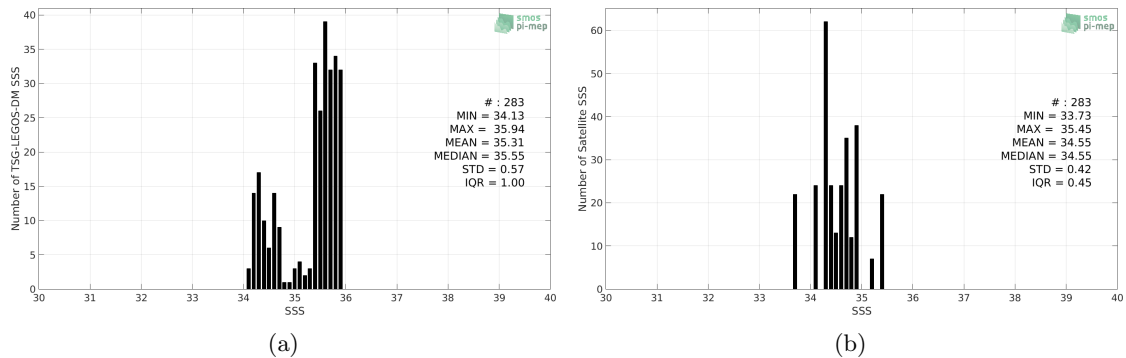
Figure 2: Histograms of SSS from TSG-LEGOS-DM (a) and SMOS L3 v2 - Daily - 0.5 Deg (CATDS-CECOS-IFREMER) (b) considering all match-up pairs per bins of 0.1 over the Congo river plume Pi-MEP region and for the full satellite product period.
