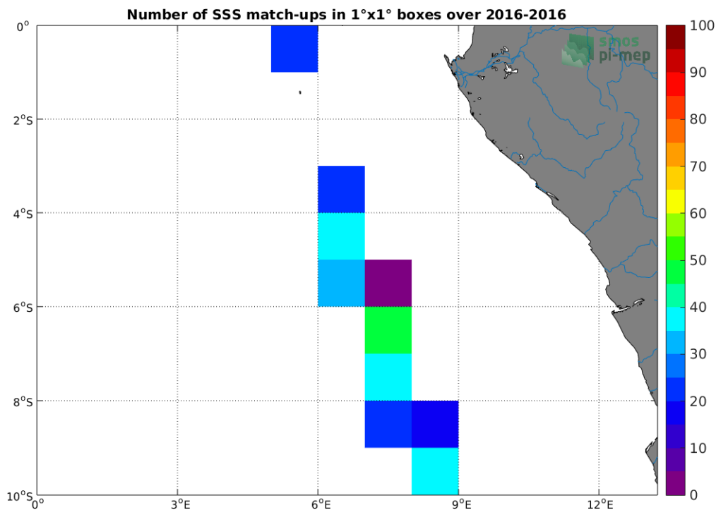
Figure 4: Number of SSS match-ups between TSG-LEGOS-DM SSS and the SMOS L3 v2 - Daily - 0.5 Deg (CATDS-CECOS-IFREMER) SSS product for the Congo river plume Pi-MEP region over 1°x1° boxes and for the full satellite product period.
