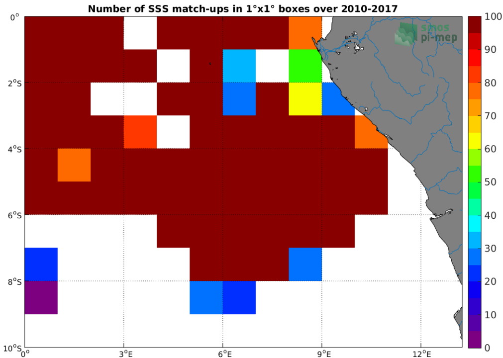
Figure 4: Number of SSS match-ups between TSG (GOSUD-Research-vessel) SSS and the SMOS SSS L3 v2 - Daily - 0.5 Deg (CATDS-CECOS-IFREMER) SSS product for the Congo river plume Pi-MEP region over 1^\circ \times 1^\circ boxes and for the full satellite product period.
