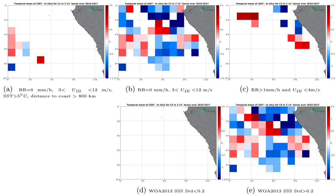
Figure 12: Temporal mean gridded over spatial boxes of size 1^\circ \times 1^\circ of \Delta SSS (SMOS SSS L3 v2 - Daily - 0.5 Deg (CATDS-CECOS-IFREMER) - TSG (GOSUD-Research-vessel)) for 5 different subdatasets corresponding to: RR=0 mm/h, 3 < U_{10} < 12 m/s, SST > 5^\circ\text{C} , distance to coast > 800 km (a), RR=0 mm/h, 3 < U_{10} < 12 m/s (b), RR > 1 mm/h and U_{10} < 4 m/s (c), WOA2013 SSS Std < 0.2 (d), WOA2013 SSS Std > 0.2 (e).
