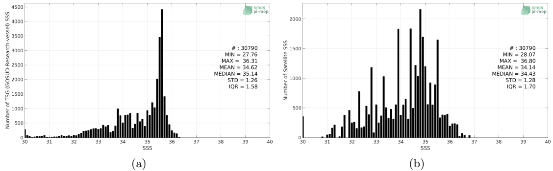
Figure 2: Histograms of SSS from TSG (GOSUD-Research-vessel) (a) and SMOS SSS L3 v2 - Daily - 0.5 Deg (CATDS-CECOS-IFREMER) (b) considering all match-up pairs per bins of 0.1 over the Congo river plume Pi-MEP region and for the full satellite product period.
