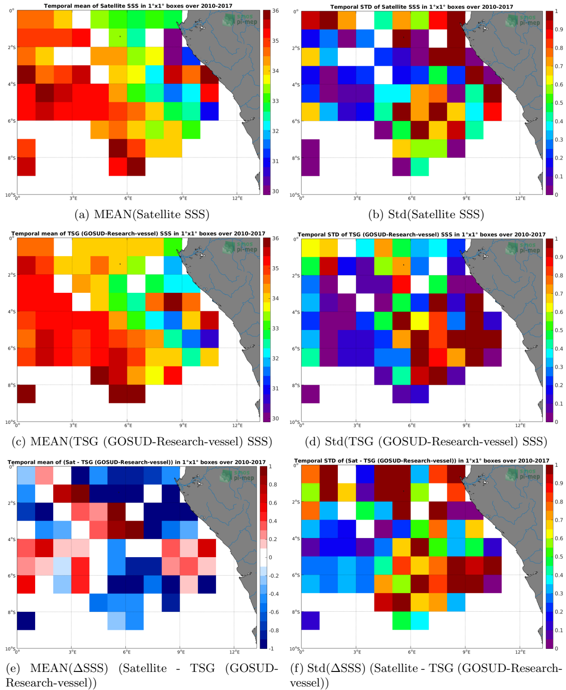
Figure 6: Temporal mean (left) and Std (right) of SSS from SMOS SSS L3 v2 - Daily - 0.5 Deg (CATDS-CECOS-IFREMER) (top), TSG (GOSUD-Research-vessel) (middle), and of \Delta SSS (Satellite - TSG (GOSUD-Research-vessel)). Only match-up pairs are used to generate these maps.
