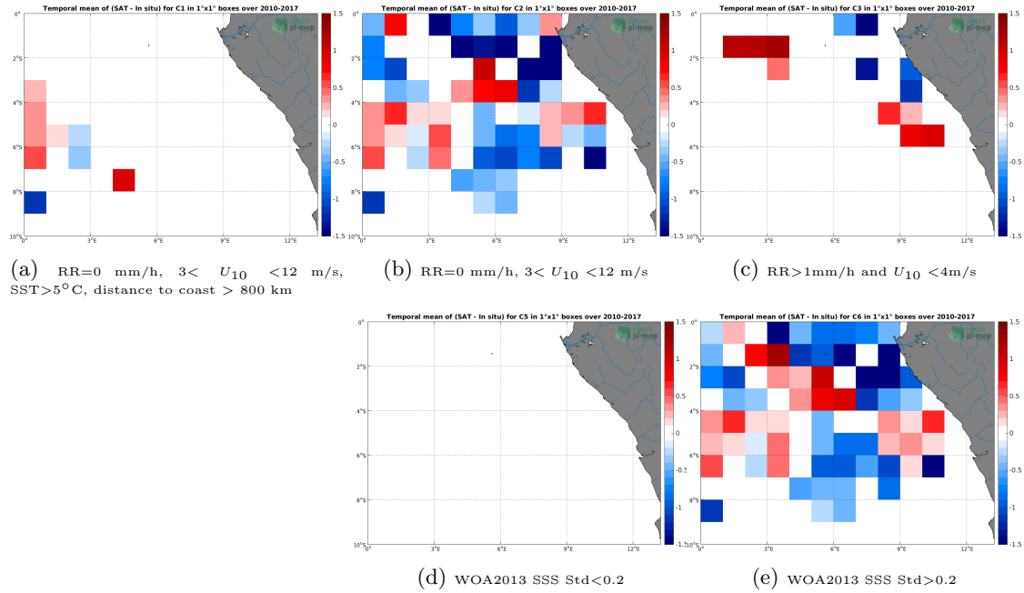
Figure 12: Temporal mean gridded over spatial boxes of size 1^{\circ}\times 1^{\circ} of \Delta SSS (SMOS L3 v2 - Daily - 0.5 Deg (CATDS-CECOS-IFREMER) - TSG-GOSUD-Research-vessel) for 5 different subdatasets corresponding to:RR=0 mm/h, 3 < U_{10} < 12 m/s, SST >5^{\circ}\text{C} , distance to coast > 800 km (a), RR=0 mm/h, 3 < U_{10} < 12 m/s (b), RR >1 mm/h and U_{10} < 4 m/s (c), WOA2013 SSS Std <0.2 (d), WOA2013 SSS Std >0.2 (e).
