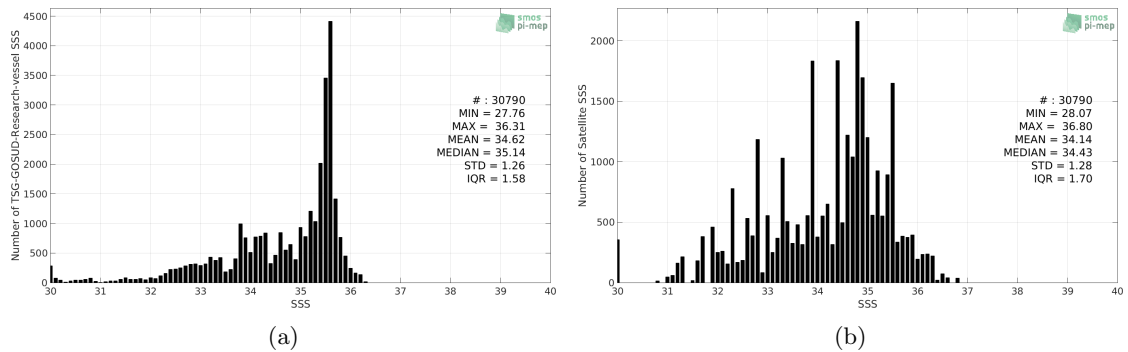
Figure 2: Histograms of SSS from TSG-GOSUD-Research-vessel (a) and SMOS L3 v2 - Daily - 0.5 Deg (CATDS-CECOS-IFREMER) (b) considering all match-up pairs per bins of 0.1 over the Congo river plume Pi-MEP region and for the full satellite product period.
