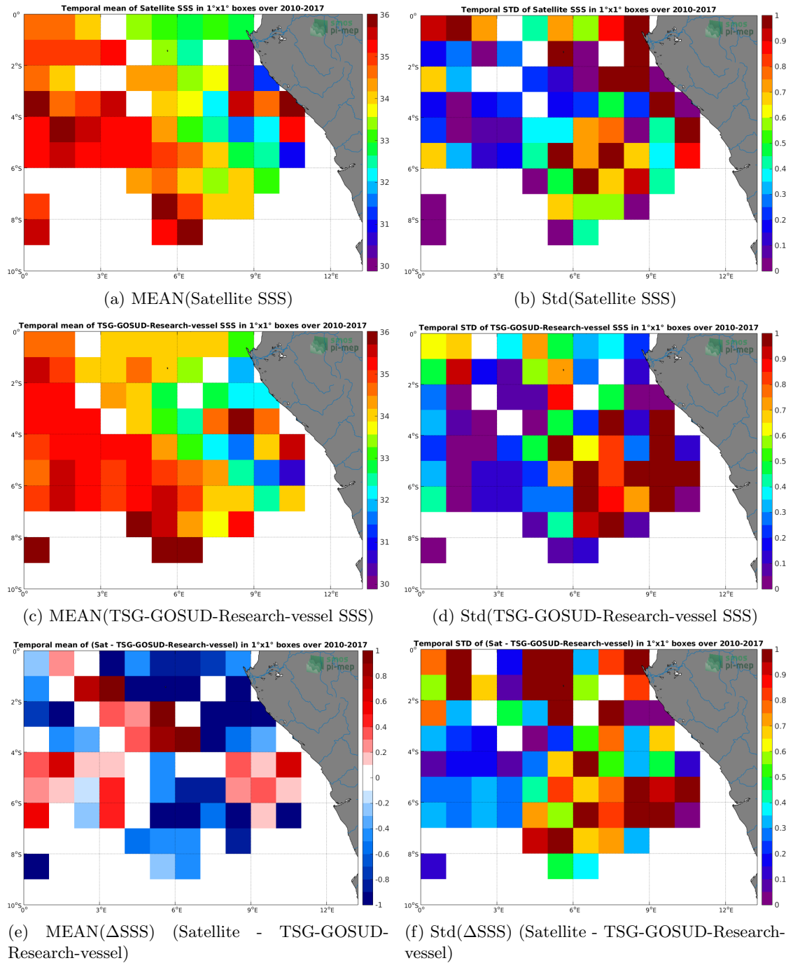
Figure 6: Temporal mean (left) and Std (right) of SSS from SMOS L3 v2 - Daily - 0.5 Deg (CATDS-CECOS-IFREMER) (top), TSG-GOSUD-Research-vessel (middle), and of \Delta SSS (Satellite - TSG-GOSUD-Research-vessel). Only match-up pairs are used to generate these maps.
