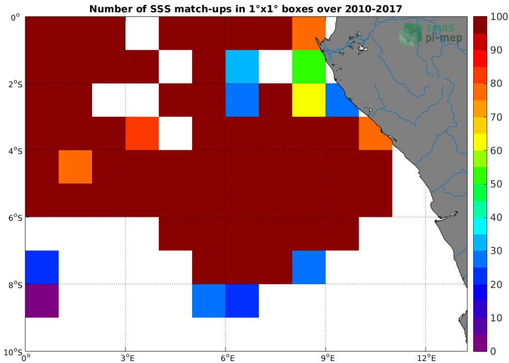
Figure 4: Number of SSS match-ups between TSG-GOSUD-Research-vessel SSS and the SMOS L3 v2 - Daily - 0.5 Deg (CATDS-CECOS-IFREMER) SSS product for the Congo river plume Pi-MEP region over 1°x1° boxes and for the full satellite product period.
