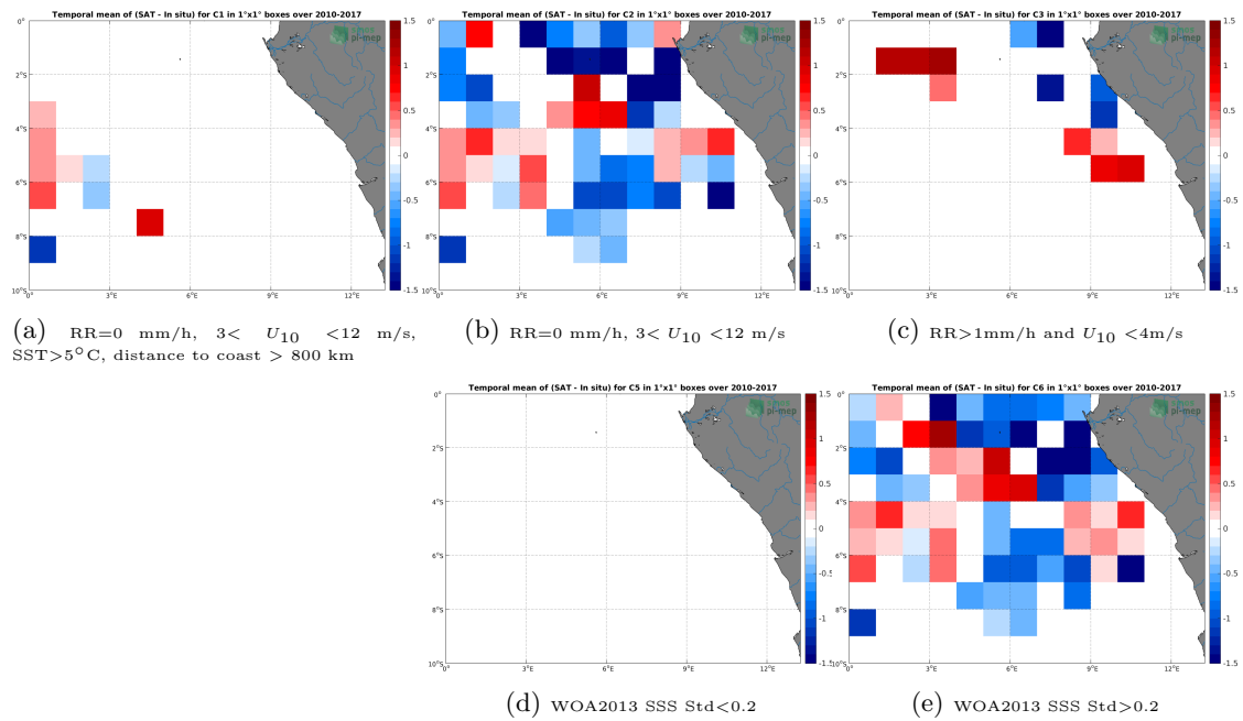
Figure 12: Temporal mean gridded over spatial boxes of size 1^\circ \times 1^\circ of \Delta SSS (SMOS-L3-CATDS-CECOS-IFREMER-V2-1DAY-0.5DEG - TSG-GOSUD-Research-vessel) for 5 different subdatasets corresponding to:RR=0 mm/h, 3 < U_{10} < 12 m/s, SST > 5^\circ\text{C} , distance to coast > 800 km (a), RR=0 mm/h, 3 < U_{10} < 12 m/s (b), RR > 1 mm/h and U_{10} < 4 m/s (c), WOA2013 SSS Std < 0.2 (d), WOA2013 SSS Std > 0.2 (e).
