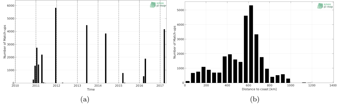
Figure 1: Number of match-ups between TSG-GOSUD-Research-vessel and SMOS-L3-CATDS-CECOS-IFREMER-V2-1DAY-0.5DEG SSS as a function of time (a) and as function of the distance to coast (b) over the Congo river plume Pi-MEP region and for the full satellite product period.
