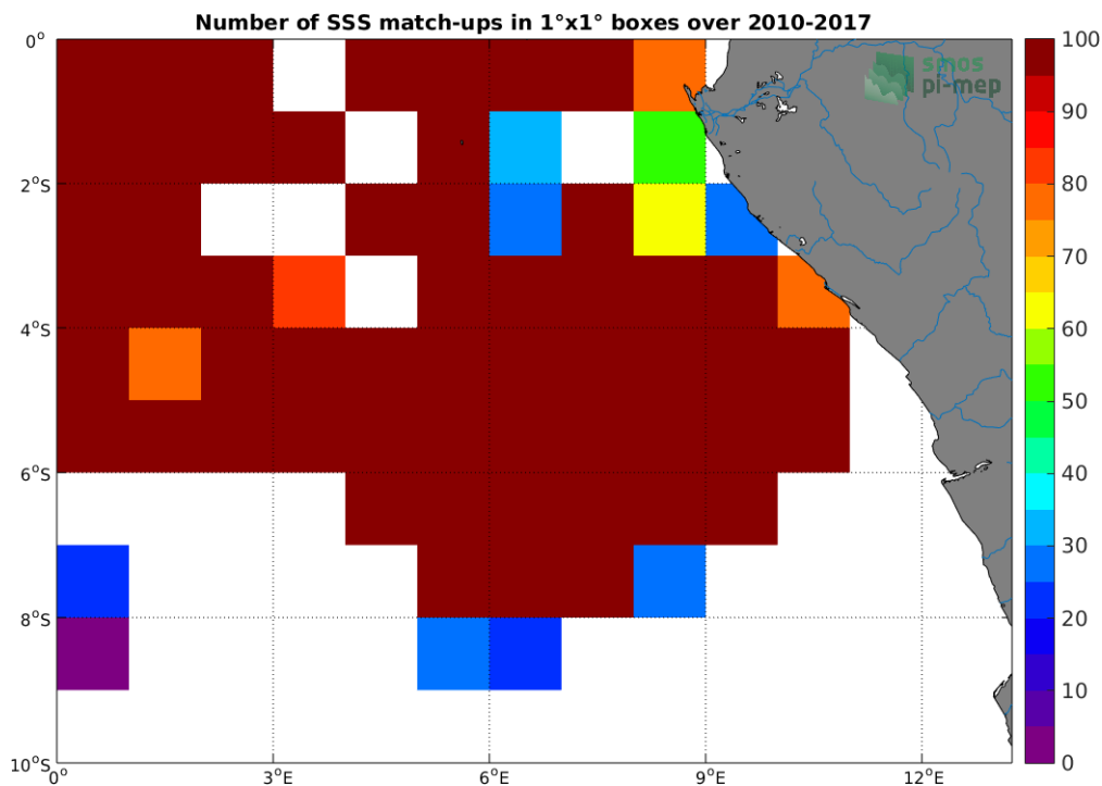
Figure 4: Number of SSS match-ups between TSG-GOSUD-Research-vessel SSS and the SMOS-L3-CATDS-CECOS-IFREMER-V2-1DAY-0.5DEG SSS product for the Congo river plume Pi-MEP region over 1°x1° boxes and for the full satellite product period.
