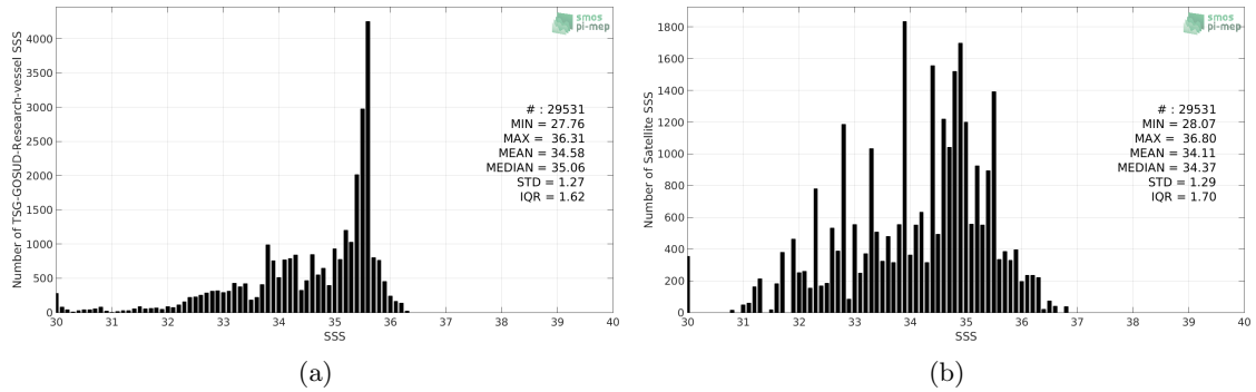
Figure 2: Histograms of SSS from TSG-GOSUD-Research-vessel (a) and SMOS-L3-CATDS-CECOS-IFREMER-V2-1DAY-0.5DEG (b) considering all match-up pairs per bins of 0.1 over the Congo river plume Pi-MEP region and for the full satellite product period.
