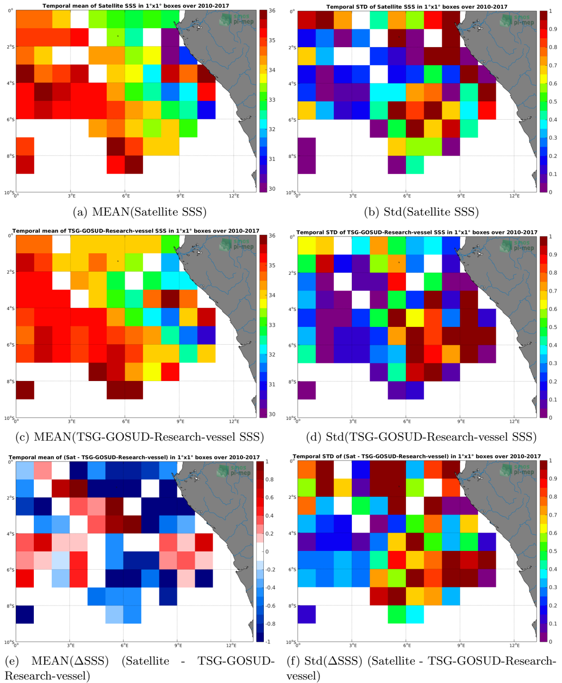
Figure 6: Temporal mean (left) and Std (right) of SSS from SMOS-L3-CATDS-CECOS-IFREMER-V2-1DAY-0.5DEG (top), TSG-GOSUD-Research-vessel (middle), and of \Delta SSS (Satellite - TSG-GOSUD-Research-vessel). Only match-up pairs are used to generate these maps.
