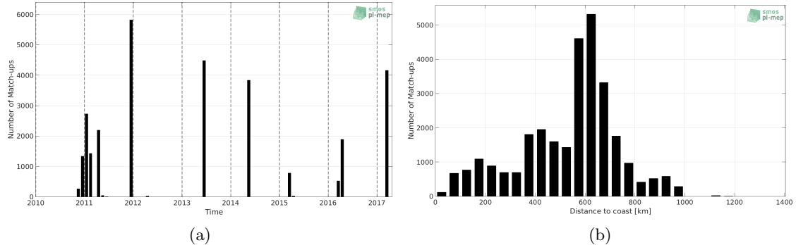
Figure 1: Number of match-ups between TSG-GOSUD-Research-vessel and SMOS-L3-CATDS-CECOS-IFREMER-V2-1DAY-0.5DEG SSS as a function of time (a) and as function of the distance to coast (b) over the Congo river plume Pi-MEP region and for the full satellite product period.
