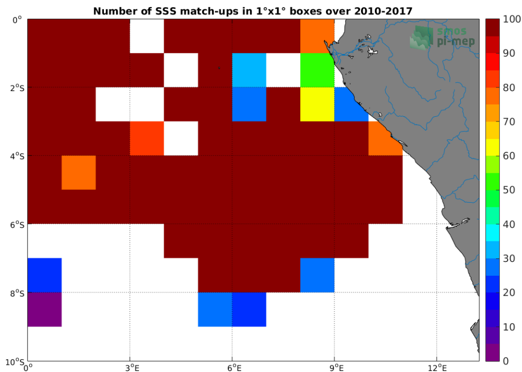
Figure 4: Number of SSS match-ups between TSG-GOSUD-Research-vessel SSS and the SMOS-L3-CATDS-CECOS-IFREMER-V2-1DAY-0.5DEG SSS product for the Congo river plume Pi-MEP region over 1^\circ \times 1^\circ boxes and for the full satellite product period.
