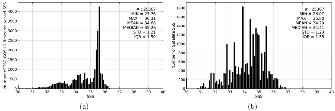
Figure 2: Histograms of SSS from TSG-GOSUD-Research-vessel (a) and SMOS-L3-CATDS-CECOS-IFREMER-V2-1DAY-0.5deg (b) considering all match-up pairs per bins of 0.1 over the Congo river plume Pi-MEP region and for the full satellite product period.
