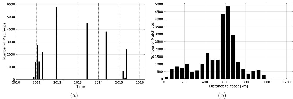
Figure 1: Number of match-ups between TSG-GOSUD-Research-vessel and SMOS-L3-CATDS-CECOS-IFREMER-V2-1DAY-0.5deg SSS as a function of time (a) and as function of the distance to coast (b) over the Congo river plume Pi-MEP region and for the full satellite product period.
