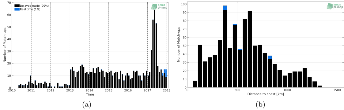
Figure 1: Number of match-ups between Argo and SMOS SSS L3 v2 - Daily - 0.5 Deg (CATDS-CECOS-IFREMER) SSS as a function of time (a) and as function of the distance to coast (b) over the Congo river plume Pi-MEP region and for the full satellite product period.
