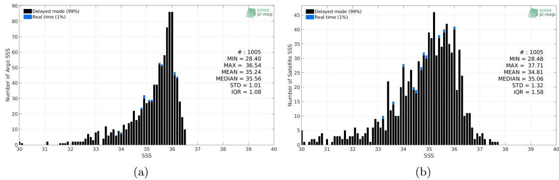
Figure 2: Histograms of SSS from Argo (a) and SMOS SSS L3 v2 - Daily - 0.5 Deg (CATDS-CECOS-IFREMER) (b) considering all match-up pairs per bins of 0.1 over the Congo river plume Pi-MEP region and for the full satellite product period.
