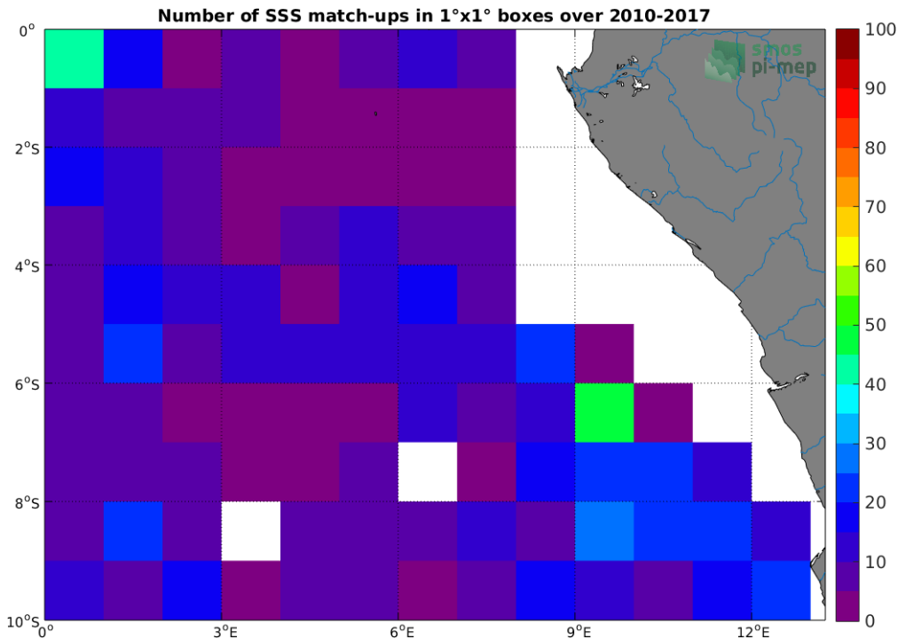
Figure 4: Number of SSS match-ups between Argo SSS and the SMOS SSS L3 v2 - Daily - 0.5 Deg (CATDS-CECOS-IFREMER) SSS product for the Congo river plume Pi-MEP region over 1^\circ \times 1^\circ boxes and for the full satellite product period.
