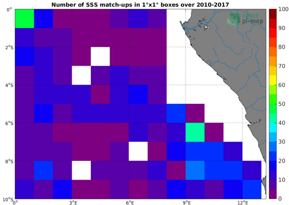
Figure 4: Number of SSS match-ups between Argo SSS and the SMOS-L3-CATDS-CECOS-IFREMER-V2-1DAY-0.5DEG SSS product for the Congo river plume Pi-MEP region over 1^\circ \times 1^\circ boxes and for the full satellite product period.
