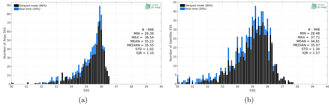
Figure 2: Histograms of SSS from Argo (a) and SMOS-L3-CATDS-CECOS-IFREMER-V2-1DAY-0.5DEG (b) considering all match-up pairs per bins of 0.1 over the Congo river plume Pi-MEP region and for the full satellite product period.
