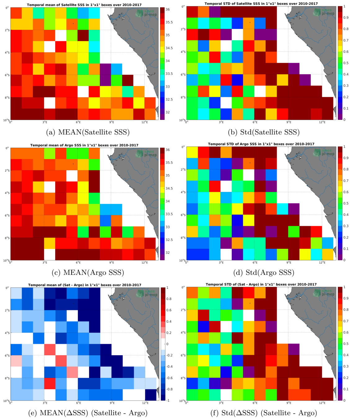
Figure 6: Temporal mean (left) and Std (right) of SSS from SMOS-L3-CATDS-CECOS-IFREMER-V2-1DAY-0.5DEG (top), Argo (middle), and of \Delta SSS (Satellite - Argo). Only match-up pairs are used to generate these maps.
