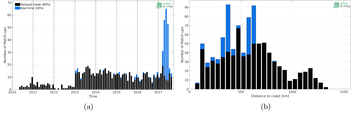
Figure 1: Number of match-ups between Argo and SMOS-L3-CATDS-CECOS-IFREMER-V2-1DAY-0.5DEG SSS as a function of time (a) and as function of the distance to coast (b) over the Congo river plume Pi-MEP region and for the full satellite product period.
