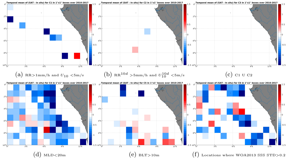
Figure 12: Temporal mean gridded over spatial boxes of size 1^\circ \times 1^\circ of \Delta SSS (SMOS-L3-CATDS-CECOS-IFREMER-V2-1DAY-0.5deg - Argo) for 6 different subdatasets corresponding to: RR > 1\text{mm/h} and U_{10} < 5\text{m/s} (a), RR^{10d} > 5\text{mm/h} and U_{10}^{10d} < 5\text{m/s} (b), C1 U C2 (c), MLD < 20\text{m} (d), BLT > 10\text{m} (e), Locations where WOA2013 SSS STD > 0.2 (f).
