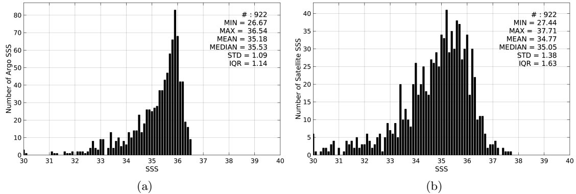
Figure 2: Histograms of SSS from Argo (a) and SMOS-L3-CATDS-CECOS-IFREMER-V2-1DAY-0.5deg (b) considering all match-up pairs per bins of 0.1 over the Congo river plume Pi-MEP region and for the full satellite product period.
