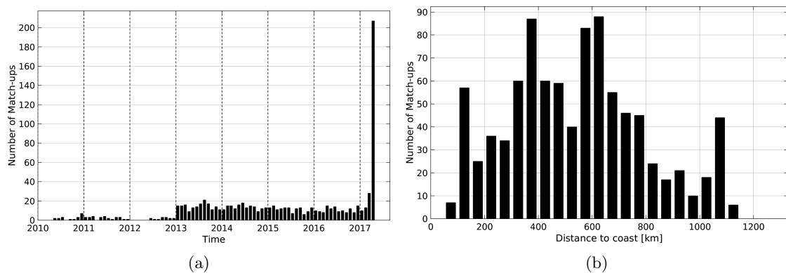
Figure 1: Number of match-ups between Argo and SMOS-L3-CATDS-CECOS-IFREMER-V2-1DAY-0.5deg SSS as a function of time (a) and as function of the distance to coast (b) over the Congo river plume Pi-MEP region and for the full satellite product period.
