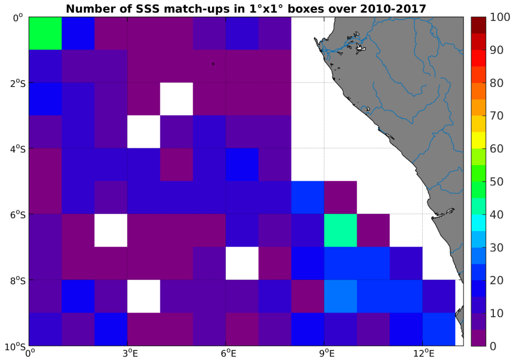
Figure 4: Number of SSS match-ups between Argo SSS and the SMOS-L3-CATDS-CECOS-IFREMER-V2-1DAY-0.5deg SSS product for the Congo river plume Pi-MEP region over 1°x1° boxes and for the full satellite product period.
