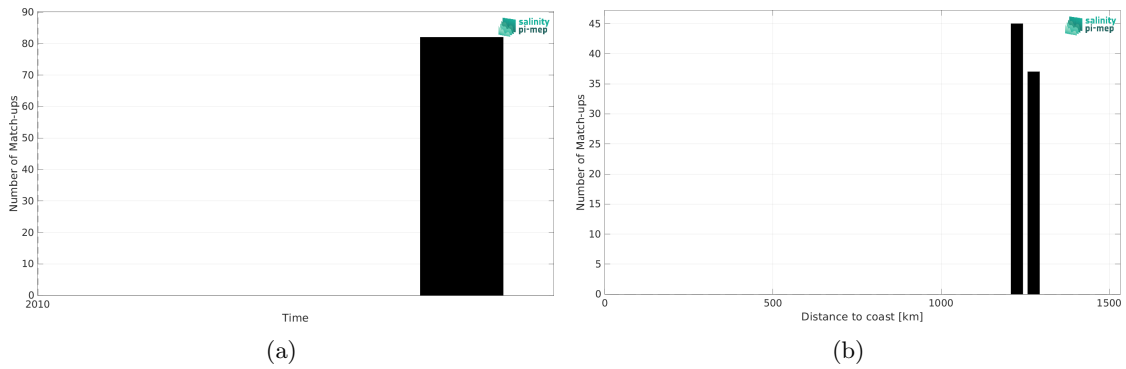
Figure 2: Number of match-ups between TSG (SAMOS) and SMOS SSS L3 v335 - Monthly - 25 km (CATDS-CPDC) SSS as a function of time (a) and as function of the distance to coast (b) over the Congo river plume Pi-MEP region and for the full satellite product period.
