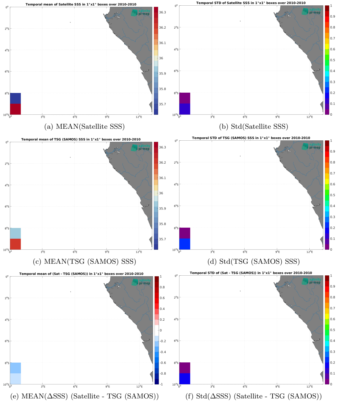
Figure 7: Temporal mean (left) and Std (right) of SSS from SMOS SSS L3 v335 - Monthly - 25 km (CATDS-CPDC) (top), TSG (SAMOS) (middle), and of \Delta SSS (Satellite - TSG (SAMOS)). Only match-up pairs are used to generate these maps.
