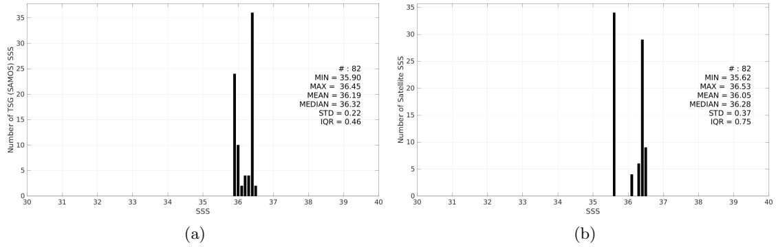
Figure 3: Histograms of SSS from TSG (SAMOS) (a) and SMOS SSS L3 v335 - Monthly - 25 km (CATDS-CPDC) (b) considering all match-up pairs per bins of 0.1 over the Congo river plume Pi-MEP region and for the full satellite product period.
