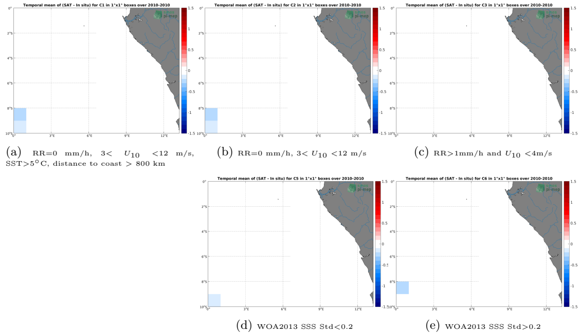
Figure 12: Temporal mean gridded over spatial boxes of size 1^\circ \times 1^\circ of \Delta SSS (SMOS SSS L3 v335 - Monthly - 25 km (CATDS-CPDC) - TSG (SAMOS)) for 5 different subdatasets corresponding to: RR=0 mm/h, 3 < U_{10} < 12 m/s, SST > 5^\circ C , distance to coast > 800 km (a), RR=0 mm/h, 3 < U_{10} < 12 m/s (b), RR > 1 mm/h and U_{10} < 4 m/s (c), WOA2013 SSS Std < 0.2 (d), WOA2013 SSS Std > 0.2 (e).
