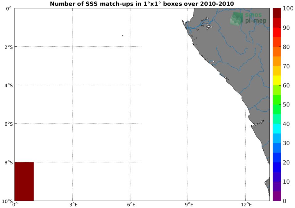
Figure 4: Number of SSS match-ups between TSG (SAMOS) SSS and the SMOS SSS L3 v335 - Monthly - 25 km (CATDS-CPDC) SSS product for the Congo river plume Pi-MEP region over 1^\circ \times 1^\circ boxes and for the full satellite product period.
