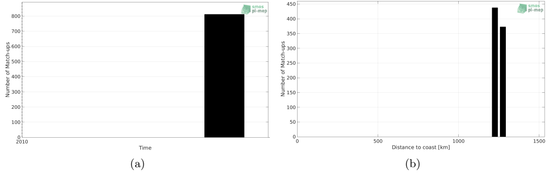
Figure 1: Number of match-ups between TSG (SAMOS) and SMOS SSS L3 v335 - Monthly - 25 km (CATDS-CPDC) SSS as a function of time (a) and as function of the distance to coast (b) over the Congo river plume Pi-MEP region and for the full satellite product period.
