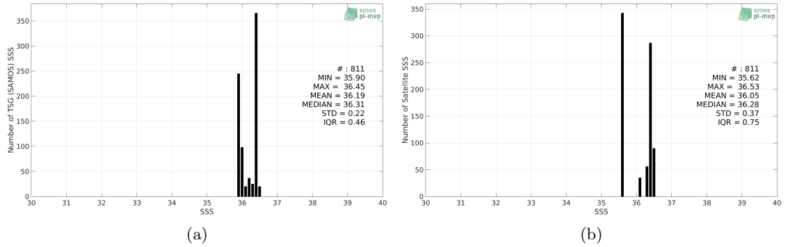
Figure 2: Histograms of SSS from TSG (SAMOS) (a) and SMOS SSS L3 v335 - Monthly - 25 km (CATDS-CPDC) (b) considering all match-up pairs per bins of 0.1 over the Congo river plume Pi-MEP region and for the full satellite product period.
