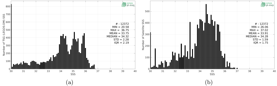
Figure 2: Histograms of SSS from TSG (LEGOS-DM) (a) and SMOS SSS L3 v335 - Monthly - 25 km (CATDS-CPDC) (b) considering all match-up pairs per bins of 0.1 over the Congo river plume Pi-MEP region and for the full satellite product period.
