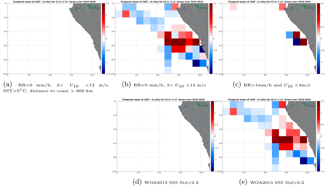
Figure 12: Temporal mean gridded over spatial boxes of size 1^{\circ}\times 1^{\circ} of \Delta\text{SSS} (SMOS SSS L3 v335 - Monthly - 25 km (CATDS-CPDC) - TSG (LEGOS-DM)) for 5 different subdatasets corresponding to: \text{RR}=0 mm/h, 3 < U_{10} < 12 m/s, \text{SST}>5^{\circ}\text{C} , distance to coast > 800 km (a), \text{RR}=0 mm/h, 3 < U_{10} < 12 m/s (b), \text{RR}>1\text{mm/h} and U_{10} < 4\text{m/s} (c), WOA2013 SSS Std <0.2 (d), WOA2013 SSS Std >0.2 (e).
