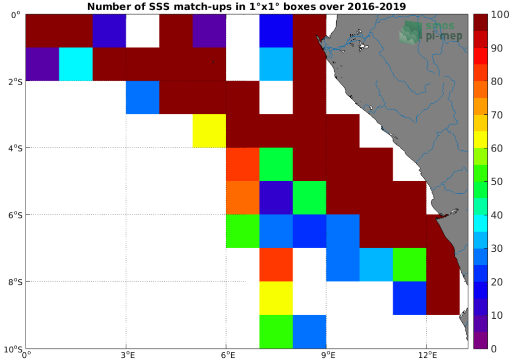
Figure 4: Number of SSS match-ups between TSG (LEGOS-DM) SSS and the SMOS SSS L3 v335 - Monthly - 25 km (CATDS-CPDC) SSS product for the Congo river plume Pi-MEP region over 1^\circ \times 1^\circ boxes and for the full satellite product period.
