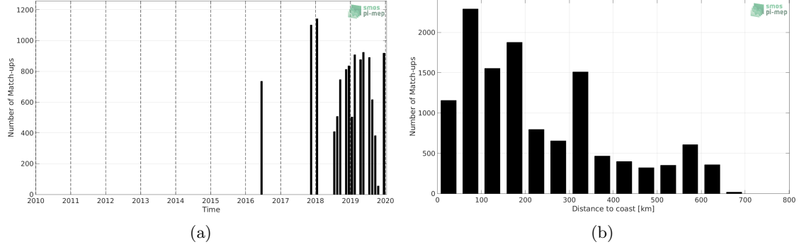
Figure 1: Number of match-ups between TSG (LEGOS-DM) and SMOS SSS L3 v335 - Monthly - 25 km (CATDS-CPDC) SSS as a function of time (a) and as function of the distance to coast (b) over the Congo river plume Pi-MEP region and for the full satellite product period.
