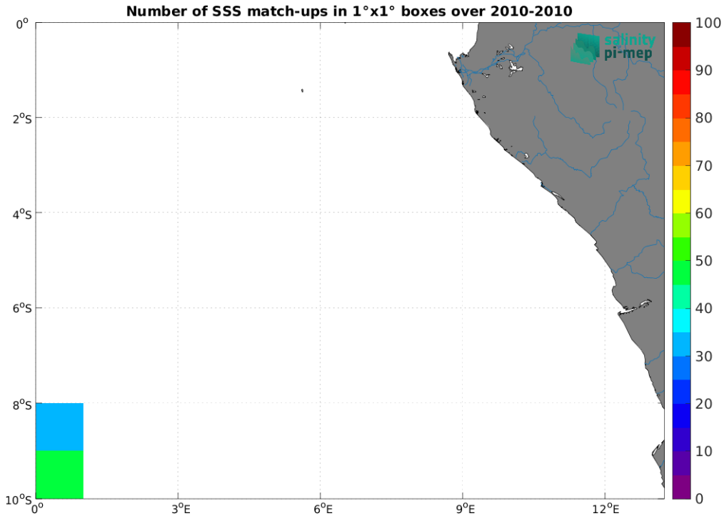
Figure 5: Number of SSS match-ups between TSG (SAMOS) SSS and the SMOS SSS L3 v335 - 10 Days - 25 km (CATDS-CPDC) SSS product for the Congo river plume Pi-MEP region over 1^\circ \times 1^\circ boxes and for the full satellite product period.
