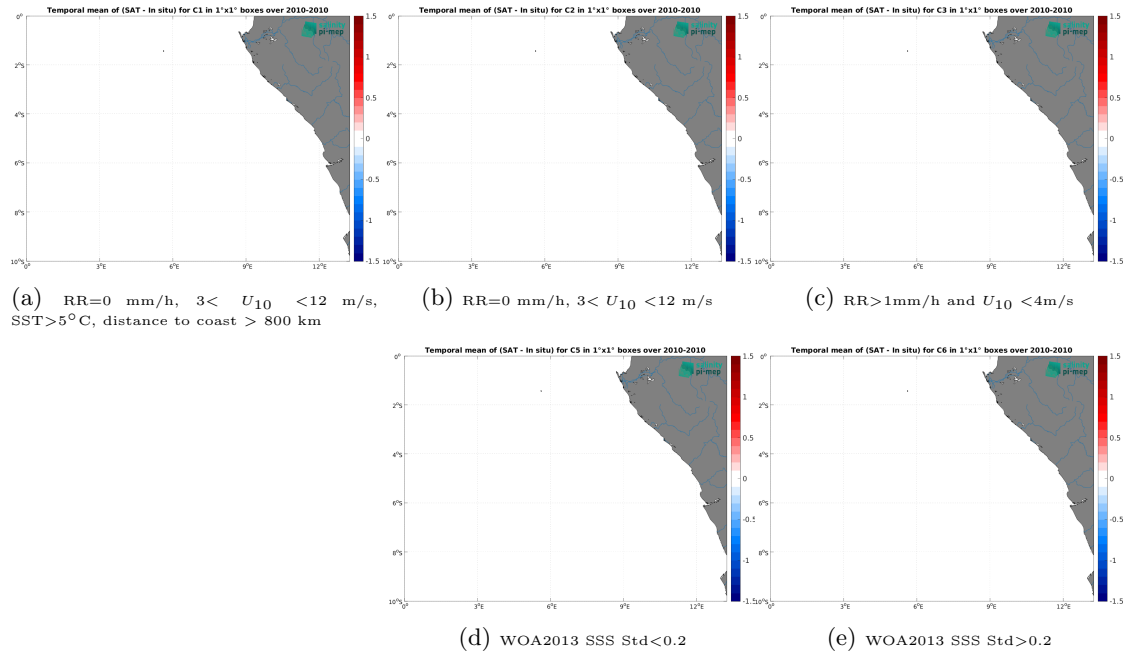
Figure 14: Temporal mean gridded over spatial boxes of size 1^\circ \times 1^\circ of \Delta SSS (SMOS SSS L3 v335 - 10 Days - 25 km (CATDS-CPDC) - TSG (SAMOS)) for 5 different subdatasets corresponding to:RR=0 mm/h, 3 < U_{10} < 12 m/s, SST >5^\circ C, distance to coast > 800 km (a), RR=0 mm/h, 3 < U_{10} < 12 m/s (b), RR >1 mm/h and U_{10} < 4 m/s (c), WOA2013 SSS Std <0.2 (d), WOA2013 SSS Std >0.2 (e).
