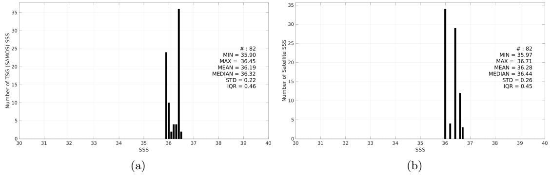
Figure 3: Histograms of SSS from TSG (SAMOS) (a) and SMOS SSS L3 v335 - 10 Days - 25 km (CATDS-CPDC) (b) considering all match-up pairs per bins of 0.1 over the Congo river plume Pi-MEP region and for the full satellite product period.
