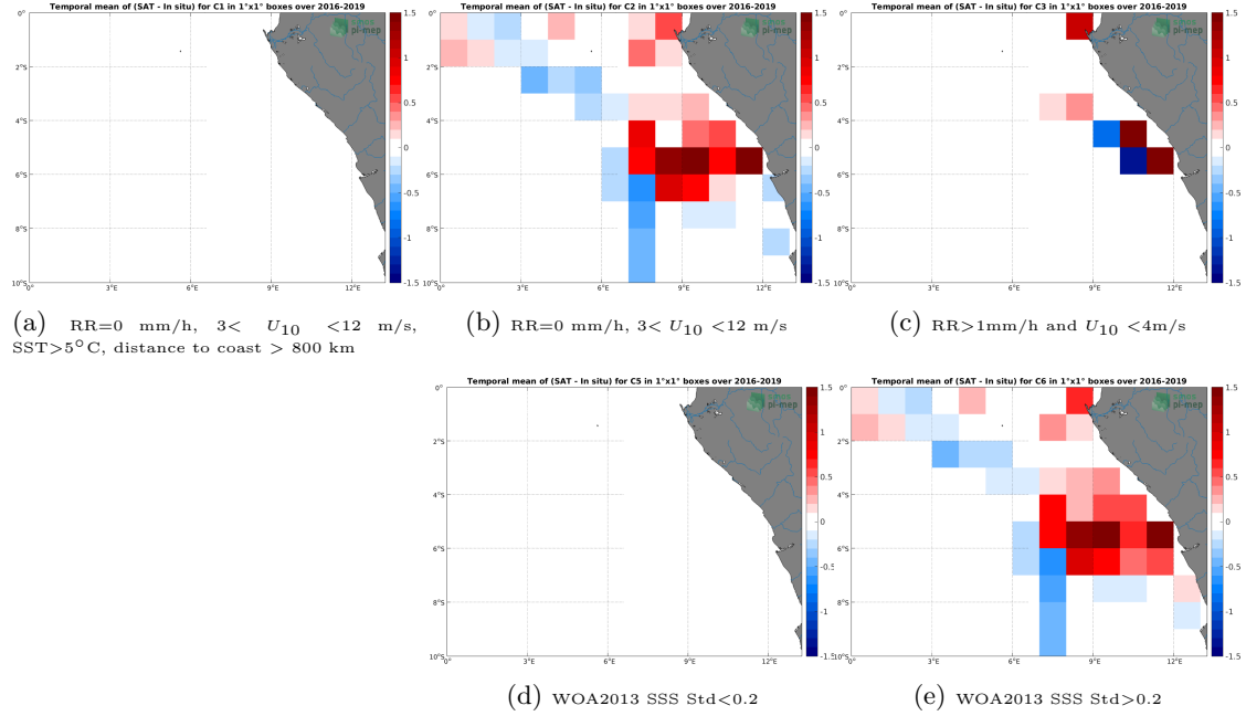
Figure 12: Temporal mean gridded over spatial boxes of size 1^{\circ}\times 1^{\circ} of \Delta\text{SSS} (SMOS SSS L3 v335 - 10 Days - 25 km (CATDS-CPDC) - TSG (LEGOS-DM)) for 5 different subdatasets corresponding to:RR=0 mm/h, 3 < U_{10} < 12 m/s, SST >5^{\circ}\text{C} , distance to coast > 800 km (a), RR=0 mm/h, 3 < U_{10} < 12 m/s (b), RR >1 mm/h and U_{10} < 4 m/s (c), WOA2013 SSS Std <0.2 (d), WOA2013 SSS Std >0.2 (e).
