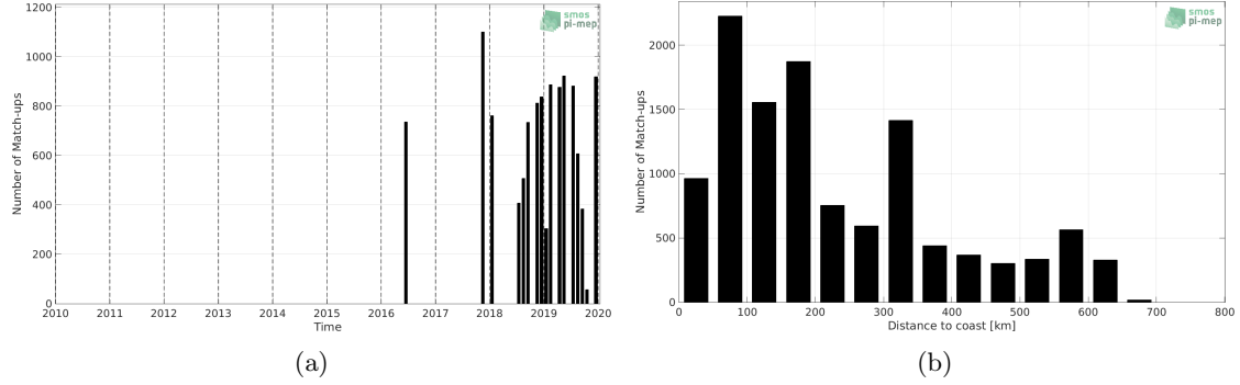
Figure 1: Number of match-ups between TSG (LEGOS-DM) and SMOS SSS L3 v335 - 10 Days - 25 km (CATDS-CPDC) SSS as a function of time (a) and as function of the distance to coast (b) over the Congo river plume Pi-MEP region and for the full satellite product period.
