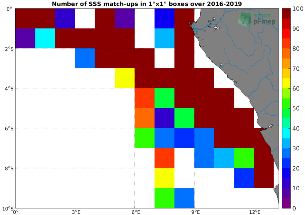
Figure 4: Number of SSS match-ups between TSG (LEGOS-DM) SSS and the SMOS SSS L3 v335 - 10 Days - 25 km (CATDS-CPDC) SSS product for the Congo river plume Pi-MEP region over 1^\circ \times 1^\circ boxes and for the full satellite product period.
