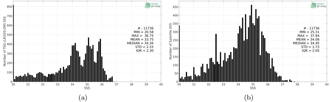
Figure 2: Histograms of SSS from TSG (LEGOS-DM) (a) and SMOS SSS L3 v335 - 10 Days - 25 km (CATDS-CPDC) (b) considering all match-up pairs per bins of 0.1 over the Congo river plume Pi-MEP region and for the full satellite product period.
