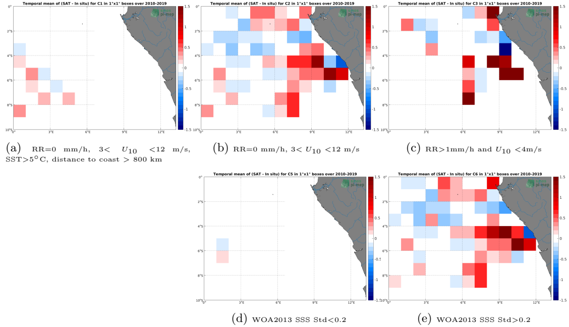
Figure 12: Temporal mean gridded over spatial boxes of size 1^\circ \times 1^\circ of \Delta SSS (SMOS SSS L3 v335 - 10 Days - 25 km (CATDS-CPDC) - TSG (GOSUD-Research-vessel)) for 5 different subdatasets corresponding to: RR=0 mm/h, 3 < U_{10} < 12 m/s, SST > 5^\circ\text{C} , distance to coast > 800 km (a), RR=0 mm/h, 3 < U_{10} < 12 m/s (b), RR > 1 mm/h and U_{10} < 4 m/s (c), WOA2013 SSS Std < 0.2 (d), WOA2013 SSS Std > 0.2 (e).
