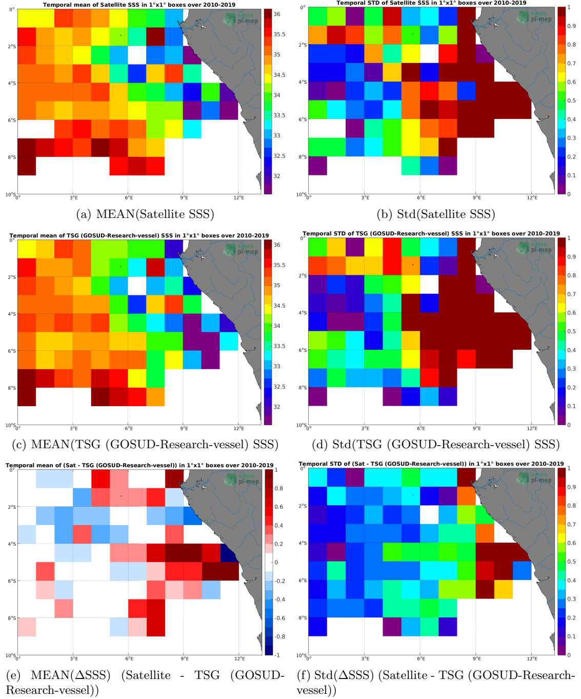
Figure 6: Temporal mean (left) and Std (right) of SSS from SMOS SSS L3 v335 - 10 Days - 25 km (CATDS-CPDC) (top), TSG (GOSUD-Research-vessel) (middle), and of \Delta SSS (Satellite - TSG (GOSUD-Research-vessel)). Only match-up pairs are used to generate these maps.
