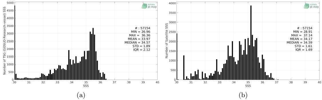
Figure 2: Histograms of SSS from TSG (GOSUD-Research-vessel) (a) and SMOS SSS L3 v335 - 10 Days - 25 km (CATDS-CPDC) (b) considering all match-up pairs per bins of 0.1 over the Congo river plume Pi-MEP region and for the full satellite product period.
