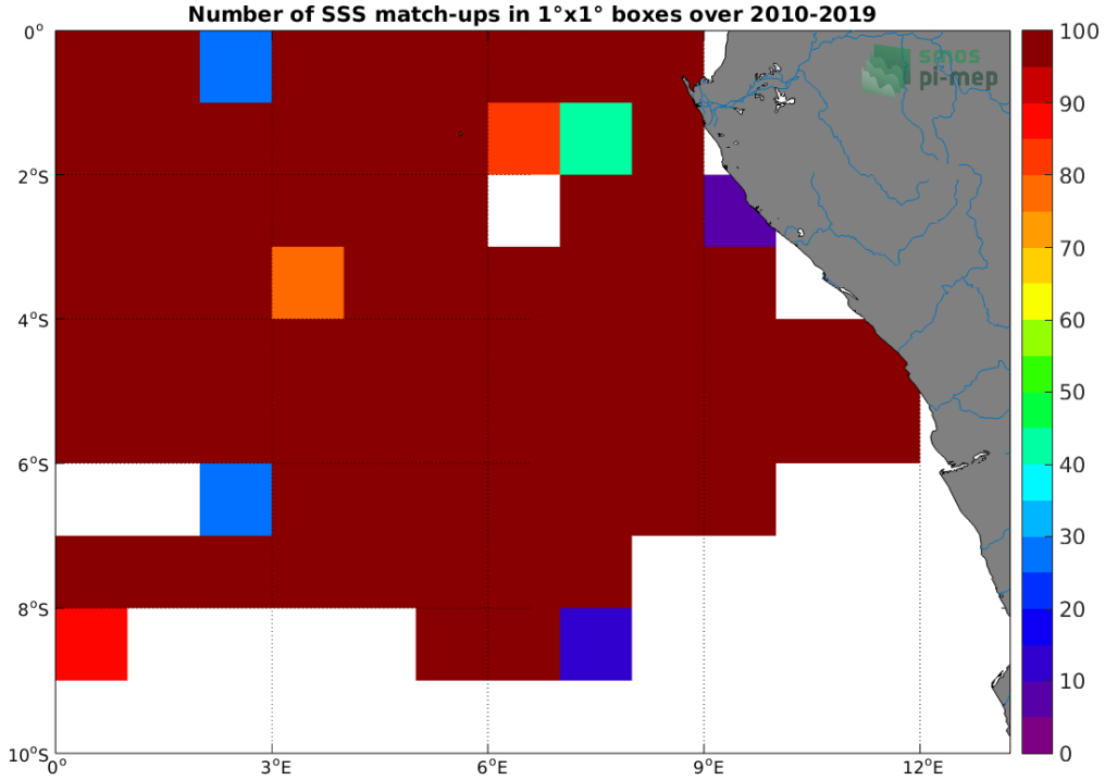
Figure 4: Number of SSS match-ups between TSG (GOSUD-Research-vessel) SSS and the SMOS SSS L3 v335 - 10 Days - 25 km (CATDS-CPDC) SSS product for the Congo river plume Pi-MEP region over 1^\circ \times 1^\circ boxes and for the full satellite product period.
