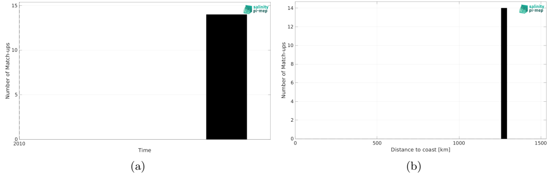
Figure 2: Number of match-ups between TSG (SAMOS) and SMOS SSS L2Q v333 - 0.25 Deg (CATDS-CPDC) SSS as a function of time (a) and as function of the distance to coast (b) over the Congo river plume Pi-MEP region and for the full satellite product period.
