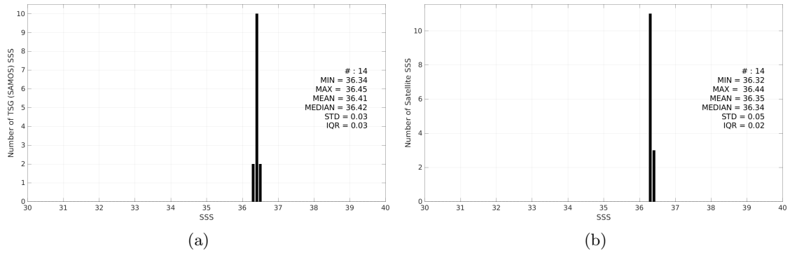
Figure 3: Histograms of SSS from TSG (SAMOS) (a) and SMOS SSS L2Q v333 - 0.25 Deg (CATDS-CPDC) (b) considering all match-up pairs per bins of 0.1 over the Congo river plume Pi-MEP region and for the full satellite product period.
