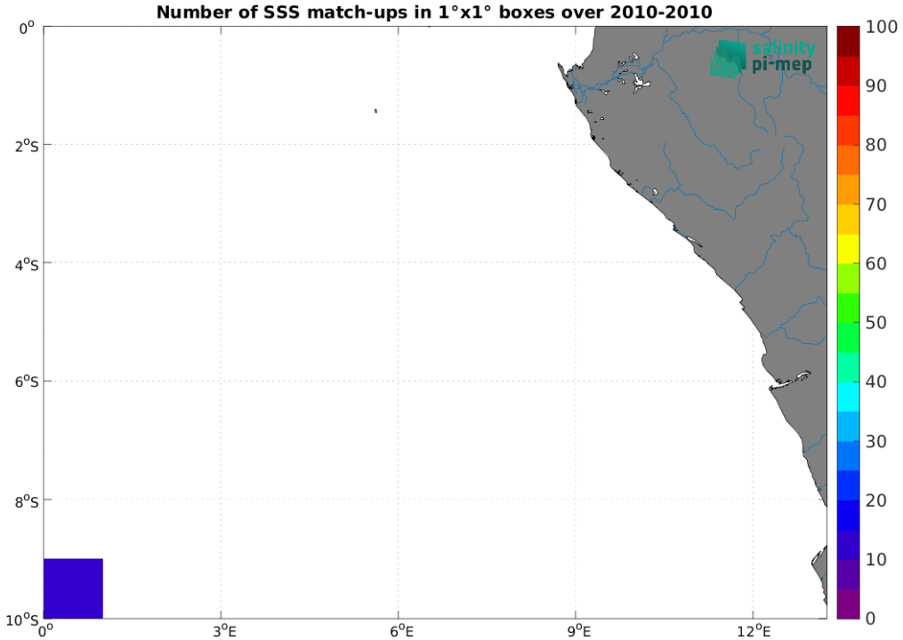
Figure 5: Number of SSS match-ups between TSG (SAMOS) SSS and the SMOS SSS L2Q v333 - 0.25 Deg (CATDS-CPDC) SSS product for the Congo river plume Pi-MEP region over 1^\circ \times 1^\circ boxes and for the full satellite product period.
