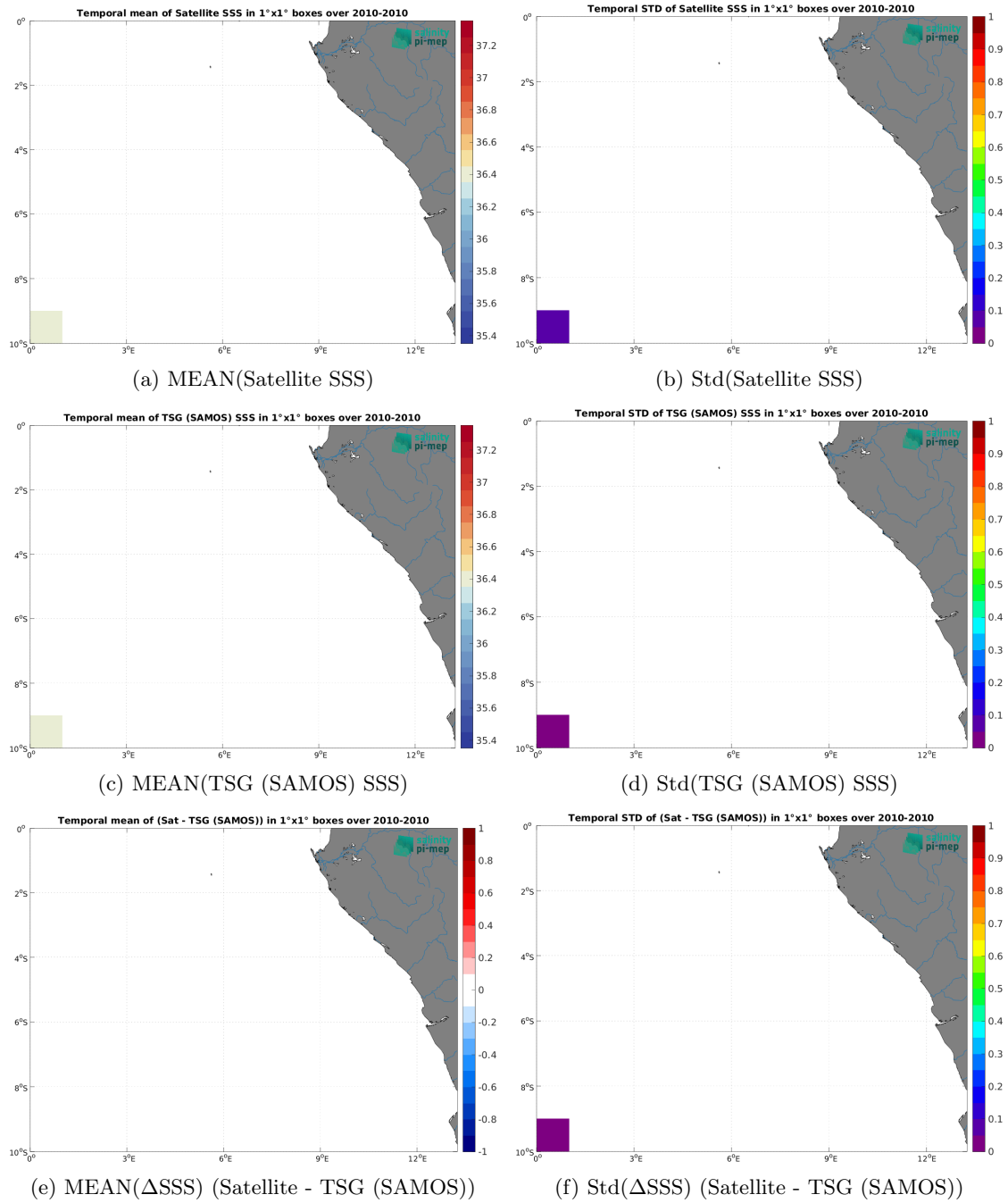
Figure 7: Temporal mean (left) and Std (right) of SSS from SMOS SSS L2Q v333 - 0.25 Deg (CATDS-CPDC) (top), TSG (SAMOS) (middle), and of \Delta SSS (Satellite - TSG (SAMOS)). Only match-up pairs are used to generate these maps.
