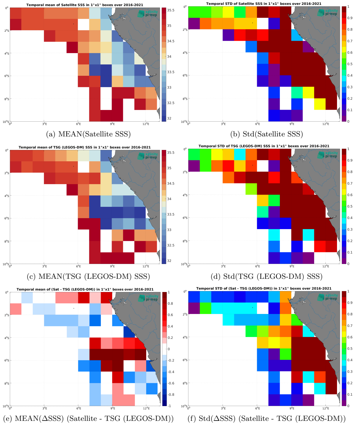
Figure 7: Temporal mean (left) and Std (right) of SSS from SMOS SSS L3 v332 - 9 Days (CATDS-CPDC) (top), TSG (LEGOS-DM) (middle), and of \Delta SSS (Satellite - TSG (LEGOS-DM)). Only match-up pairs are used to generate these maps.
