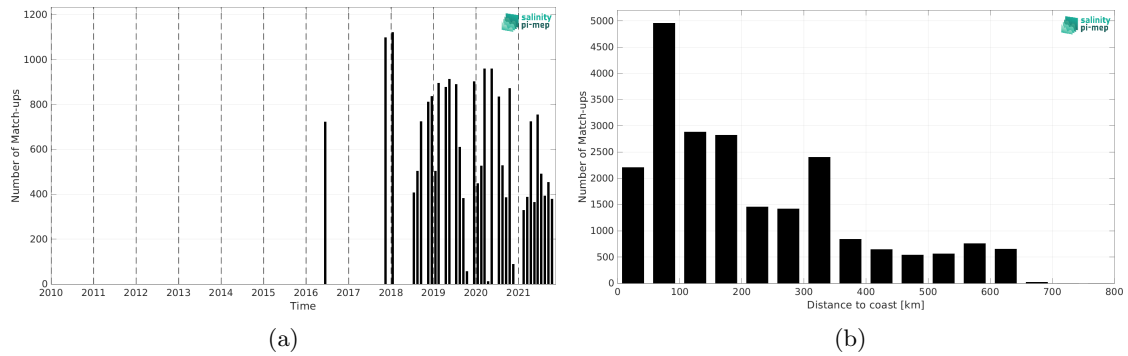
Figure 2: Number of match-ups between TSG (LEGOS-DM) and SMOS SSS L3 v332 - 9 Days (CATDS-CPDC) SSS as a function of time (a) and as function of the distance to coast (b) over the Congo river plume Pi-MEP region and for the full satellite product period.
