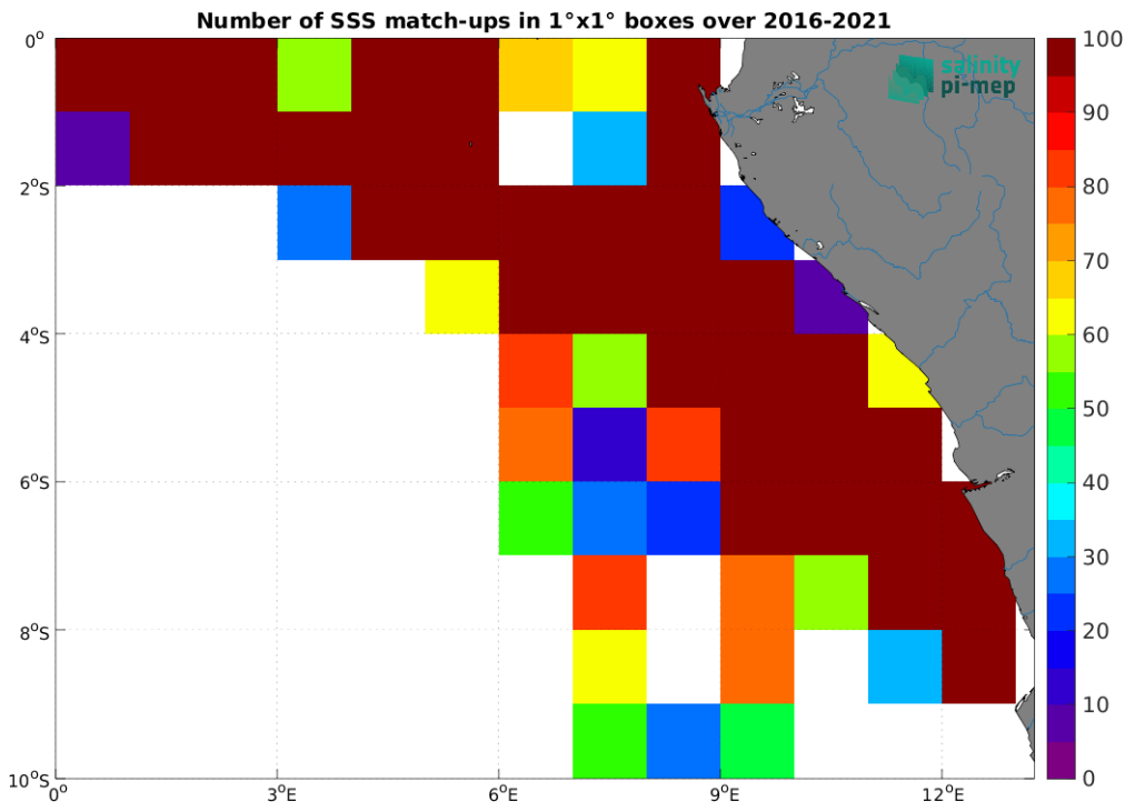
Figure 5: Number of SSS match-ups between TSG (LEGOS-DM) SSS and the SMOS SSS L3 v332 - 9 Days (CATDS-CPDC) SSS product for the Congo river plume Pi-MEP region over 1^\circ \times 1^\circ boxes and for the full satellite product period.
