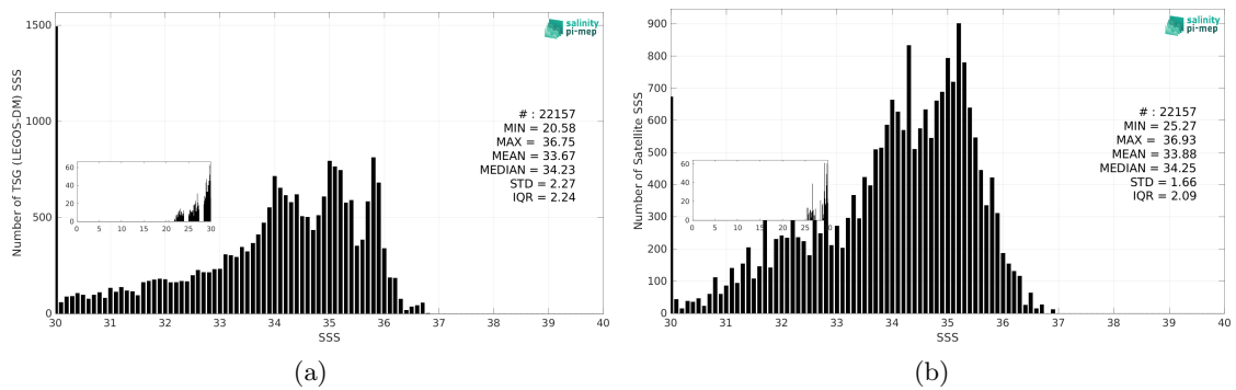
Figure 3: Histograms of SSS from TSG (LEGOS-DM) (a) and SMOS SSS L3 v332 - 9 Days (CATDS-CPDC) (b) considering all match-up pairs per bins of 0.1 over the Congo river plume Pi-MEP region and for the full satellite product period.
