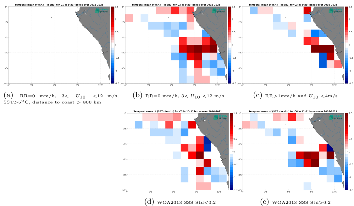
Figure 14: Temporal mean gridded over spatial boxes of size 1^\circ \times 1^\circ of \Delta SSS (SMOS SSS L3 v332 - 9 Days (CATDS-CPDC) - TSG (LEGOS-DM)) for 5 different subdatasets corresponding to:RR=0 mm/h, 3 < U_{10} < 12 m/s, SST > 5^\circ\text{C} , distance to coast > 800 km (a), RR=0 mm/h, 3 < U_{10} < 12 m/s (b), RR > 1 mm/h and U_{10} < 4 m/s (c), WOA2013 SSS Std < 0.2 (d), WOA2013 SSS Std > 0.2 (e).
