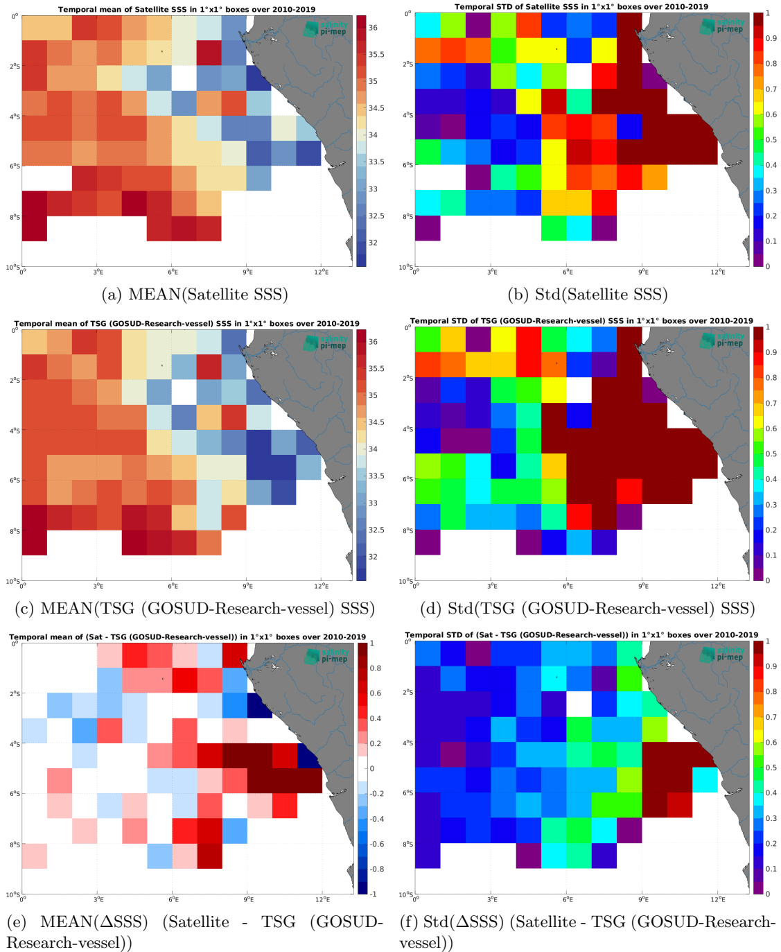
Figure 6: Temporal mean (left) and Std (right) of SSS from SMOS SSS L3 v332 - 9 Days (CATDS-CPDC) (top), TSG (GOSUD-Research-vessel) (middle), and of \Delta SSS (Satellite - TSG (GOSUD-Research-vessel)). Only match-up pairs are used to generate these maps.
