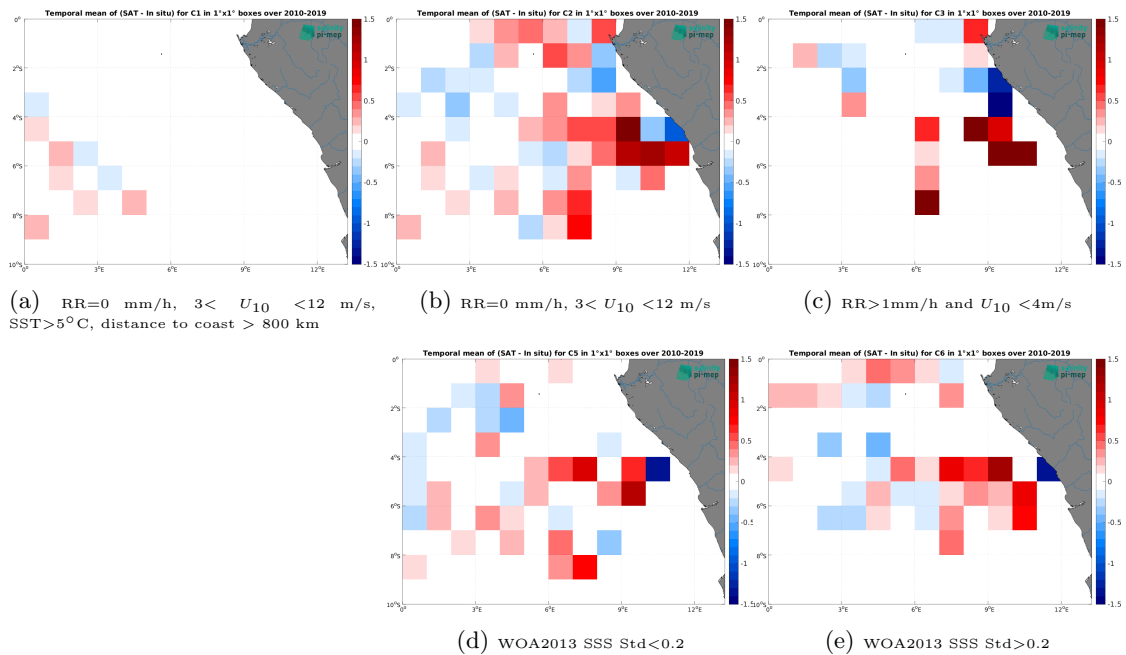
Figure 12: Temporal mean gridded over spatial boxes of size 1^\circ \times 1^\circ of \Delta SSS (SMOS SSS L3 v332 - 9 Days (CATDS-CPDC) - TSG (GOSUD-Research-vessel)) for 5 different subdatasets corresponding to:RR=0 mm/h, 3 < U_{10} < 12 m/s, SST>5°C, distance to coast > 800 km (a), RR=0 mm/h, 3 < U_{10} < 12 m/s (b), RR>1mm/h and U_{10} < 4 m/s (c), WOA2013 SSS Std<0.2 (d), WOA2013 SSS Std>0.2 (e).
