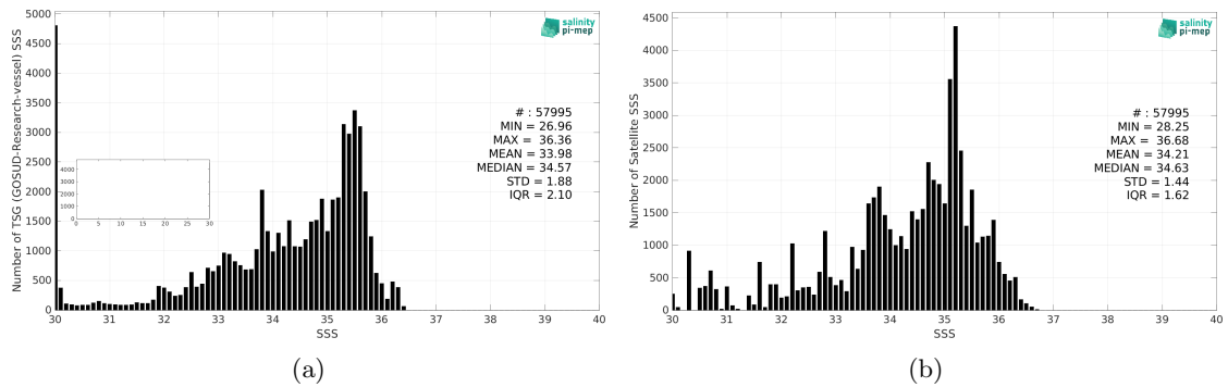
Figure 2: Histograms of SSS from TSG (GOSUD-Research-vessel) (a) and SMOS SSS L3 v332 - 9 Days (CATDS-CPDC) (b) considering all match-up pairs per bins of 0.1 over the Congo river plume Pi-MEP region and for the full satellite product period.
