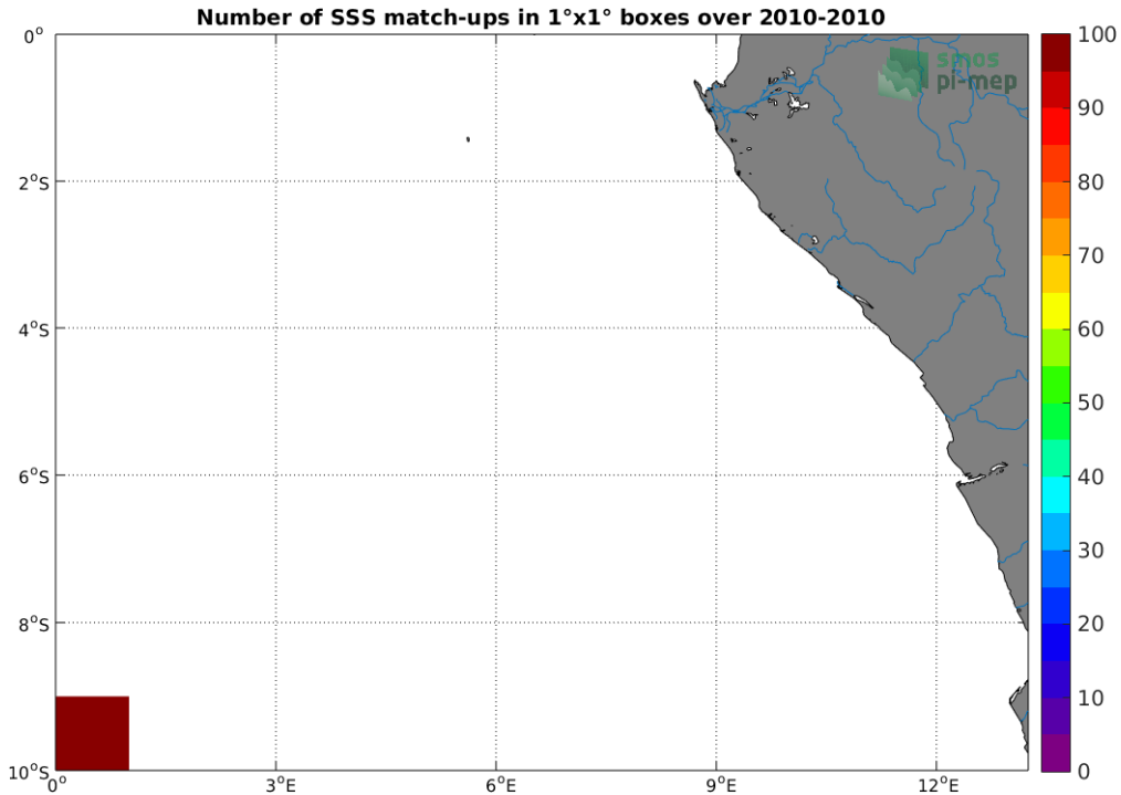
Figure 4: Number of SSS match-ups between TSG (SAMOS) SSS and the SMOS SSS L2Q v321 - 0.25 Deg (CATDS-CPDC) SSS product for the Congo river plume Pi-MEP region over 1^\circ \times 1^\circ boxes and for the full satellite product period.
