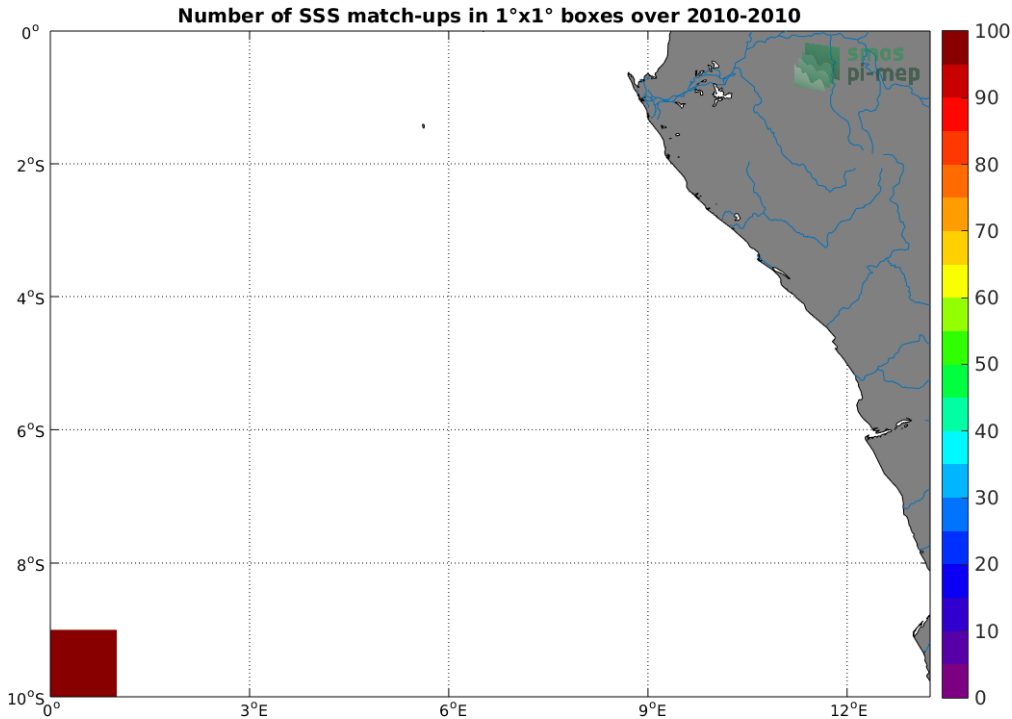
Figure 4: Number of SSS match-ups between TSG (SAMOS) SSS and the SMOS SSS L2Q v321 - 0.25 Deg (CATDS-CPDC) SSS product for the Congo river plume Pi-MEP region over 1^{\circ} \times 1^{\circ} boxes and for the full satellite product period.
