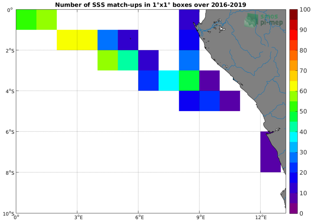
Figure 4: Number of SSS match-ups between TSG (LEGOS-DM) SSS and the SMOS SSS L2Q v321 - 0.25 Deg (CATDS-CPDC) SSS product for the Congo river plume Pi-MEP region over 1^\circ \times 1^\circ boxes and for the full satellite product period.
