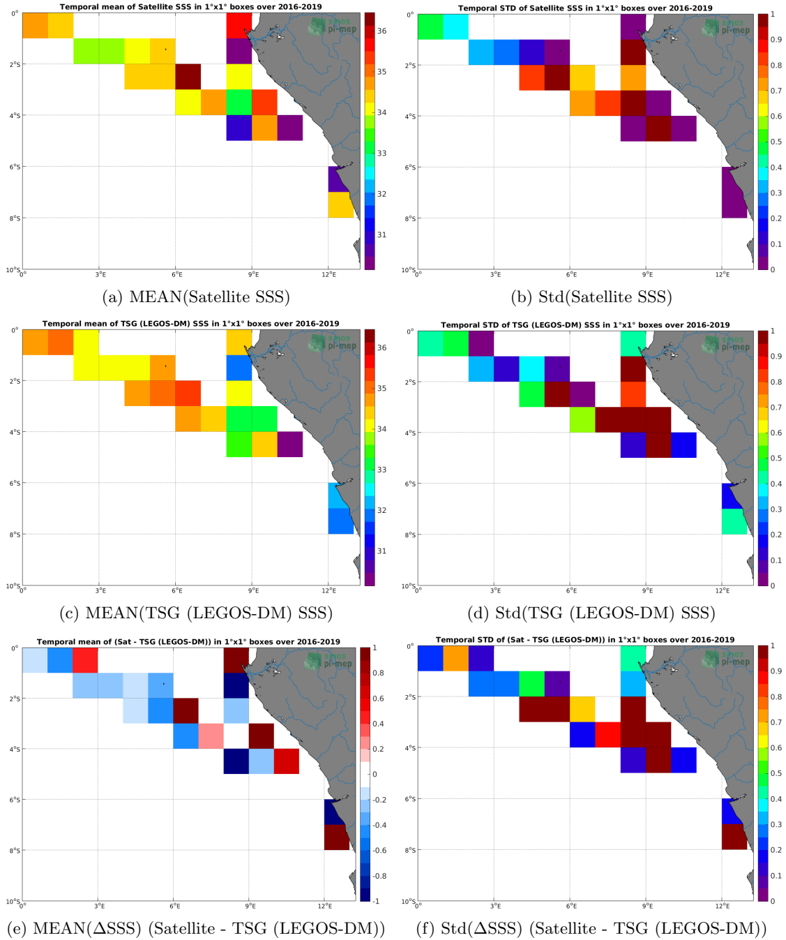
Figure 6: Temporal mean (left) and Std (right) of SSS from SMOS SSS L2Q v321 - 0.25 Deg (CATDS-CPDC) (top), TSG (LEGOS-DM) (middle), and of \Delta SSS (Satellite - TSG (LEGOS-DM)). Only match-up pairs are used to generate these maps.
