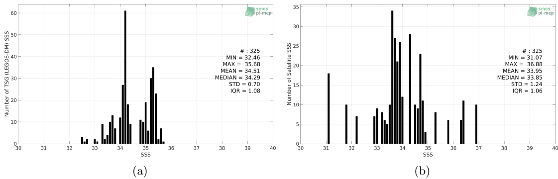
Figure 2: Histograms of SSS from TSG (LEGOS-DM) (a) and SMOS SSS L2Q v321 - 0.25 Deg (CATDS-CPDC) (b) considering all match-up pairs per bins of 0.1 over the Congo river plume Pi-MEP region and for the full satellite product period.
