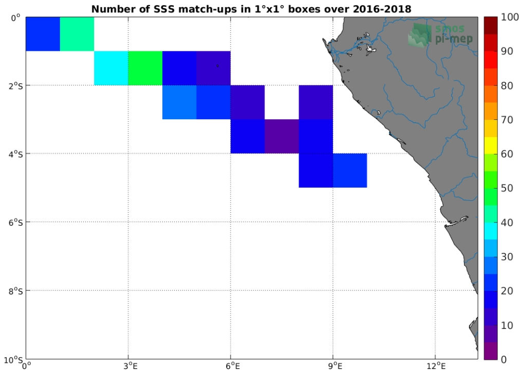
Figure 4: Number of SSS match-ups between TSG (LEGOS-DM) SSS and the SMOS SSS L2Q v321 - 0.25 Deg (CATDS-CPDC) SSS product for the Congo river plume Pi-MEP region over 1°x1° boxes and for the full satellite product period.
