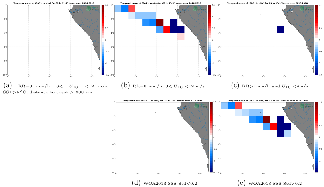
Figure 12: Temporal mean gridded over spatial boxes of size 1^{\circ}\times 1^{\circ} of \Delta\text{SSS} (SMOS SSS L2Q v321 - 0.25 Deg (CATDS-CPDC) - TSG (LEGOS-DM)) for 5 different subdatasets corresponding to:RR=0 mm/h, 3 < U_{10} < 12 m/s, SST > 5^{\circ}\text{C} , distance to coast > 800 km (a), RR=0 mm/h, 3 < U_{10} < 12 m/s (b), RR > 1 mm/h and U_{10} < 4 m/s (c), WOA2013 SSS Std < 0.2 (d), WOA2013 SSS Std > 0.2 (e).
