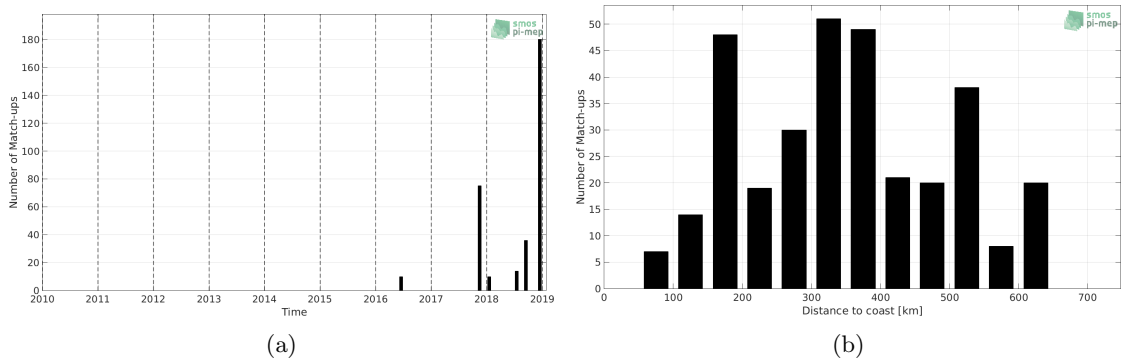
Figure 1: Number of match-ups between TSG (LEGOS-DM) and SMOS SSS L2Q v321 - 0.25 Deg (CATDS-CPDC) SSS as a function of time (a) and as function of the distance to coast (b) over the Congo river plume Pi-MEP region and for the full satellite product period.
