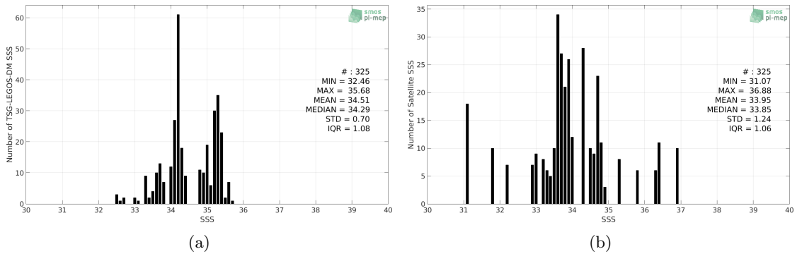
Figure 2: Histograms of SSS from TSG-LEGOS-DM (a) and SMOS L2Q v321 - 0.25 Deg (CATDS-CPDC) (b) considering all match-up pairs per bins of 0.1 over the Congo river plume Pi-MEP region and for the full satellite product period.
