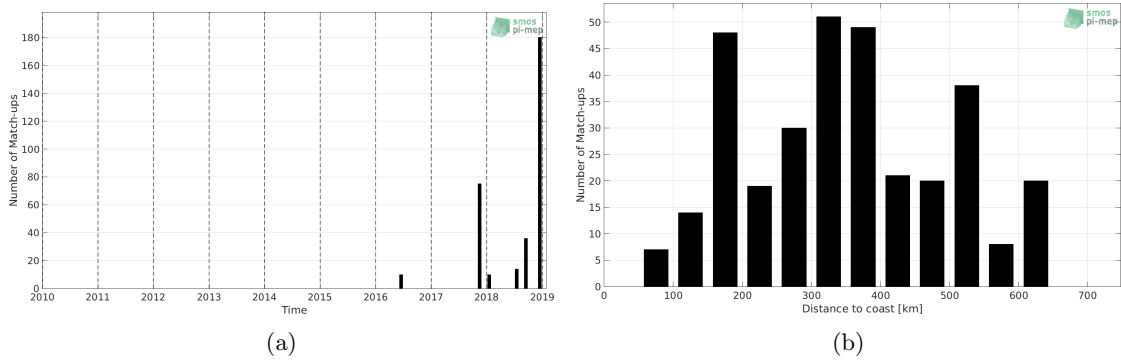
Figure 1: Number of match-ups between TSG-LEGOS-DM and SMOS L2Q v321 - 0.25 Deg (CATDS-CPDC) SSS as a function of time (a) and as function of the distance to coast (b) over the Congo river plume Pi-MEP region and for the full satellite product period.
