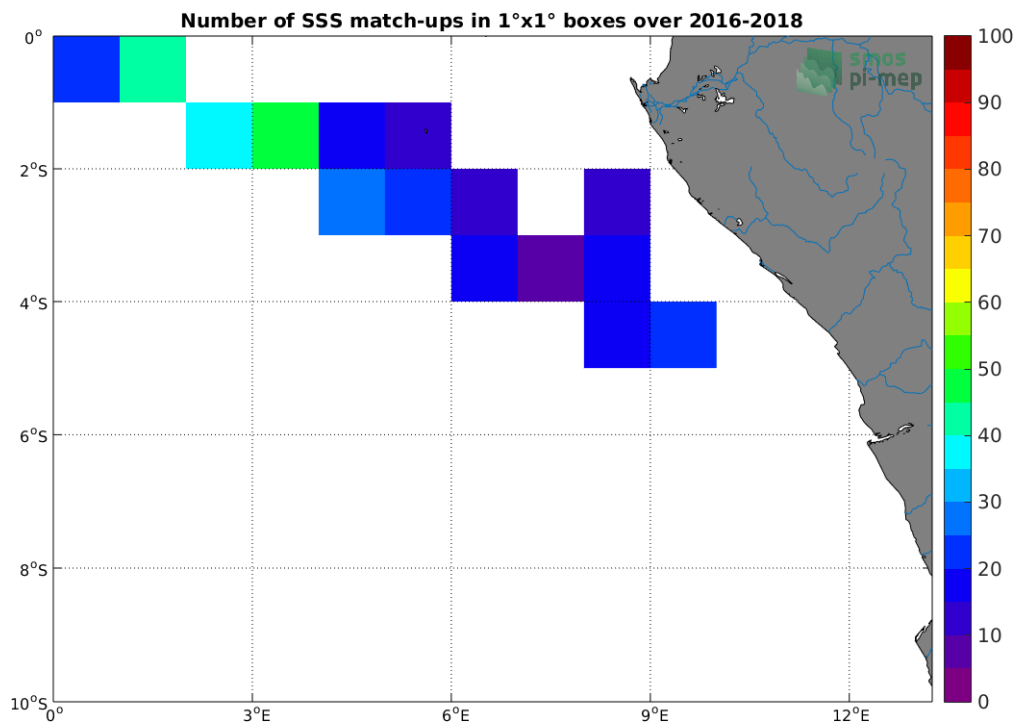
Figure 4: Number of SSS match-ups between TSG-LEGOS-DM SSS and the SMOS L2Q v321 - 0.25 Deg (CATDS-CPDC) SSS product for the Congo river plume Pi-MEP region over 1°x1° boxes and for the full satellite product period.
