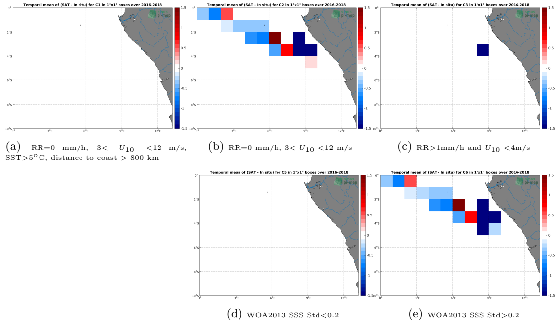
Figure 12: Temporal mean gridded over spatial boxes of size 1^\circ \times 1^\circ of \Delta SSS (SMOS L2Q v321 - 0.25 Deg (CATDS-CPDC) - TSG-LEGOS-DM) for 5 different subdatasets corresponding to:RR=0 mm/h, 3 < U_{10} < 12 m/s, SST > 5^\circ\text{C} , distance to coast > 800 km (a), RR=0 mm/h, 3 < U_{10} < 12 m/s (b), RR > 1 mm/h and U_{10} < 4 m/s (c), WOA2013 SSS Std < 0.2 (d), WOA2013 SSS Std > 0.2 (e).
