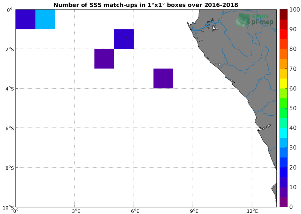
Figure 4: Number of SSS match-ups between TSG-LEGOS-DM SSS and the SMOS-L3-CATDS-CPDC-V321-L2Q SSS product for the Congo river plume Pi-MEP region over 1°x1° boxes and for the full satellite product period.
