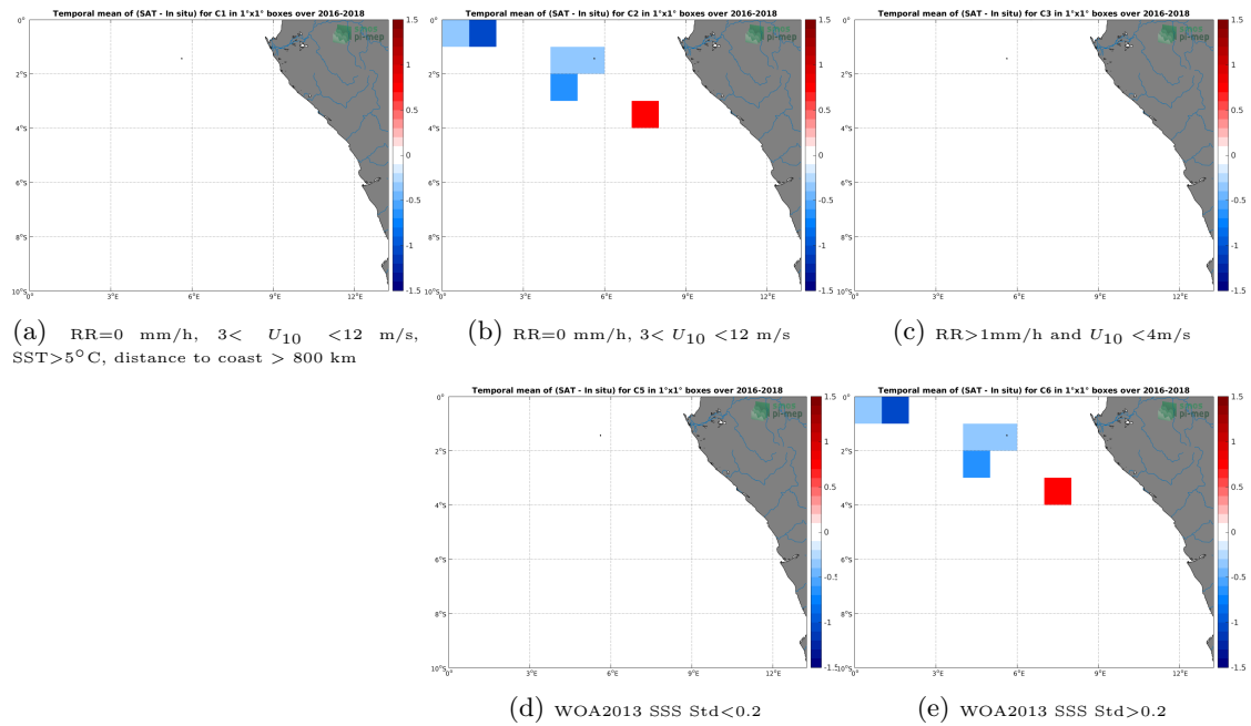
Figure 12: Temporal mean gridded over spatial boxes of size 1^\circ \times 1^\circ of \Delta SSS (SMOS-L3-CATDS-CPDC-V321-L2Q - TSG-LEGOS-DM) for 5 different subdatasets corresponding to:RR=0 mm/h, 3 < U_{10} < 12 m/s, SST > 5^\circ\text{C} , distance to coast > 800 km (a), RR=0 mm/h, 3 < U_{10} < 12 m/s (b), RR > 1 mm/h and U_{10} < 4 m/s (c), WOA2013 SSS Std < 0.2 (d), WOA2013 SSS Std > 0.2 (e).
