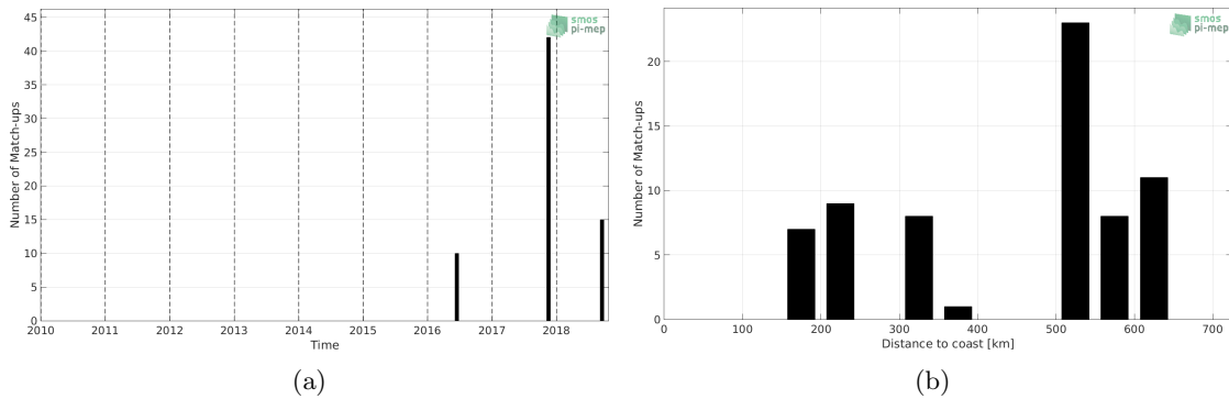
Figure 1: Number of match-ups between TSG-LEGOS-DM and SMOS-L3-CATDS-CPDC-V321-L2Q SSS as a function of time (a) and as function of the distance to coast (b) over the Congo river plume Pi-MEP region and for the full satellite product period.
