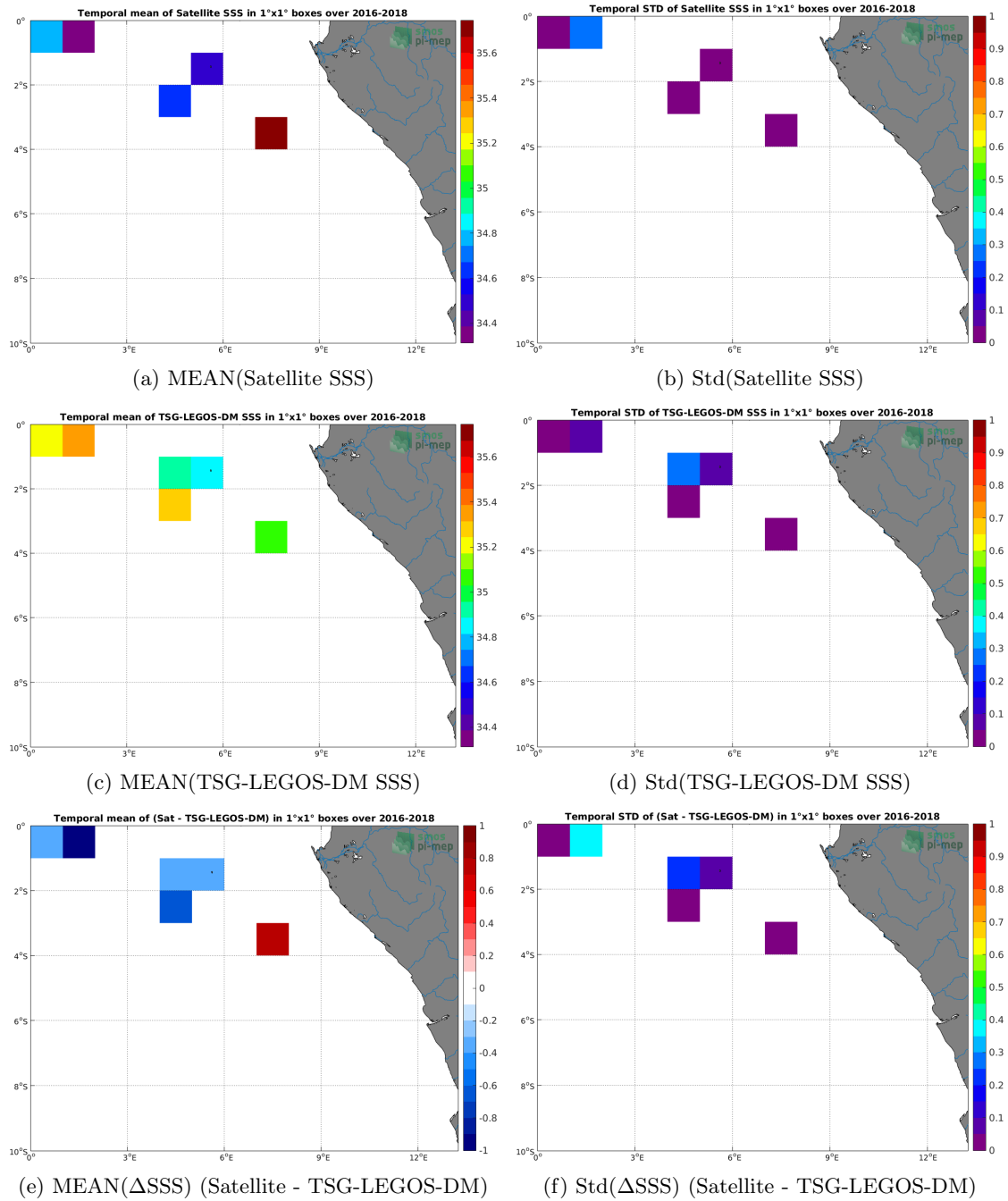
Figure 6: Temporal mean (left) and Std (right) of SSS from SMOS-L3-CATDS-CPDC-V321-L2Q (top), TSG-LEGOS-DM (middle), and of \Delta SSS (Satellite - TSG-LEGOS-DM). Only match-up pairs are used to generate these maps.
