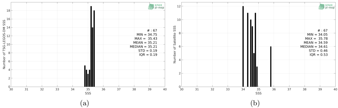
Figure 2: Histograms of SSS from TSG-LEGOS-DM (a) and SMOS-L3-CATDS-CPDC-V321-L2Q (b) considering all match-up pairs per bins of 0.1 over the Congo river plume Pi-MEP region and for the full satellite product period.
