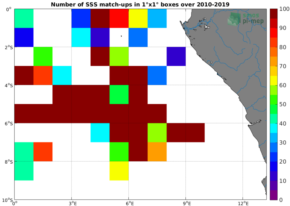
Figure 4: Number of SSS match-ups between TSG (GOSUD-Research-vessel) SSS and the SMOS SSS L2Q v321 - 0.25 Deg (CATDS-CPDC) SSS product for the Congo river plume Pi-MEP region over 1^\circ \times 1^\circ boxes and for the full satellite product period.
