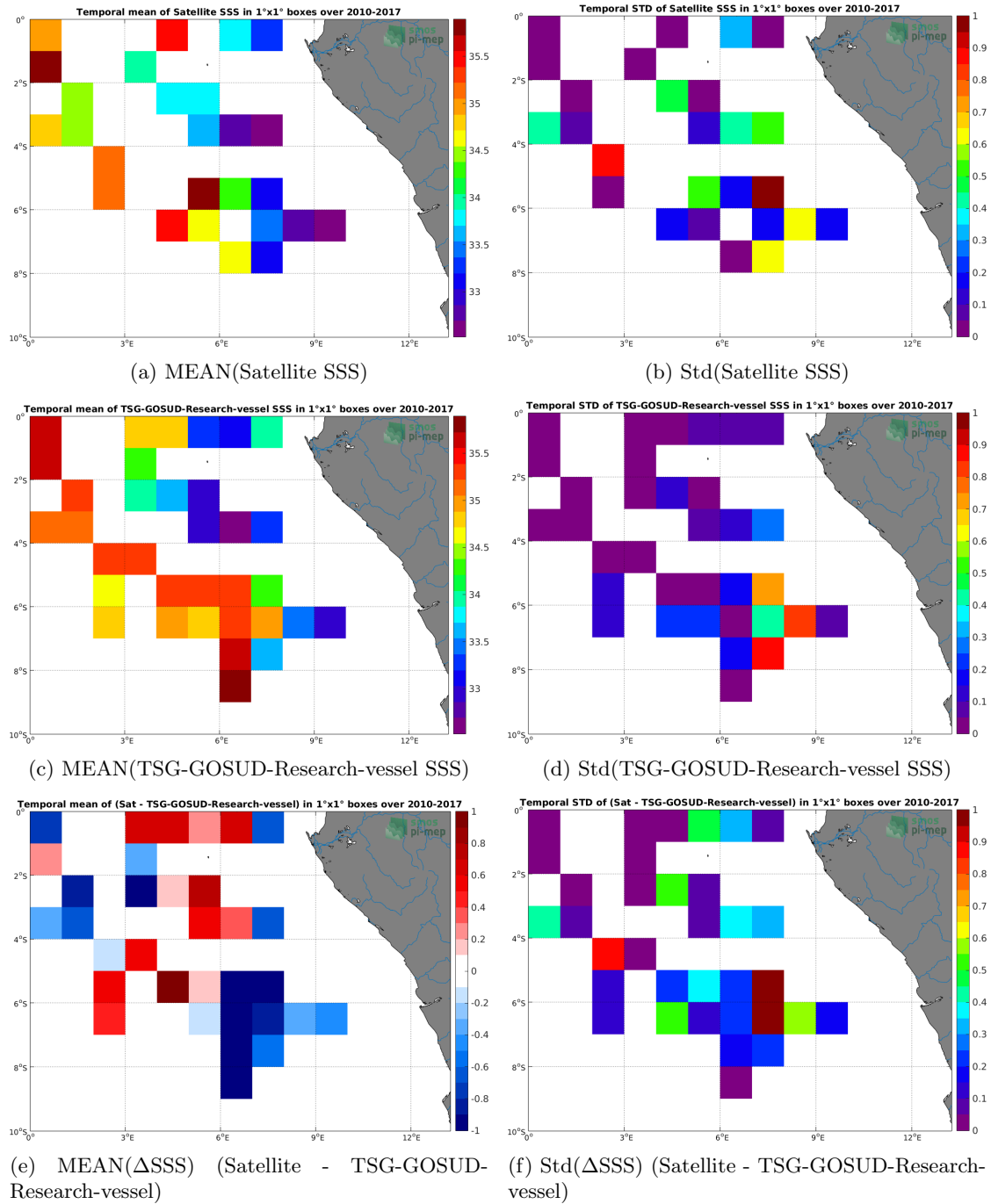
Figure 6: Temporal mean (left) and Std (right) of SSS from SMOS-L3-CATDS-CPDC-V321-L2Q (top), TSG-GOSUD-Research-vessel (middle), and of \Delta SSS (Satellite - TSG-GOSUD-Research-vessel). Only match-up pairs are used to generate these maps.
