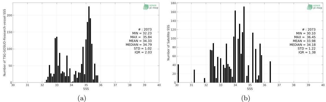
Figure 2: Histograms of SSS from TSG-GOSUD-Research-vessel (a) and SMOS-L3-CATDS-CPDC-V321-L2Q (b) considering all match-up pairs per bins of 0.1 over the Congo river plume Pi-MEP region and for the full satellite product period.
