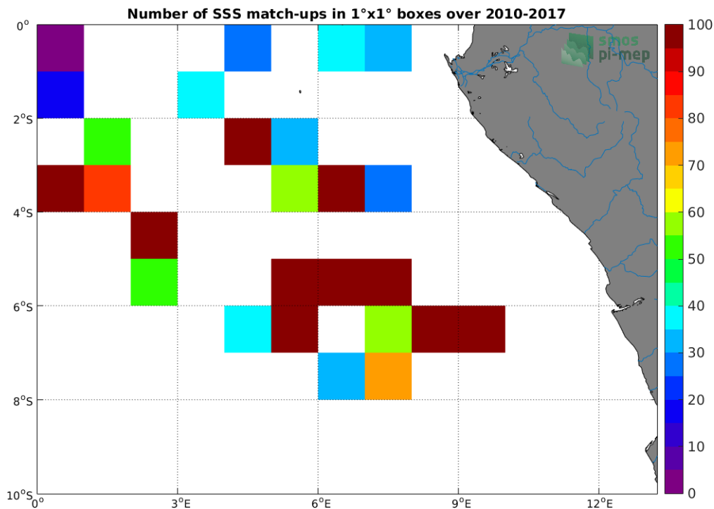
Figure 4: Number of SSS match-ups between TSG-GOSUD-Research-vessel SSS and the SMOS-L3-CATDS-CPDC-V321-L2Q SSS product for the Congo river plume Pi-MEP region over 1°x1° boxes and for the full satellite product period.
