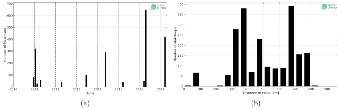
Figure 1: Number of match-ups between TSG-GOSUD-Research-vessel and SMOS-L3-CATDS-CPDC-V321-L2Q SSS as a function of time (a) and as function of the distance to coast (b) over the Congo river plume Pi-MEP region and for the full satellite product period.
