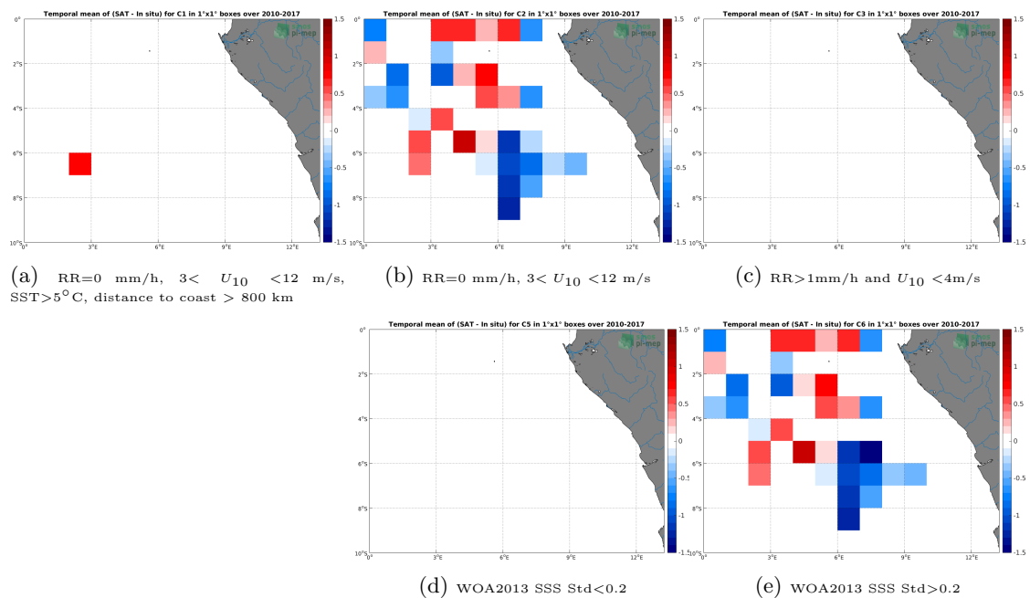
Figure 12: Temporal mean gridded over spatial boxes of size 1^\circ \times 1^\circ of \Delta SSS (SMOS-L3-CATDS-CPDC-V321-L2Q - TSG-GOSUD-Research-vessel) for 5 different subdatasets corresponding to:RR=0 mm/h, 3 < U_{10} < 12 m/s, SST > 5^\circ\text{C} , distance to coast > 800 km (a), RR=0 mm/h, 3 < U_{10} < 12 m/s (b), RR > 1 mm/h and U_{10} < 4 m/s (c), WOA2013 SSS Std < 0.2 (d), WOA2013 SSS Std > 0.2 (e).
