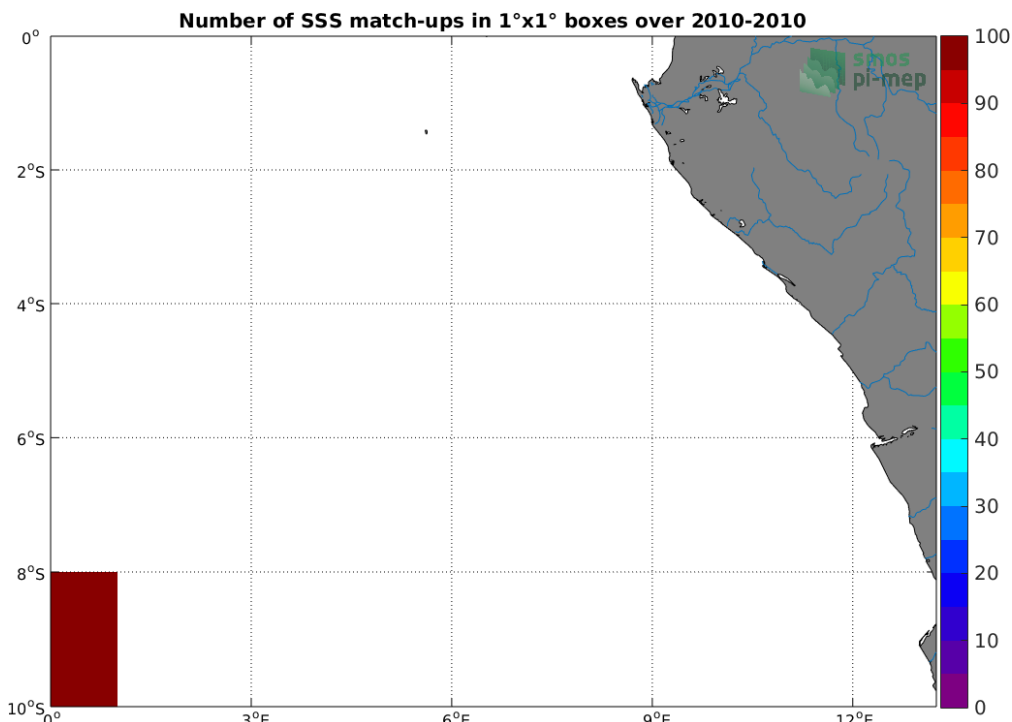
Figure 4: Number of SSS match-ups between TSG (SAMOS) SSS and the SMOS SSS L3 v317 - Monthly - 25 km (CATDS-CPDC) SSS product for the Congo river plume Pi-MEP region over 1^\circ \times 1^\circ boxes and for the full satellite product period.
