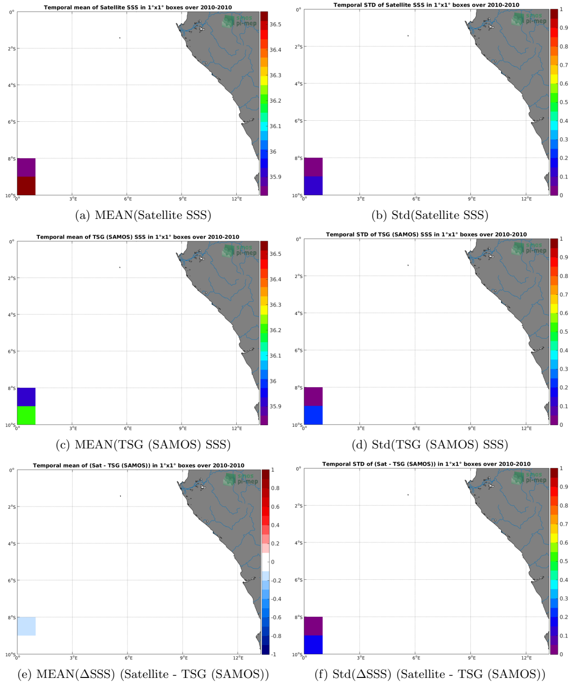
Figure 6: Temporal mean (left) and Std (right) of SSS from SMOS SSS L3 v317 - Monthly - 25 km (CATDS-CPDC) (top), TSG (SAMOS) (middle), and of \Delta SSS (Satellite - TSG (SAMOS)). Only match-up pairs are used to generate these maps.
