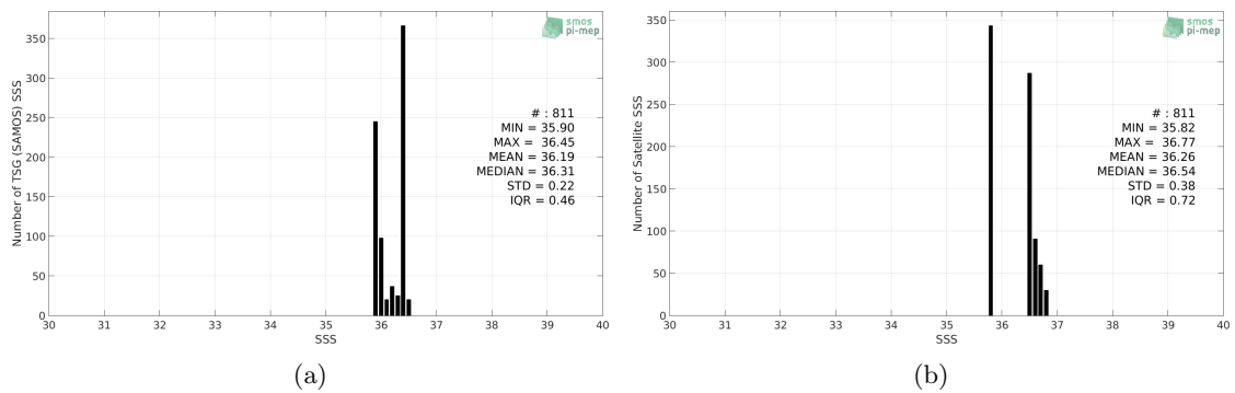
Figure 2: Histograms of SSS from TSG (SAMOS) (a) and SMOS SSS L3 v317 - Monthly - 25 km (CATDS-CPDC) (b) considering all match-up pairs per bins of 0.1 over the Congo river plume Pi-MEP region and for the full satellite product period.
