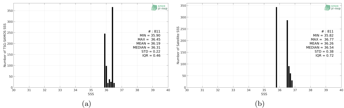
Figure 2: Histograms of SSS from TSG-SAMOS (a) and SMOS L3 v317 - Monthly - 25 km (CATDS-CPDC) (b) considering all match-up pairs per bins of 0.1 over the Congo river plume Pi-MEP region and for the full satellite product period.
