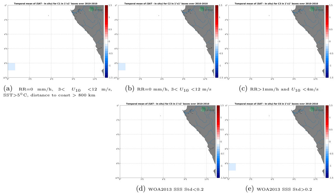
Figure 12: Temporal mean gridded over spatial boxes of size 1^\circ \times 1^\circ of \Delta SSS (SMOS L3 v317 - Monthly - 25 km (CATDS-CPDC) - TSG-SAMOS) for 5 different subdatasets corresponding to:RR=0 mm/h, 3 < U_{10} < 12 m/s, SST > 5^\circ\text{C} , distance to coast > 800 km (a), RR=0 mm/h, 3 < U_{10} < 12 m/s (b), RR > 1 mm/h and U_{10} < 4 m/s (c), WOA2013 SSS Std < 0.2 (d), WOA2013 SSS Std > 0.2 (e).
