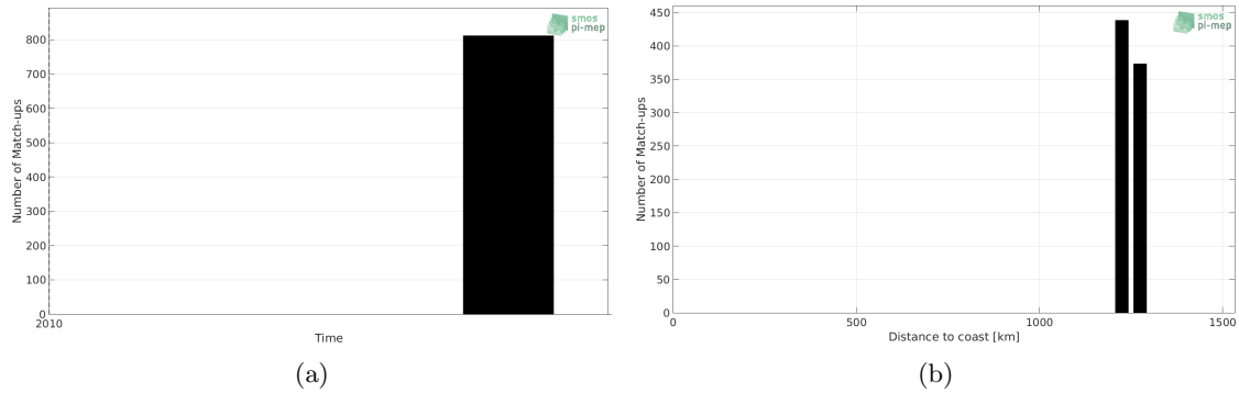
Figure 1: Number of match-ups between TSG-SAMOS and SMOS L3 v317 - Monthly - 25 km (CATDS-CPDC) SSS as a function of time (a) and as function of the distance to coast (b) over the Congo river plume Pi-MEP region and for the full satellite product period.
