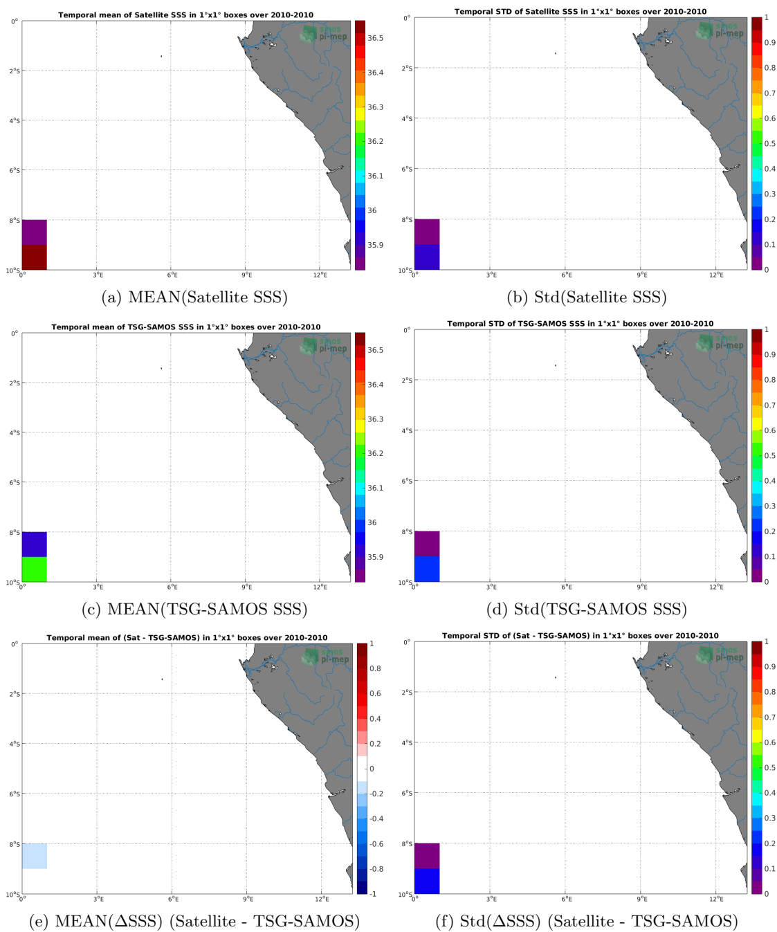
Figure 6: Temporal mean (left) and Std (right) of SSS from SMOS L3 v317 - Monthly - 25 km (CATDS-CPDC) (top), TSG-SAMOS (middle), and of \Delta SSS (Satellite - TSG-SAMOS). Only match-up pairs are used to generate these maps.
