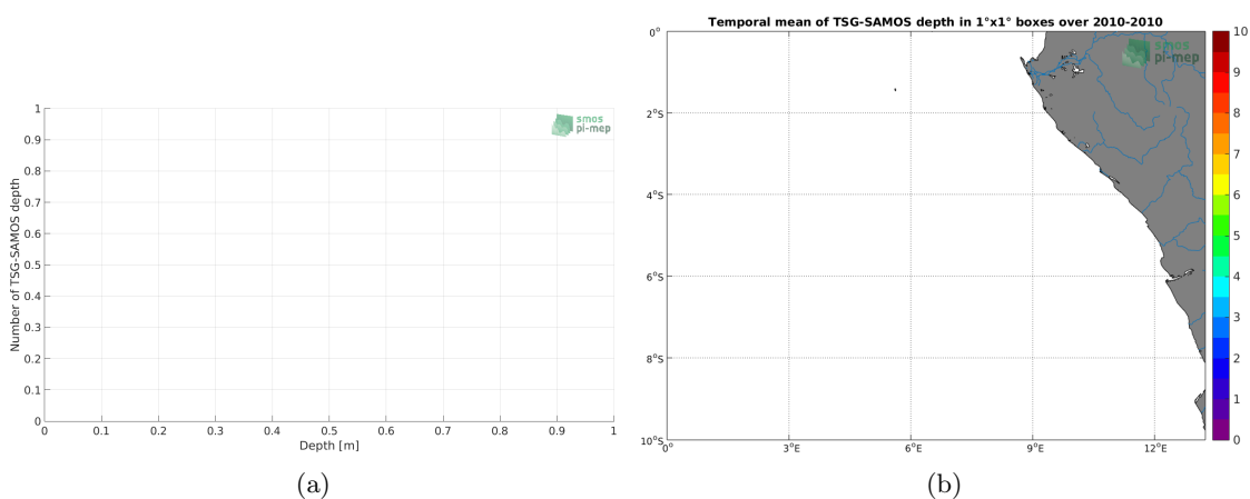
Figure 3: Histograms of the depth of the upper level SSS measurements from TSG-SAMOS in the Match-up DataBase for the Congo river plume Pi-MEP region (a) and temporal mean spatial distribution of pressure of the in situ SSS data over 1^\circ \times 1^\circ boxes and for the full satellite product period (b).
