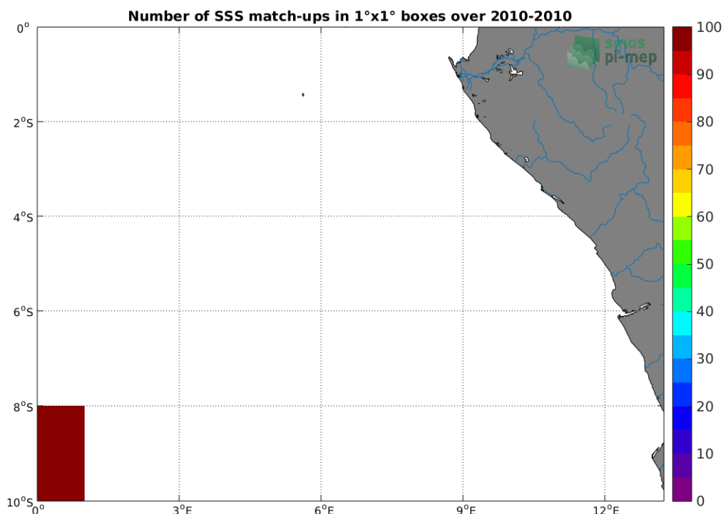
Figure 4: Number of SSS match-ups between TSG-SAMOS SSS and the SMOS L3 v317 - Monthly - 25 km (CATDS-CPDC) SSS product for the Congo river plume Pi-MEP region over 1^\circ \times 1^\circ boxes and for the full satellite product period.
