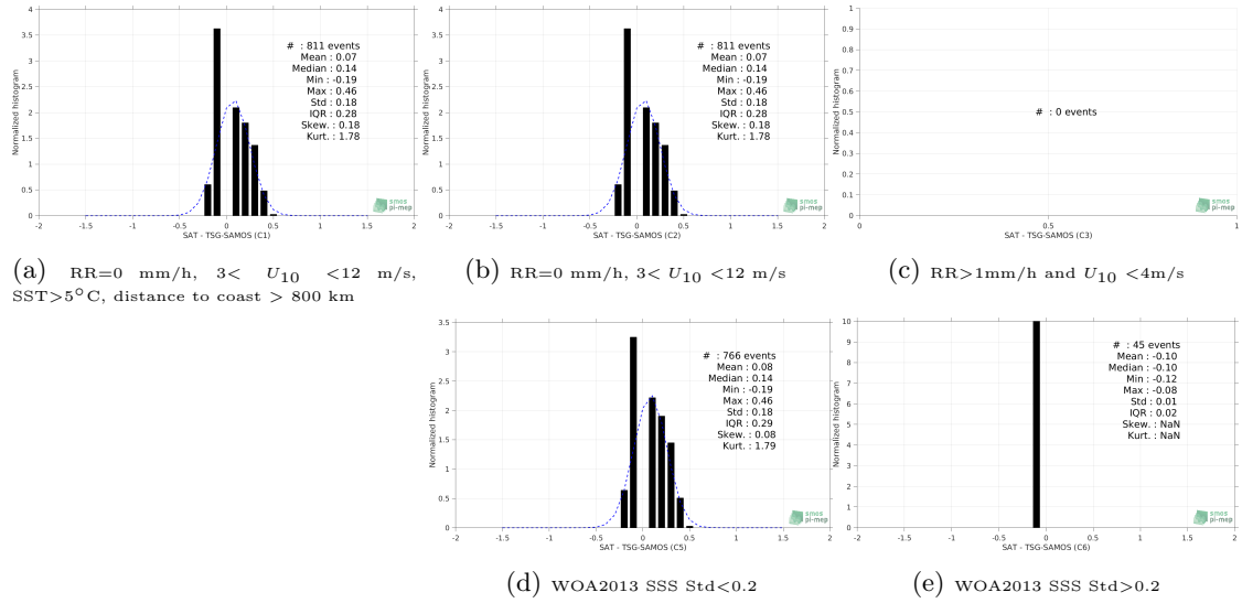
Figure 13: Normalized histogram of \Delta SSS (SMOS-L3-CATDS-CPDC-V317-MONTHLY-25KM - TSG-SAMOS) for 5 different subdatasets corresponding to: RR=0 mm/h, 3 < U_{10} < 12 m/s, SST > 5°C, distance to coast > 800 km (a), RR=0 mm/h, 3 < U_{10} < 12 m/s (b), RR > 1mm/h and U_{10} < 4 m/s (c), WOA2013 SSS Std < 0.2 (d), WOA2013 SSS Std > 0.2 (e).
