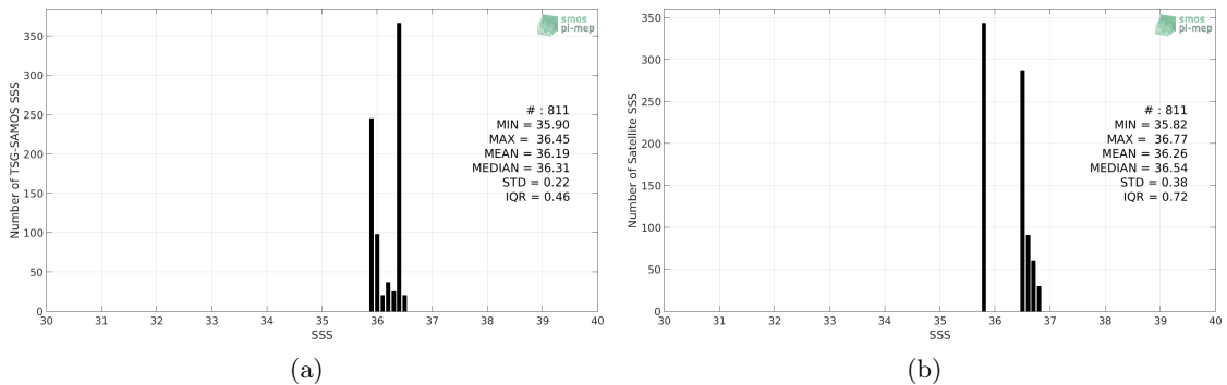
Figure 2: Histograms of SSS from TSG-SAMOS (a) and SMOS-L3-CATDS-CPDC-V317-MONTHLY-25KM (b) considering all match-up pairs per bins of 0.1 over the Congo river plume Pi-MEP region and for the full satellite product period.
