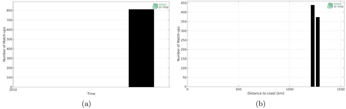
Figure 1: Number of match-ups between TSG-SAMOS and SMOS-L3-CATDS-CPDC-V317-MONTHLY-25KM SSS as a function of time (a) and as function of the distance to coast (b) over the Congo river plume Pi-MEP region and for the full satellite product period.
