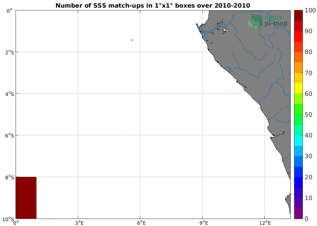
Figure 4: Number of SSS match-ups between TSG-SAMOS SSS and the SMOS-L3-CATDS-CPDC-V317-MONTHLY-25KM SSS product for the Congo river plume Pi-MEP region over 1^\circ \times 1^\circ boxes and for the full satellite product period.
