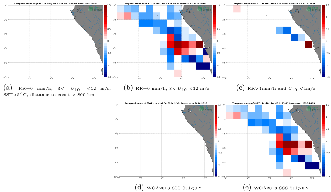
Figure 12: Temporal mean gridded over spatial boxes of size 1^\circ \times 1^\circ of \Delta SSS (SMOS L3 v317 - Monthly - 25 km (CATDS-CPDC) - TSG-LEGOS-DM) for 5 different subdatasets corresponding to:RR=0 mm/h, 3 < U_{10} < 12 m/s, SST > 5^\circ\text{C} , distance to coast > 800 km (a), RR=0 mm/h, 3 < U_{10} < 12 m/s (b), RR > 1 mm/h and U_{10} < 4 m/s (c), WOA2013 SSS Std < 0.2 (d), WOA2013 SSS Std > 0.2 (e).
