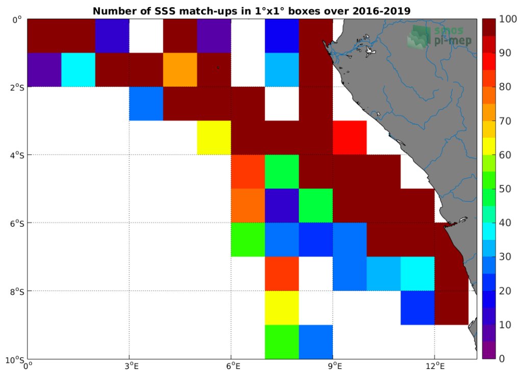
Figure 4: Number of SSS match-ups between TSG-LEGOS-DM SSS and the SMOS L3 v317 - Monthly - 25 km (CATDS-CPDC) SSS product for the Congo river plume Pi-MEP region over 1°x1° boxes and for the full satellite product period.
