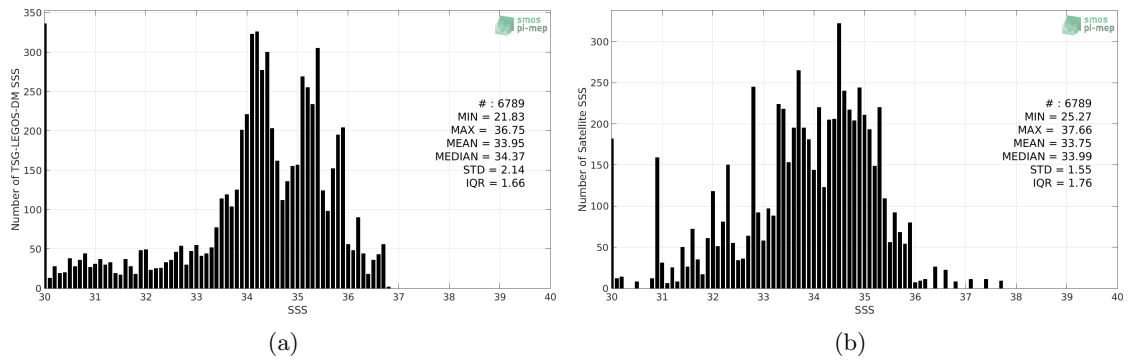
Figure 2: Histograms of SSS from TSG-LEGOS-DM (a) and SMOS L3 v317 - Monthly - 25 km (CATDS-CPDC) (b) considering all match-up pairs per bins of 0.1 over the Congo river plume Pi-MEP region and for the full satellite product period.
