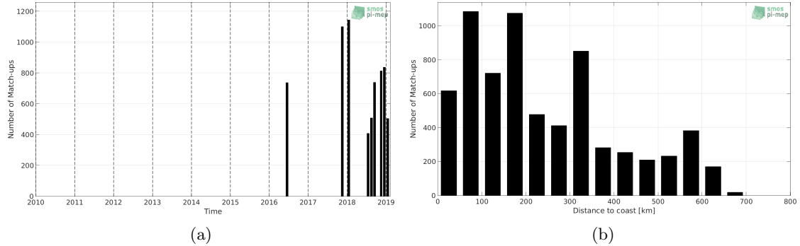
Figure 1: Number of match-ups between TSG-LEGOS-DM and SMOS L3 v317 - Monthly - 25 km (CATDS-CPDC) SSS as a function of time (a) and as function of the distance to coast (b) over the Congo river plume Pi-MEP region and for the full satellite product period.
