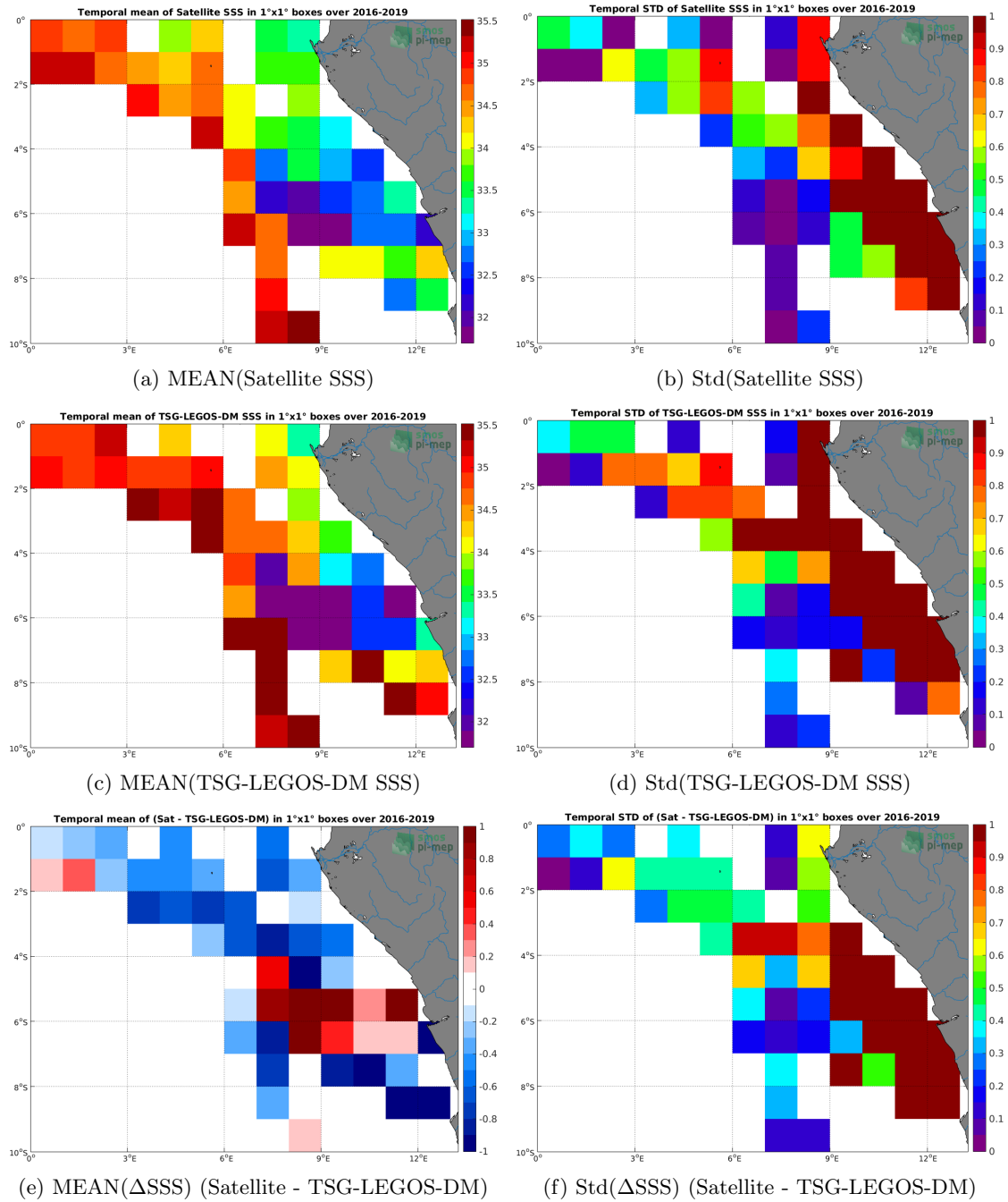
Figure 6: Temporal mean (left) and Std (right) of SSS from SMOS L3 v317 - Monthly - 25 km (CATDS-CPDC) (top), TSG-LEGOS-DM (middle), and of \Delta SSS (Satellite - TSG-LEGOS-DM). Only match-up pairs are used to generate these maps.
