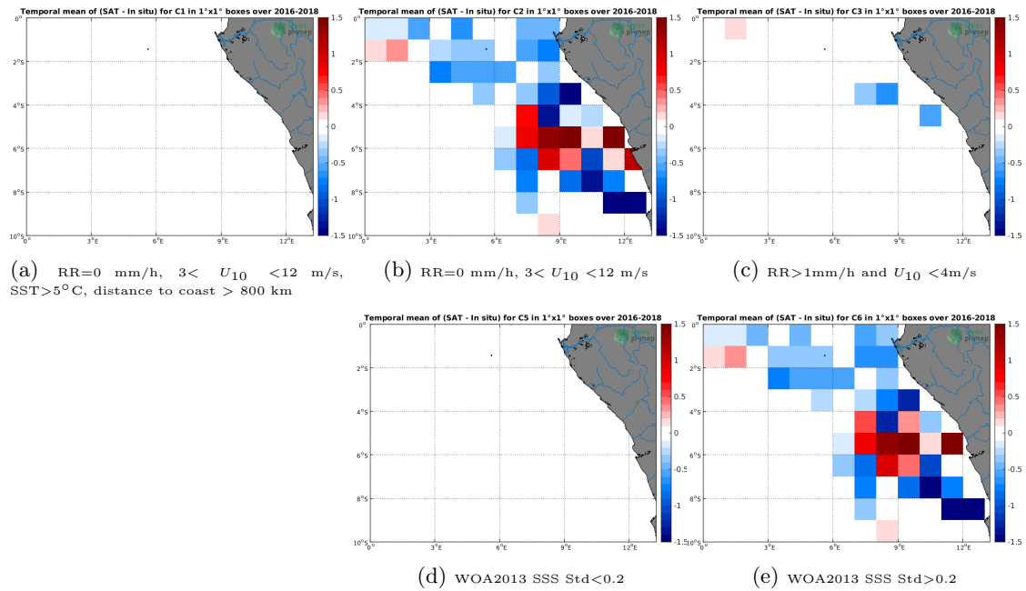
Figure 12: Temporal mean gridded over spatial boxes of size 1^\circ \times 1^\circ of \Delta SSS (SMOS-L3-CATDS-CPDC-V317-MONTHLY-25KM - TSG-LEGOS-DM) for 5 different subdatasets corresponding to:RR=0 mm/h, 3 < U_{10} < 12 m/s, SST >5^\circ C, distance to coast > 800 km (a), RR=0 mm/h, 3 < U_{10} < 12 m/s (b), RR >1 mm/h and U_{10} < 4 m/s (c), WOA2013 SSS Std <0.2 (d), WOA2013 SSS Std >0.2 (e).
