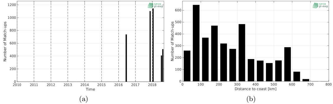
Figure 1: Number of match-ups between TSG-LEGOS-DM and SMOS-L3-CATDS-CPDC-V317-MONTHLY-25KM SSS as a function of time (a) and as function of the distance to coast (b) over the Congo river plume Pi-MEP region and for the full satellite product period.
