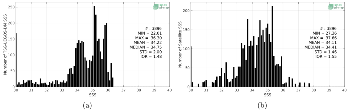
Figure 2: Histograms of SSS from TSG-LEGOS-DM (a) and SMOS-L3-CATDS-CPDC-V317-MONTHLY-25KM (b) considering all match-up pairs per bins of 0.1 over the Congo river plume Pi-MEP region and for the full satellite product period.
