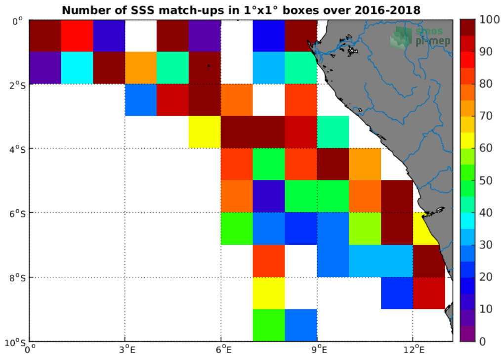
Figure 4: Number of SSS match-ups between TSG-LEGOS-DM SSS and the SMOS-L3-CATDS-CPDC-V317-MONTHLY-25KM SSS product for the Congo river plume Pi-MEP region over 1°x1° boxes and for the full satellite product period.
