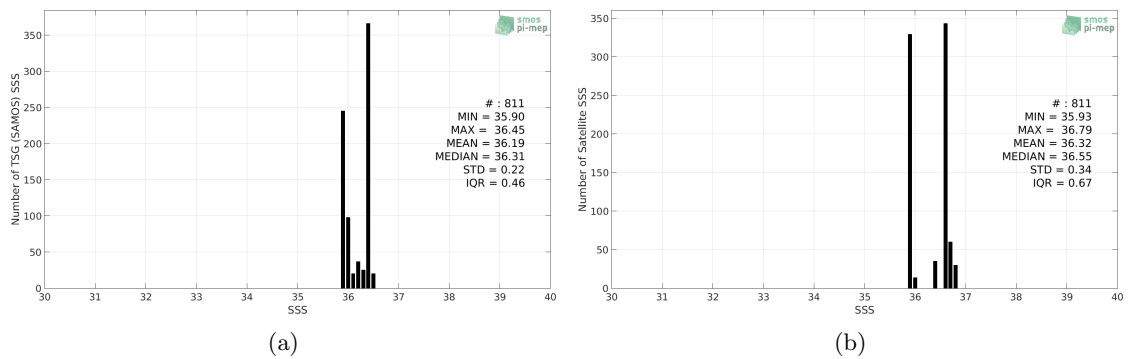
Figure 2: Histograms of SSS from TSG (SAMOS) (a) and SMOS SSS L3 v317 - 10 Days - 25 km (CATDS-CPDC) (b) considering all match-up pairs per bins of 0.1 over the Congo river plume Pi-MEP region and for the full satellite product period.
