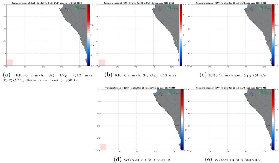
Figure 12: Temporal mean gridded over spatial boxes of size 1^\circ \times 1^\circ of \Delta SSS (SMOS SSS L3 v317 - 10 Days - 25 km (CATDS-CPDC) - TSG (SAMOS)) for 5 different subdatasets corresponding to:RR=0 mm/h, 3 < U_{10} < 12 m/s, SST >5^\circ\text{C} , distance to coast > 800 km (a), RR=0 mm/h, 3 < U_{10} < 12 m/s (b), RR >1 mm/h and U_{10} < 4 m/s (c), WOA2013 SSS Std <0.2 (d), WOA2013 SSS Std >0.2 (e).
