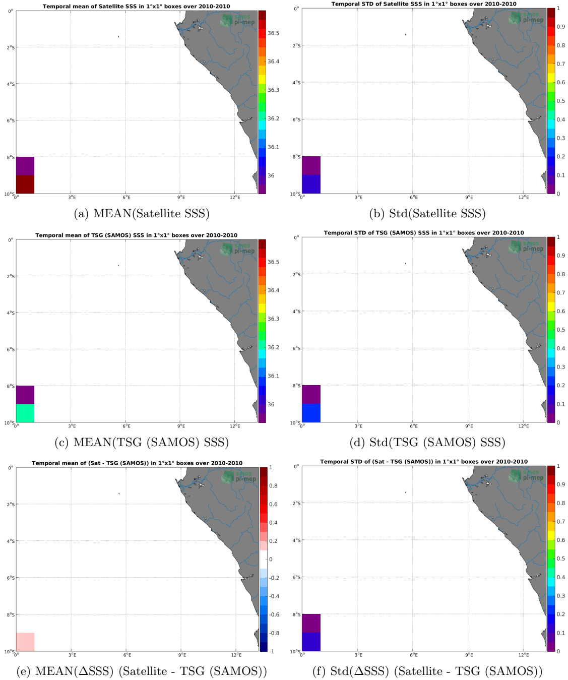
Figure 6: Temporal mean (left) and Std (right) of SSS from SMOS SSS L3 v317 - 10 Days - 25 km (CATDS-CPDC) (top), TSG (SAMOS) (middle), and of \Delta SSS (Satellite - TSG (SAMOS)). Only match-up pairs are used to generate these maps.
