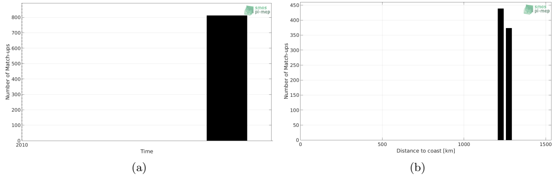
Figure 1: Number of match-ups between TSG (SAMOS) and SMOS SSS L3 v317 - 10 Days - 25 km (CATDS-CPDC) SSS as a function of time (a) and as function of the distance to coast (b) over the Congo river plume Pi-MEP region and for the full satellite product period.
