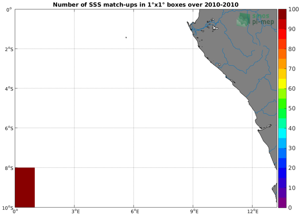
Figure 4: Number of SSS match-ups between TSG (SAMOS) SSS and the SMOS SSS L3 v317 - 10 Days - 25 km (CATDS-CPDC) SSS product for the Congo river plume Pi-MEP region over 1^\circ \times 1^\circ boxes and for the full satellite product period.
