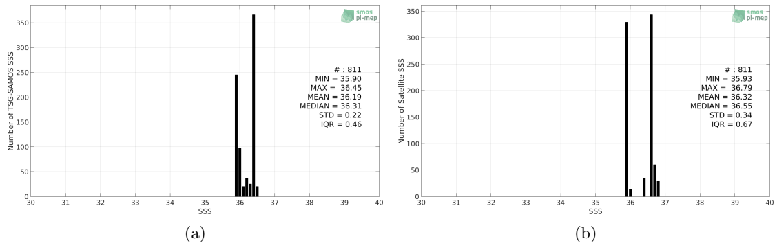
Figure 2: Histograms of SSS from TSG-SAMOS (a) and SMOS-L3-CATDS-CPDC-V317-10DAYS-25KM (b) considering all match-up pairs per bins of 0.1 over the Congo river plume Pi-MEP region and for the full satellite product period.
