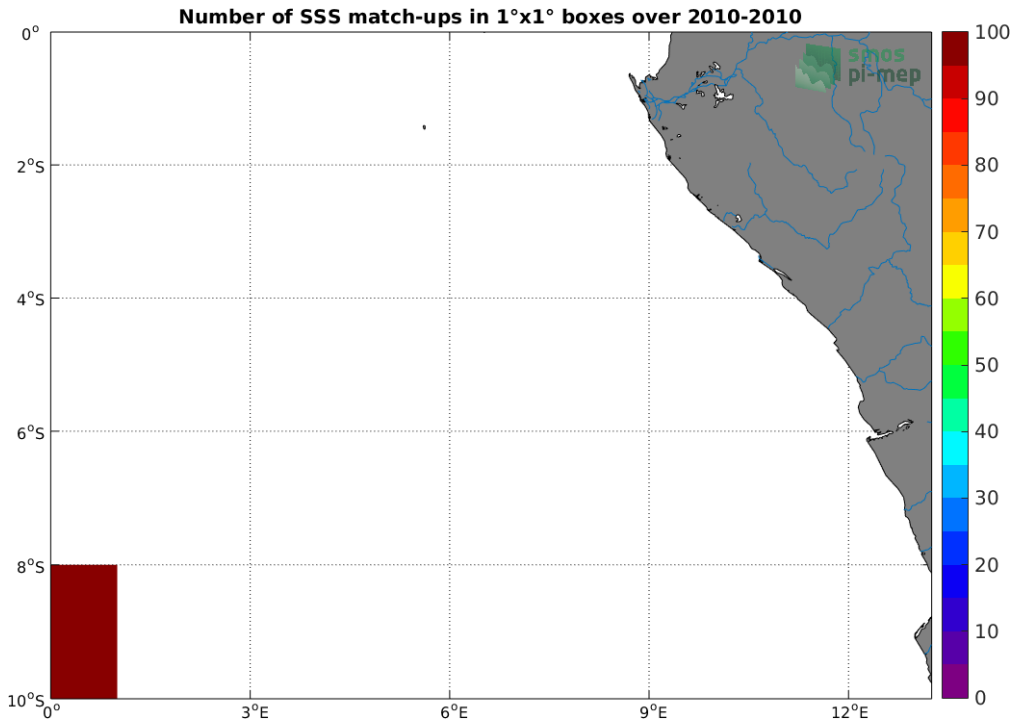
Figure 4: Number of SSS match-ups between TSG-SAMOS SSS and the SMOS-L3-CATDS-CPDC-V317-10DAYS-25KM SSS product for the Congo river plume Pi-MEP region over 1^\circ \times 1^\circ boxes and for the full satellite product period.
