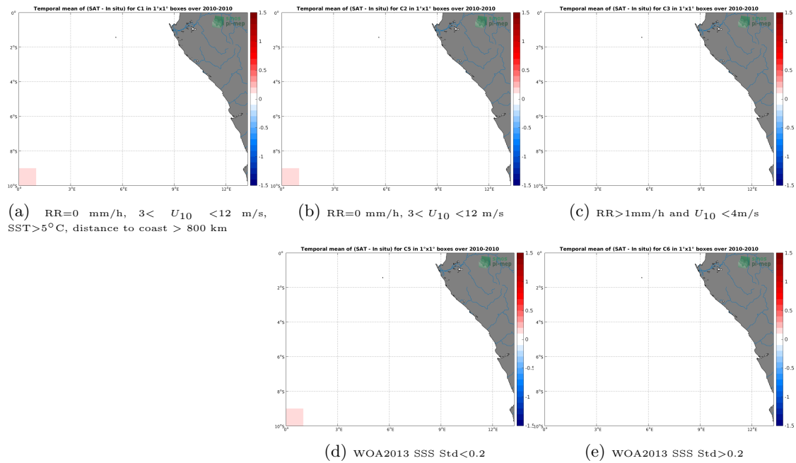
Figure 12: Temporal mean gridded over spatial boxes of size 1^\circ \times 1^\circ of \Delta SSS (SMOS-L3-CATDS-CPDC-V317-10DAYS-25KM - TSG-SAMOS) for 5 different subdatasets corresponding to:RR=0 mm/h, 3 < U_{10} < 12 m/s, SST > 5^\circ\text{C} , distance to coast > 800 km (a), RR=0 mm/h, 3 < U_{10} < 12 m/s (b), RR > 1 mm/h and U_{10} < 4 m/s (c), WOA2013 SSS Std < 0.2 (d), WOA2013 SSS Std > 0.2 (e).
