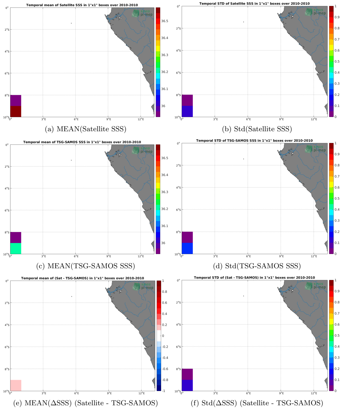
Figure 6: Temporal mean (left) and Std (right) of SSS from SMOS-L3-CATDS-CPDC-V317-10DAYS-25KM (top), TSG-SAMOS (middle), and of \Delta SSS (Satellite - TSG-SAMOS). Only match-up pairs are used to generate these maps.
