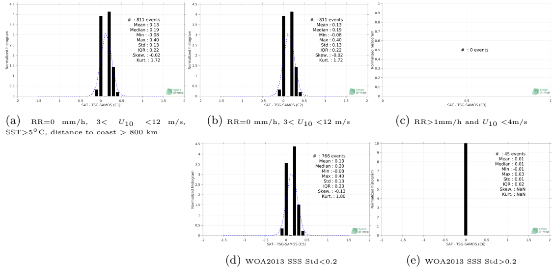
Figure 13: Normalized histogram of \Delta SSS (SMOS-L3-CATDS-CPDC-V317-10DAYS-25KM - TSG-SAMOS) for 5 different subdatasets corresponding to: RR=0 mm/h, 3 < U_{10} < 12 m/s, SST > 5°C, distance to coast > 800 km (a), RR=0 mm/h, 3 < U_{10} < 12 m/s (b), RR > 1mm/h and U_{10} < 4 m/s (c), WOA2013 SSS Std < 0.2 (d), WOA2013 SSS Std > 0.2 (e).
