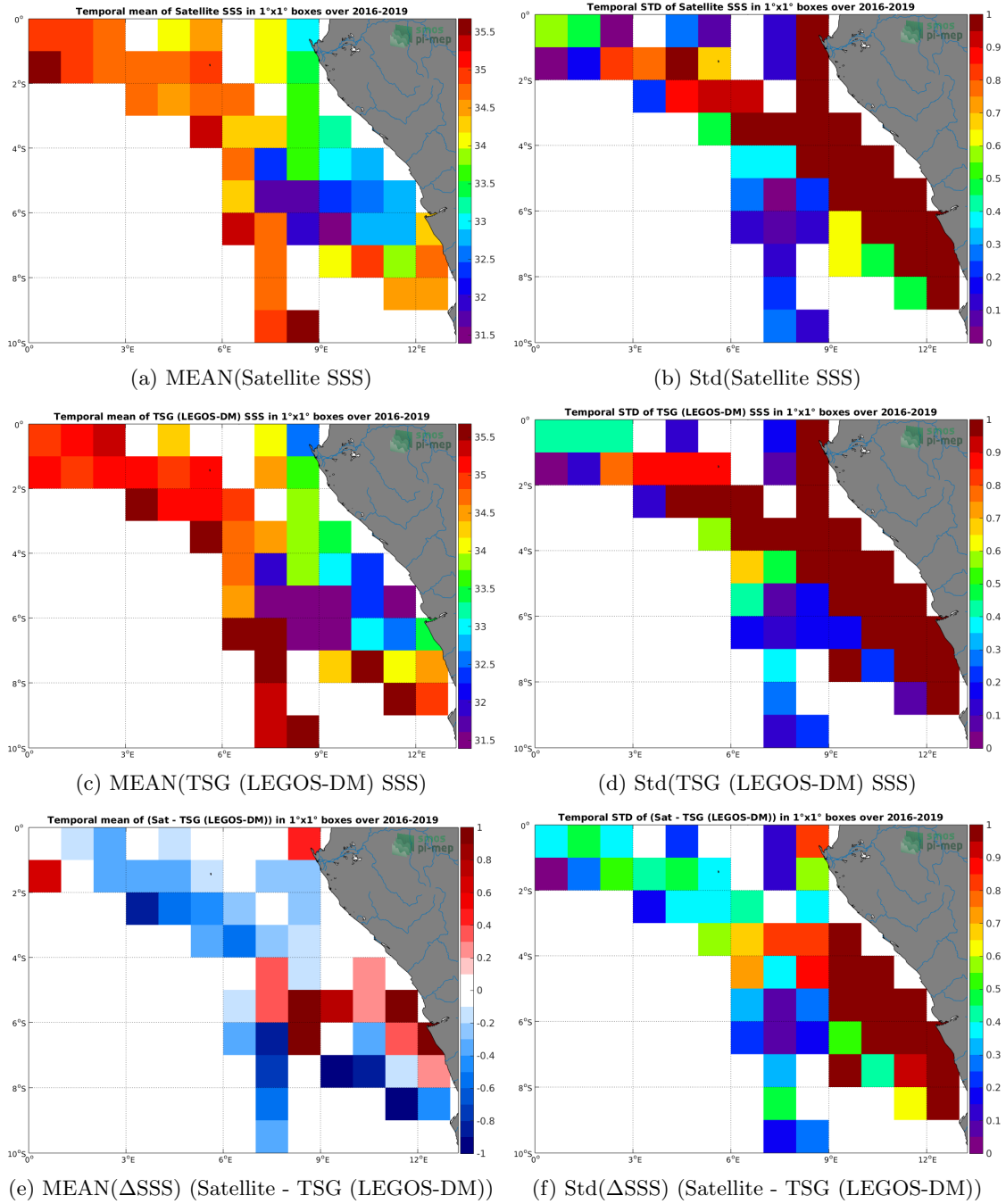
Figure 6: Temporal mean (left) and Std (right) of SSS from SMOS SSS L3 v317 - 10 Days - 25 km (CATDS-CPDC) (top), TSG (LEGOS-DM) (middle), and of \Delta SSS (Satellite - TSG (LEGOS-DM)). Only match-up pairs are used to generate these maps.
