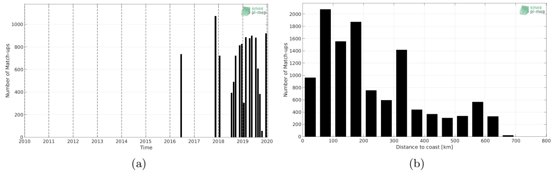
Figure 1: Number of match-ups between TSG (LEGOS-DM) and SMOS SSS L3 v317 - 10 Days - 25 km (CATDS-CPDC) SSS as a function of time (a) and as function of the distance to coast (b) over the Congo river plume Pi-MEP region and for the full satellite product period.
