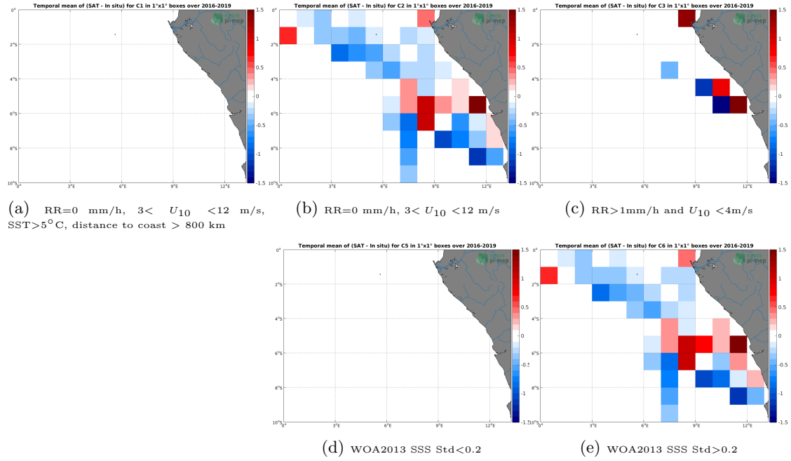
Figure 12: Temporal mean gridded over spatial boxes of size 1^{\circ}\times 1^{\circ} of \Delta\text{SSS} (SMOS SSS L3 v317 - 10 Days - 25 km (CATDS-CPDC) - TSG (LEGOS-DM)) for 5 different subdatasets corresponding to:RR=0 mm/h, 3 < U_{10} < 12 m/s, SST >5^{\circ}\text{C} , distance to coast > 800 km (a), RR=0 mm/h, 3 < U_{10} < 12 m/s (b), RR >1 mm/h and U_{10} < 4 m/s (c), WOA2013 SSS Std <0.2 (d), WOA2013 SSS Std >0.2 (e).
