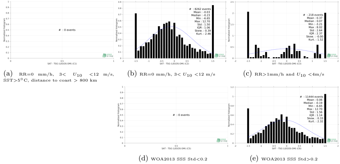
Figure 13: Normalized histogram of \Delta\text{SSS} (SMOS SSS L3 v317 - 10 Days - 25 km (CATDS-CPDC) - TSG (LEGOS-DM)) for 5 different subdatasets corresponding to: RR=0 mm/h, 3 < U_{10} < 12 m/s, SST > 5^\circ\text{C} , distance to coast > 800 km (a), RR=0 mm/h, 3 < U_{10} < 12 m/s (b), RR > 1\text{mm/h} and U_{10} < 4\text{m/s} (c), WOA2013 SSS Std < 0.2 (d), WOA2013 SSS Std > 0.2 (e).
