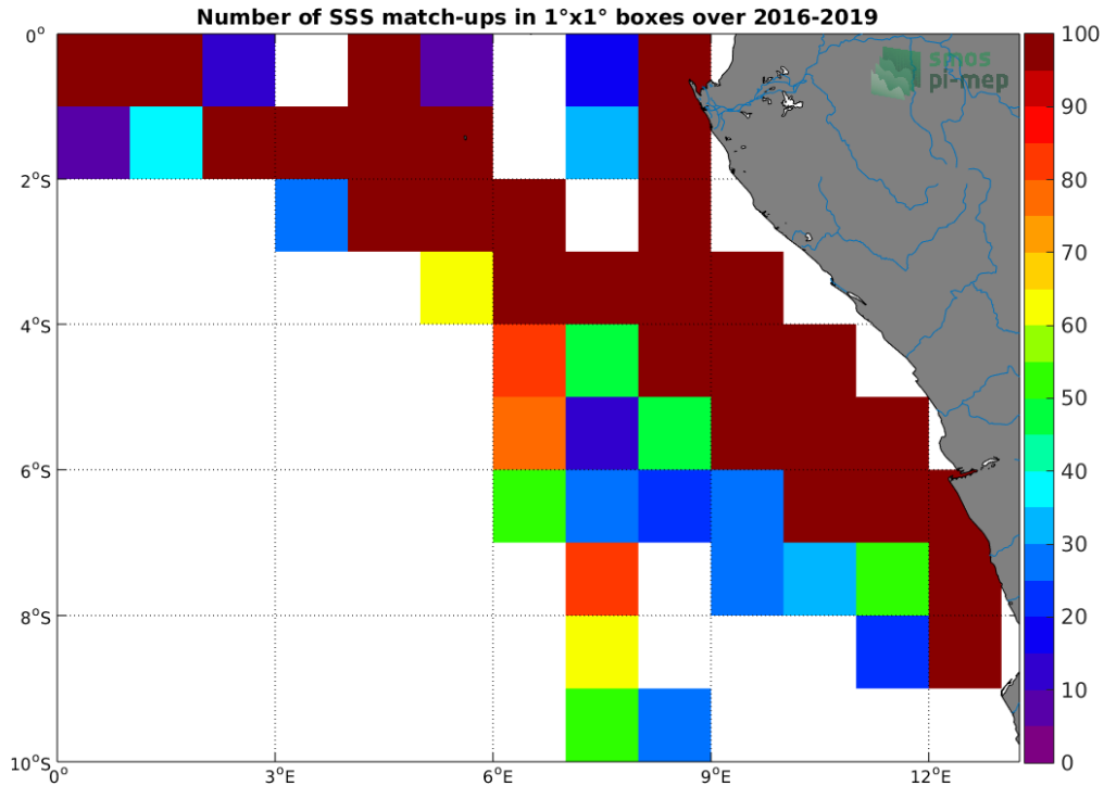
Figure 4: Number of SSS match-ups between TSG (LEGOS-DM) SSS and the SMOS SSS L3 v317 - 10 Days - 25 km (CATDS-CPDC) SSS product for the Congo river plume Pi-MEP region over 1^\circ \times 1^\circ boxes and for the full satellite product period.
