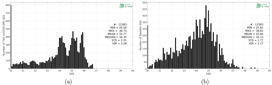
Figure 2: Histograms of SSS from TSG (LEGOS-DM) (a) and SMOS SSS L3 v317 - 10 Days - 25 km (CATDS-CPDC) (b) considering all match-up pairs per bins of 0.1 over the Congo river plume Pi-MEP region and for the full satellite product period.
