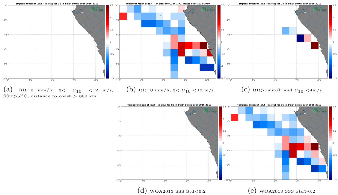
Figure 12: Temporal mean gridded over spatial boxes of size 1^\circ \times 1^\circ of \Delta SSS (SMOS L3 v317 - 10 Days - 25 km (CATDS-CPDC) - TSG-LEGOS-DM) for 5 different subdatasets corresponding to:RR=0 mm/h, 3 < U_{10} < 12 m/s, SST > 5^\circ\text{C} , distance to coast > 800 km (a), RR=0 mm/h, 3 < U_{10} < 12 m/s (b), RR > 1 mm/h and U_{10} < 4 m/s (c), WOA2013 SSS Std < 0.2 (d), WOA2013 SSS Std > 0.2 (e).
