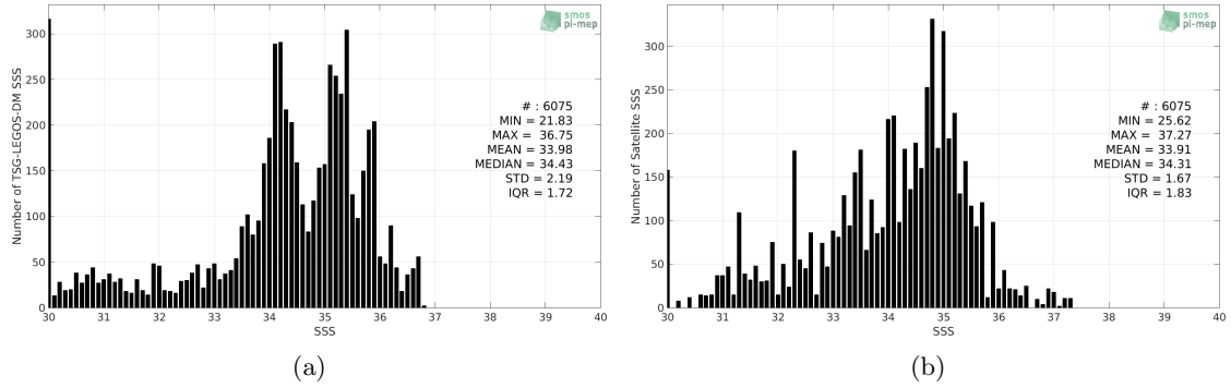
Figure 2: Histograms of SSS from TSG-LEGOS-DM (a) and SMOS L3 v317 - 10 Days - 25 km (CATDS-CPDC) (b) considering all match-up pairs per bins of 0.1 over the Congo river plume Pi-MEP region and for the full satellite product period.
