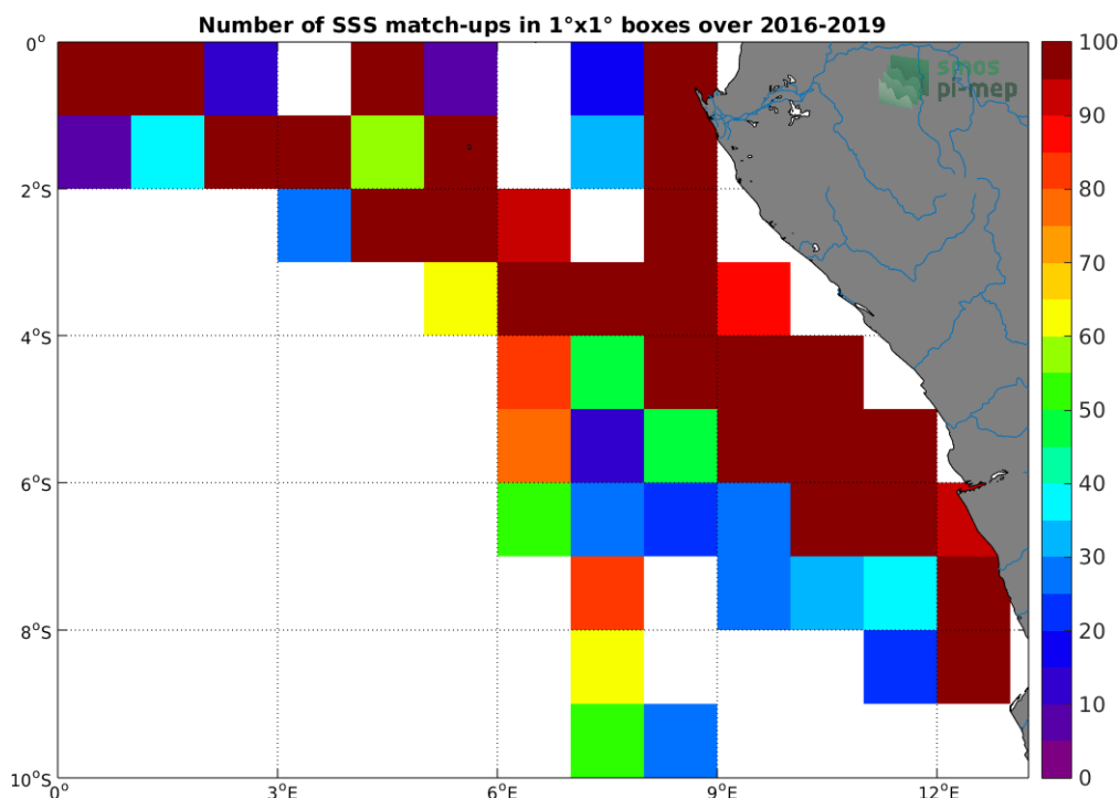
Figure 4: Number of SSS match-ups between TSG-LEGOS-DM SSS and the SMOS L3 v317 - 10 Days - 25 km (CATDS-CPDC) SSS product for the Congo river plume Pi-MEP region over 1°x1° boxes and for the full satellite product period.
