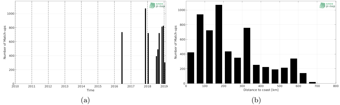
Figure 1: Number of match-ups between TSG-LEGOS-DM and SMOS L3 v317 - 10 Days - 25 km (CATDS-CPDC) SSS as a function of time (a) and as function of the distance to coast (b) over the Congo river plume Pi-MEP region and for the full satellite product period.
