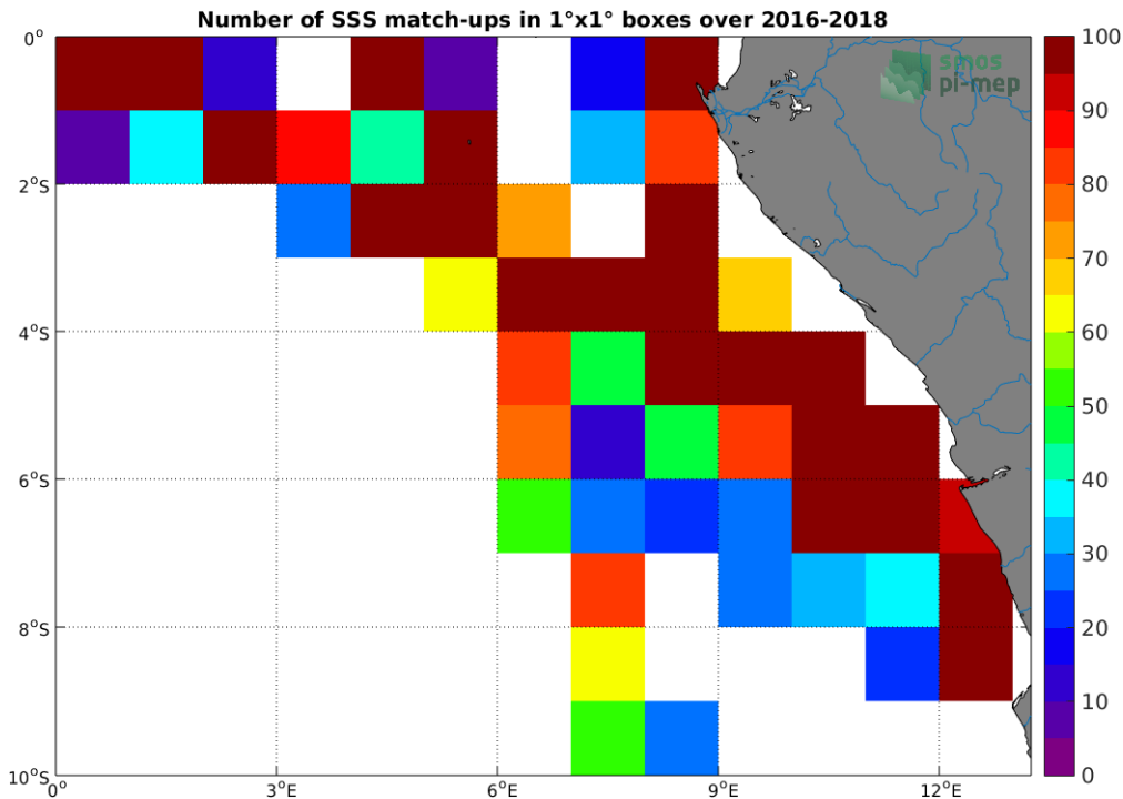
Figure 4: Number of SSS match-ups between TSG-LEGOS-DM SSS and the SMOS-L3-CATDS-CPDC-V317-10DAYS-25KM SSS product for the Congo river plume Pi-MEP region over 1°x1° boxes and for the full satellite product period.
